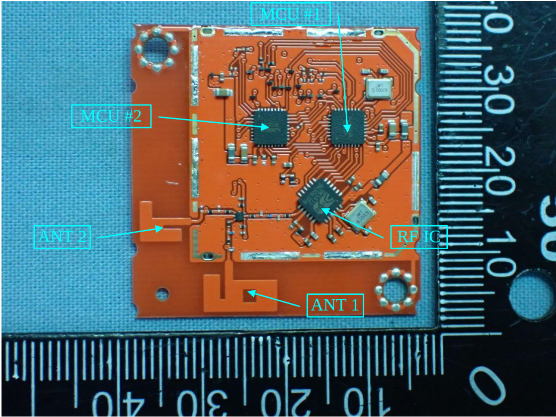
Figure 4 Antenna View
