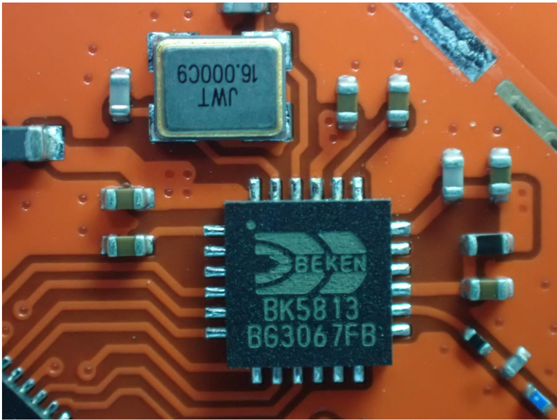
Figure 7 RF IC: BK5813 / Oscillator View
