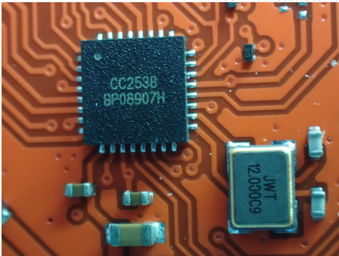
Figure 5 MCU#1: CC2538 / Oscillator View
