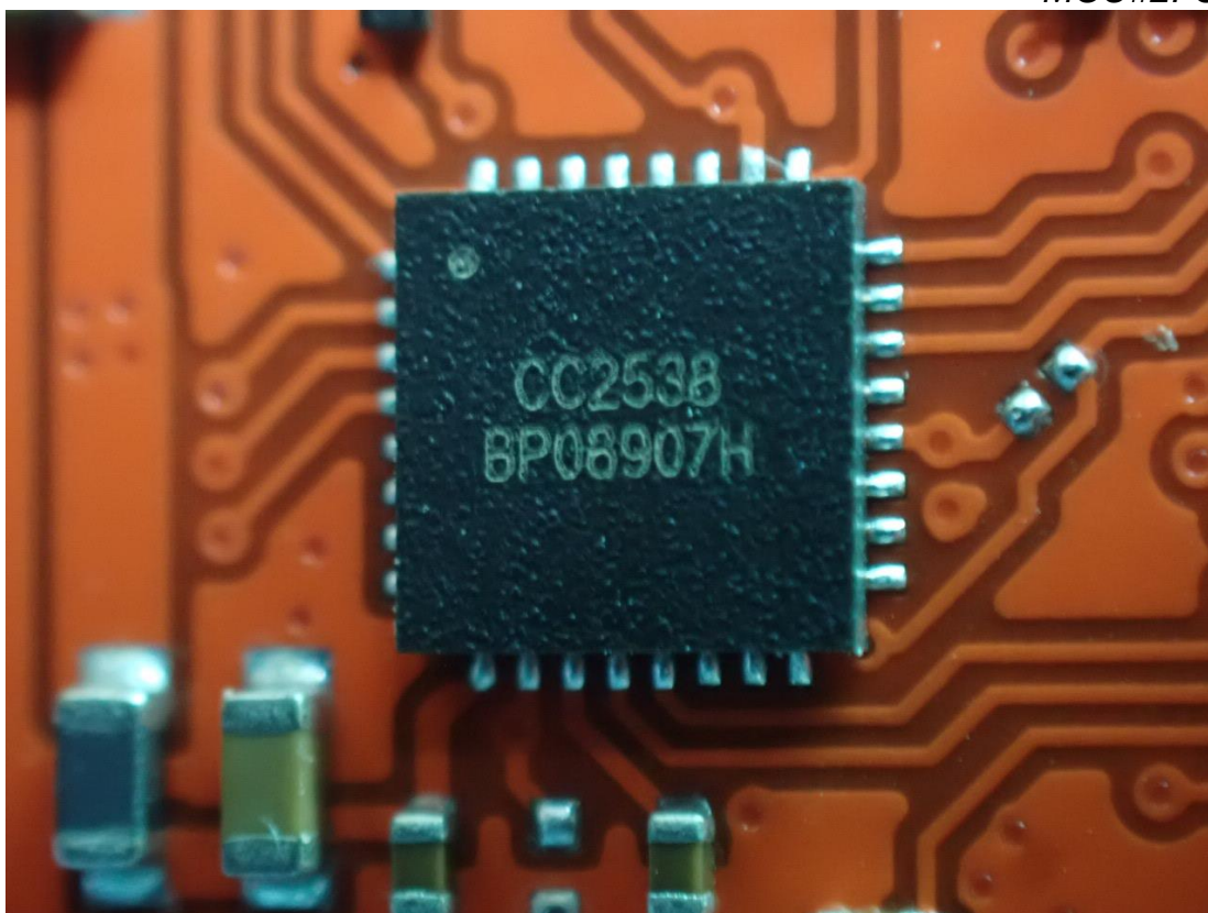
Figure 6 MCU#2: CC2538
