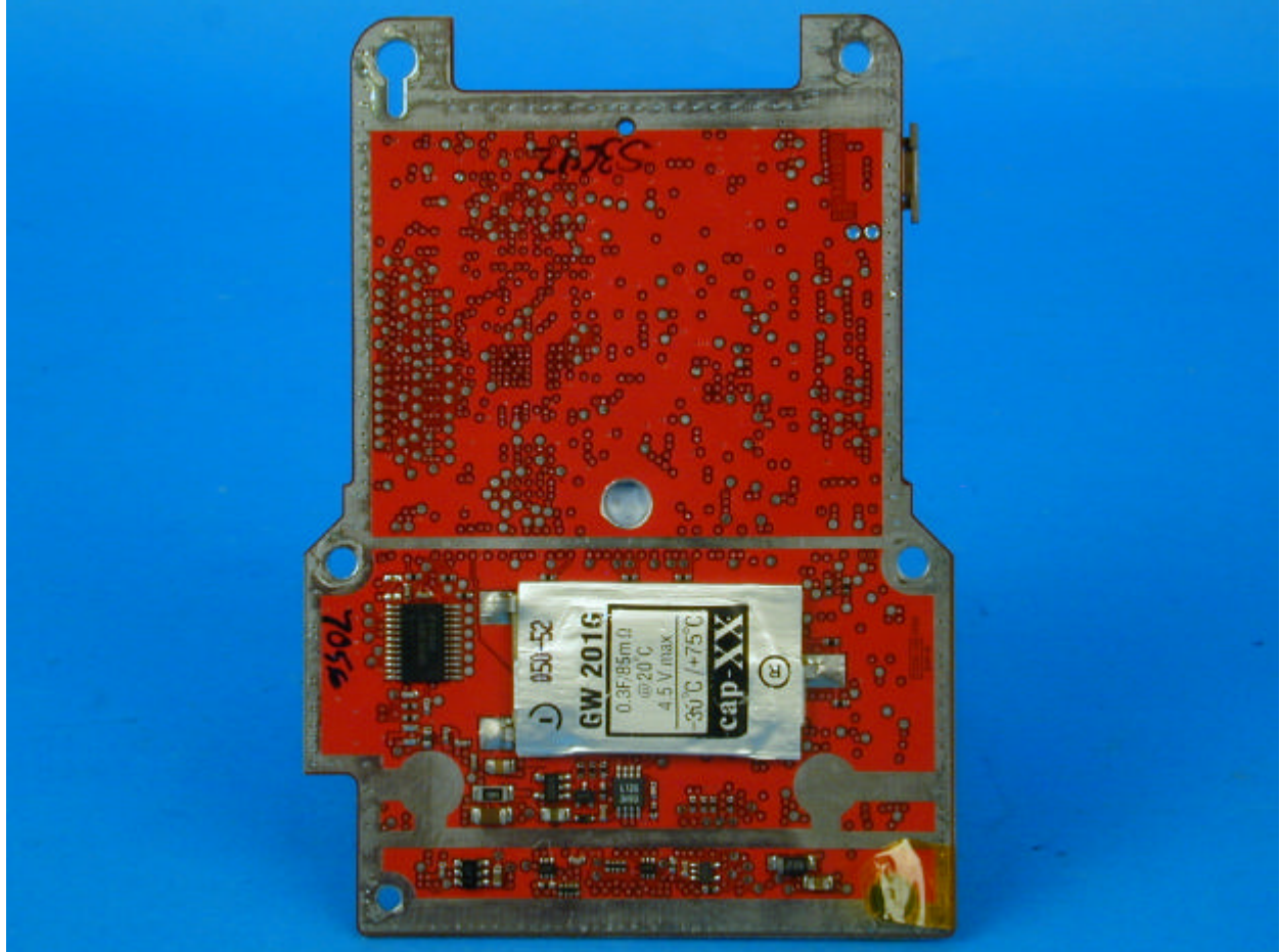
Internal View 5
