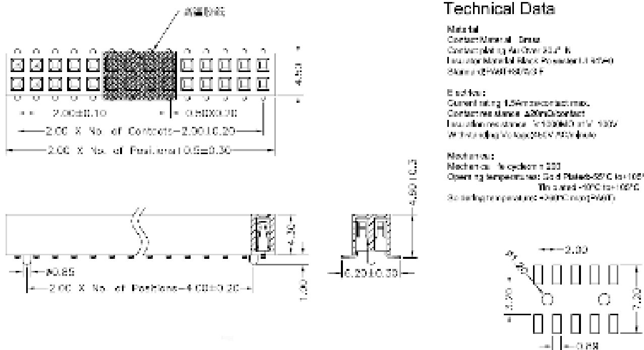
Figure 2-3 Female Connector Dimensions
