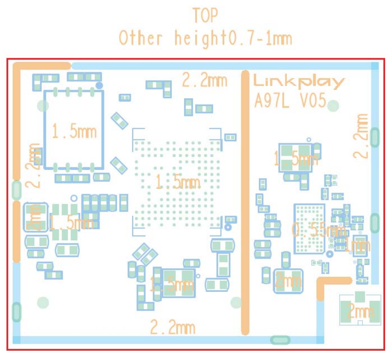
Figure 2-7 TOP Components Height
