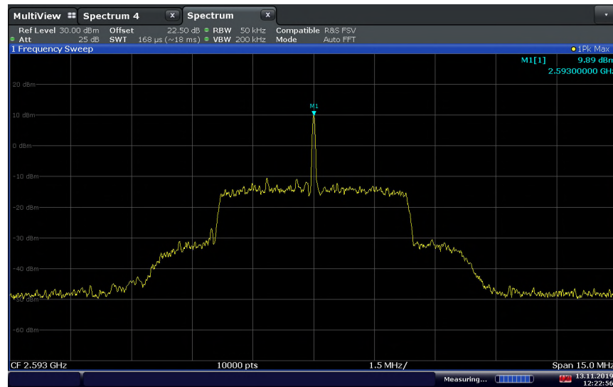
LTE Band 41 Downlink 120VAC @ 20°C
