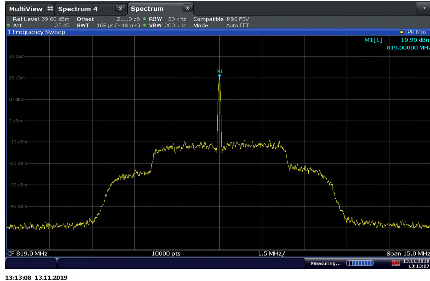
LTE Band 26 (814 – 849 MHz) Uplink 120VAC @ 20°C
