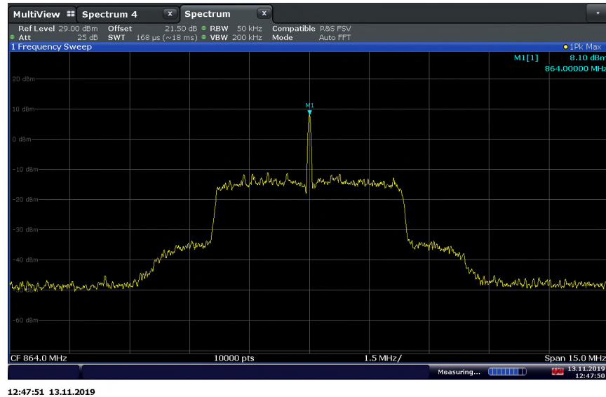
LTE Band 26 (859 – 869 MHz) Downlink 120VAC @ 20°C
