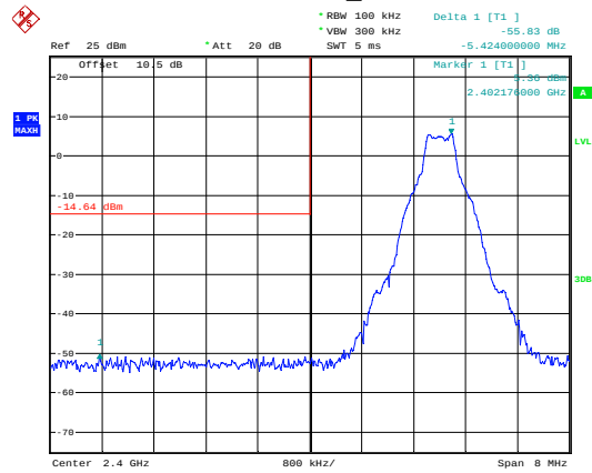
GFSK_Low
