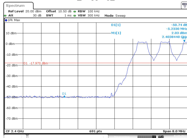
GFSK_Hopping_Lower
