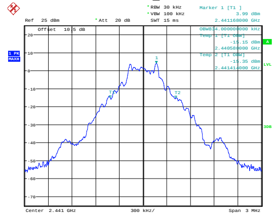
GFSK_Middle
