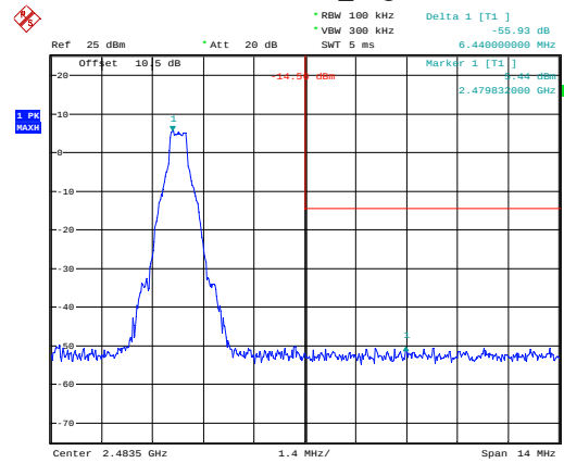
GFSK_High
