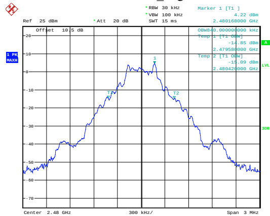
GFSK_High
