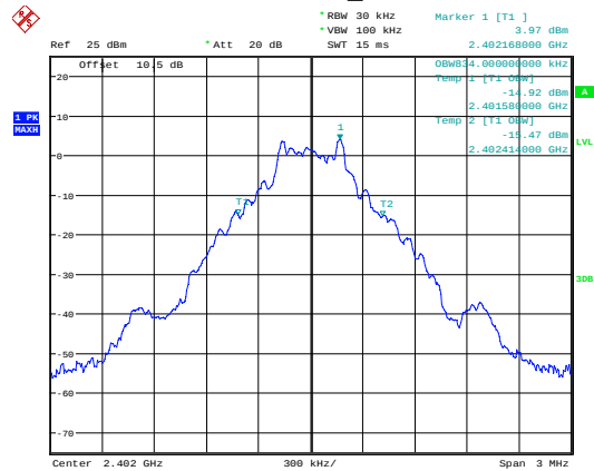
GFSK_Low
