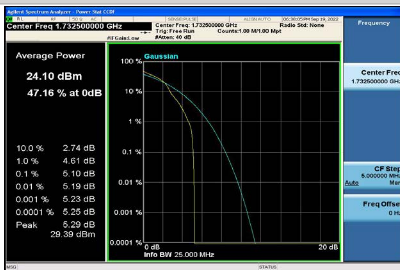
Band4-3MHz-16QAM-20175-1RB#0
