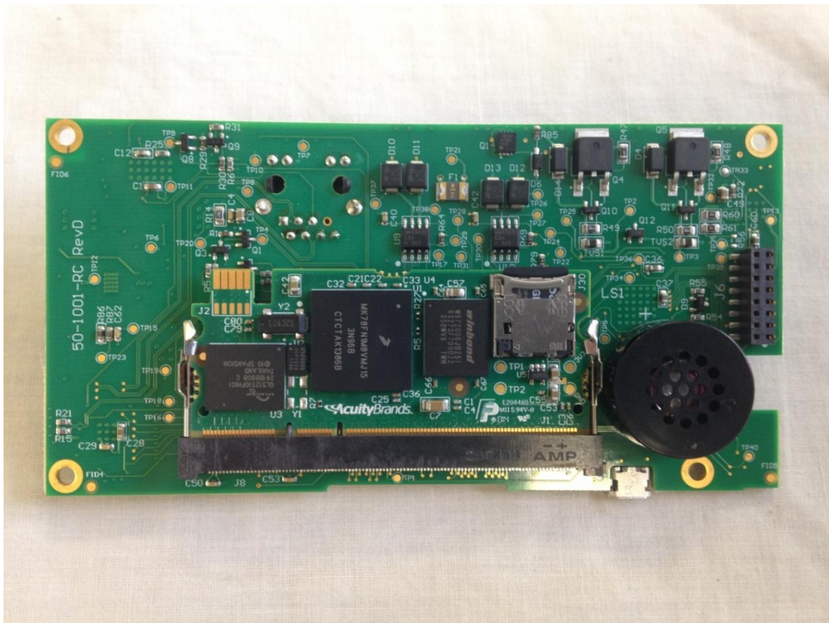
Photo 9- Back Side of Circuit Board #1 with Circuit Board #2 Attached
