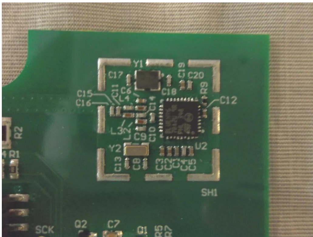
Photo 17- Radio on Circuit Board #3
