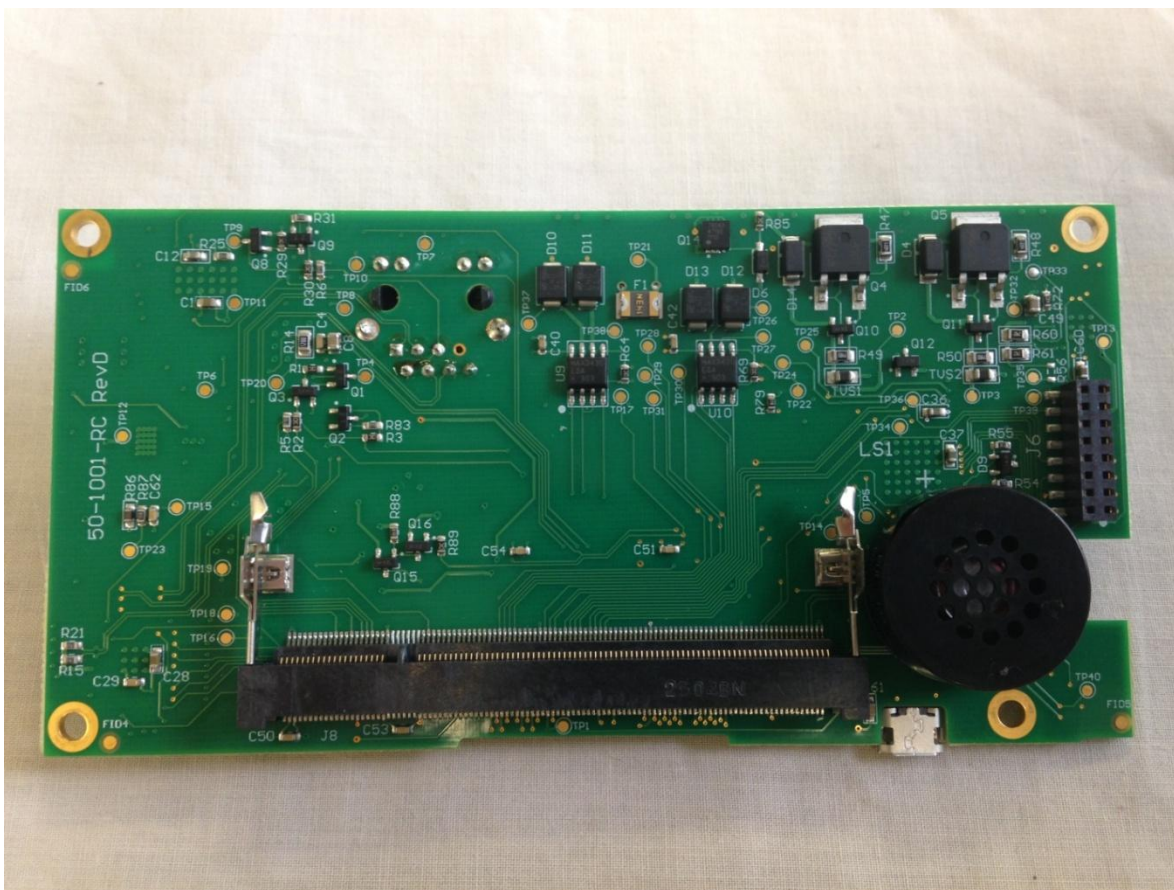
Photo 8- Back Side of Circuit Board #1 with Circuit Board #2 Removed
