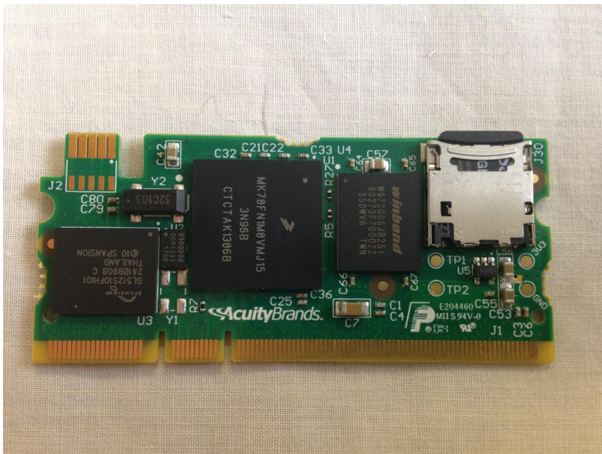
Photo 9- Front Side of Circuit Board #2
