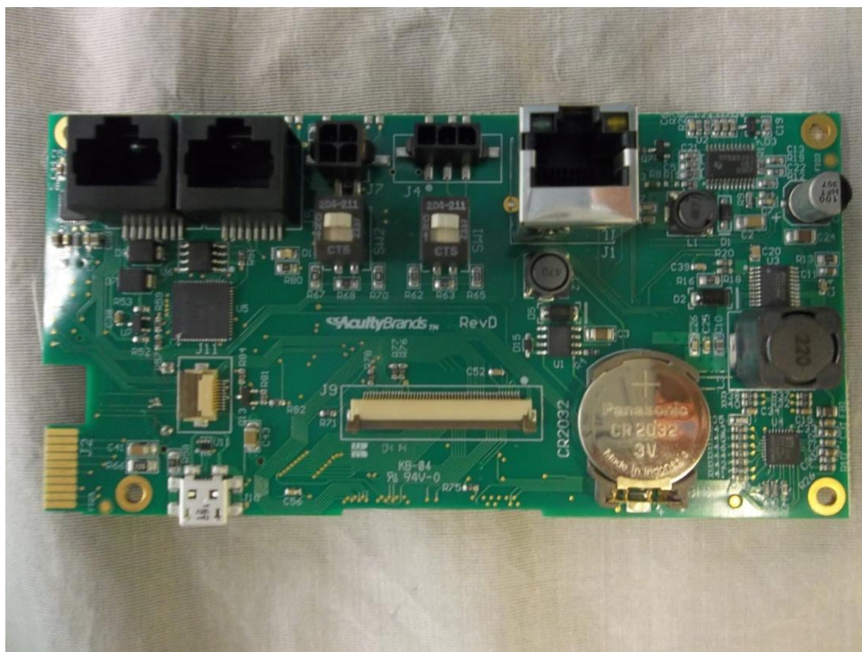
Photo 6- Front Side of Circuit Board #1
