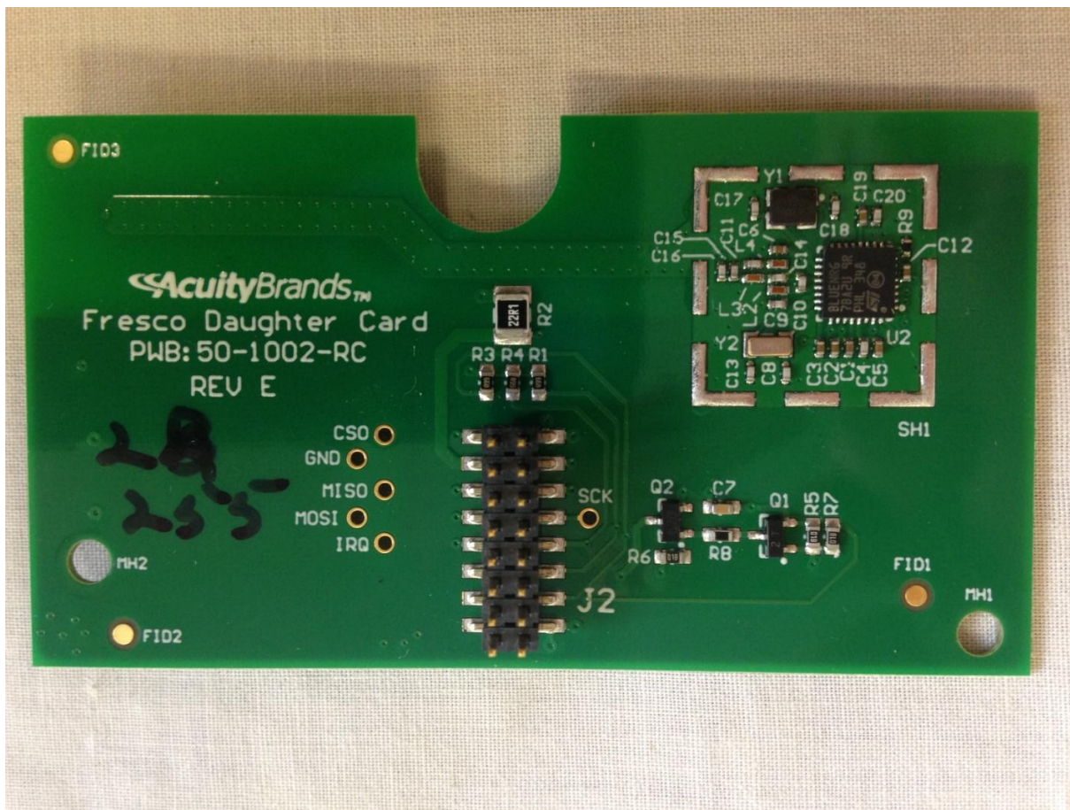
Photo 16- Top of Circuit Board #3, with Radio
