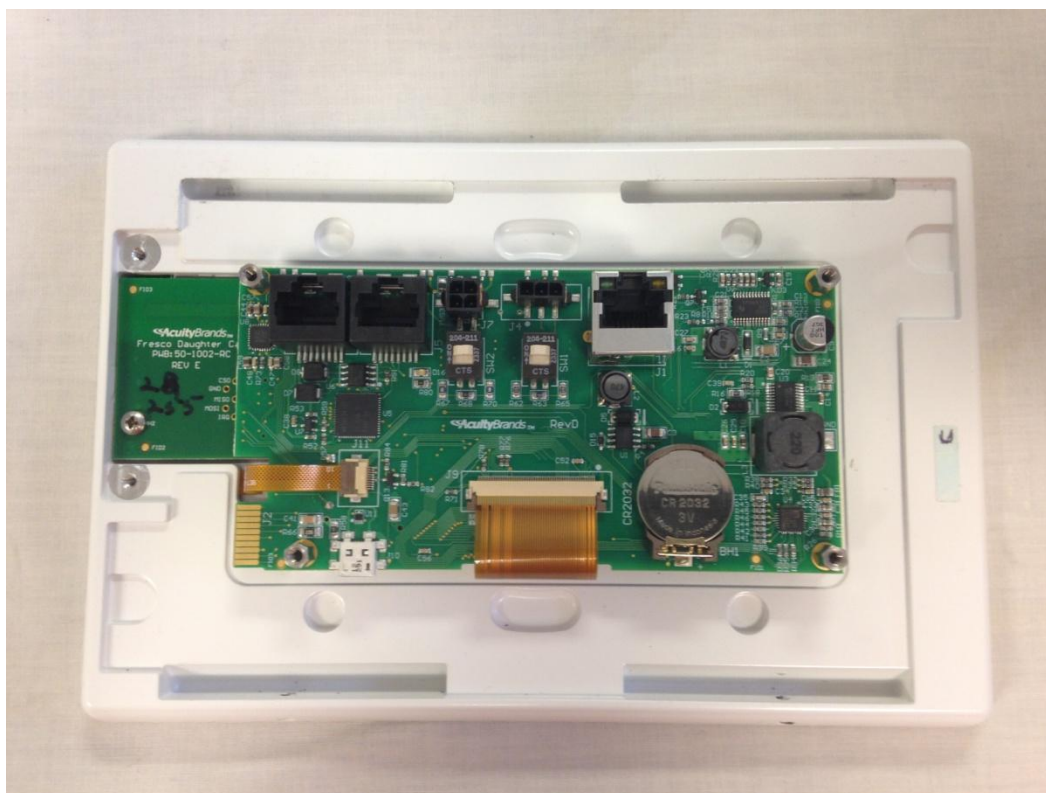
Photo 1- Back of EUT with Back Cover Removed
