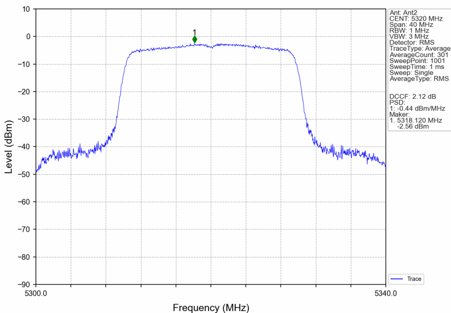
802.11ax(HEW20)_HCH_5320MHz_SU_/_MIMO_NTNV
