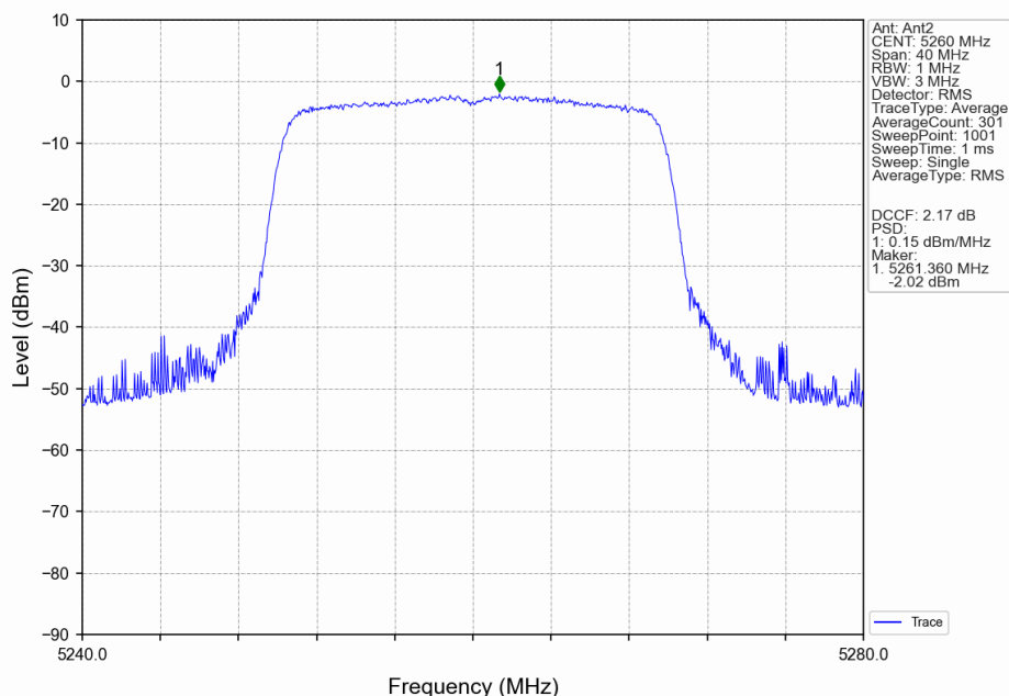
802.11ax(HEW20)_LCH_5260MHz_SU_ / _MIMO_NTNV
