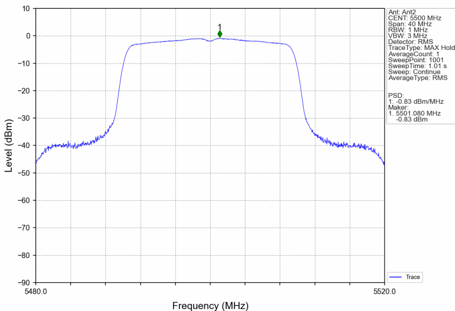
802.11ax(HEW20)_LCH_5500MHz_SU_ / _Ant2_NTNV
