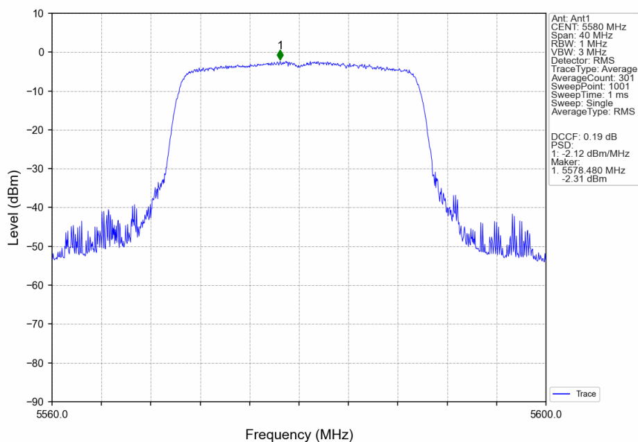
802.11ax(HEW20)_MCH_5580MHz_SU_/_Ant1_NTNV
