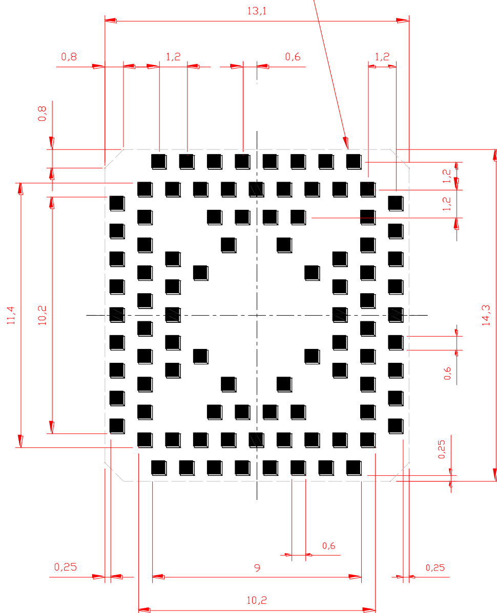
Package outline
