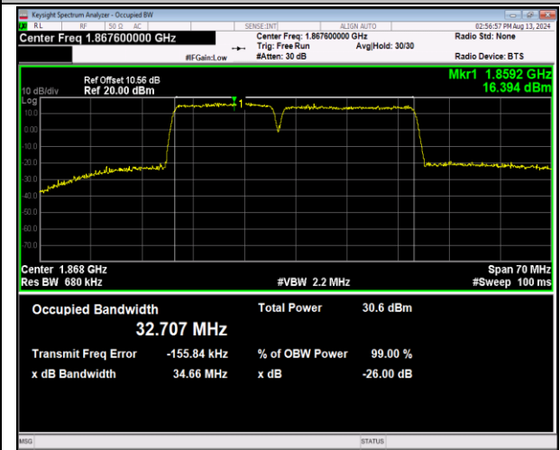
2-2-15MHz-20MHz-QPSK-QPSK-18678-18849-75RB#0-100 100RB#0-PASS
