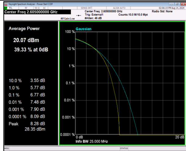
41-41-20MHz-20MHz-QPSK-QPSK-40641-40839-100RB#0-100RB#0-PASS
