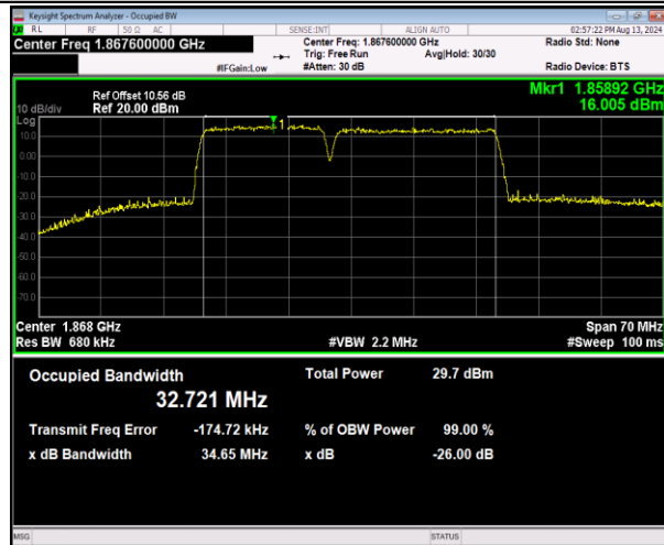
2-2-15MHz-20MHz-16QAM-16QAM-18678-18849-75RB#0-100 0-100RB#0-PASS
