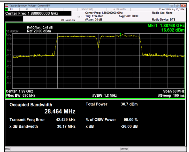
2-2-15MHz-15MHz-QPSK-QPSK-18825-18975-75RB#0-7 75RB#0-PASS
