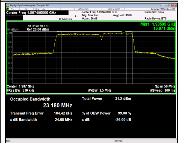
2-2-15MHz-10MHz-QPSK-QPSK-19027-19147-75RB#0-50RB#0-PASS
