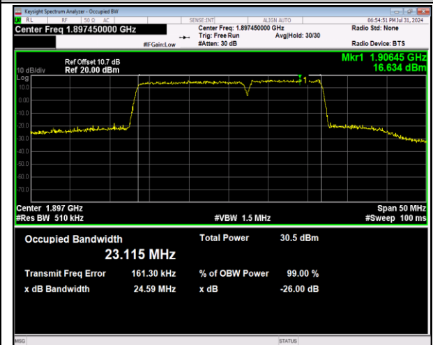
2-2-15MHz-10MHz-64QAM-64QAM-19027-19147-75RB#0-50RB#0-PASS
