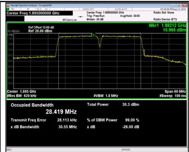
2-2-15MHz-15MHz-16QAM-16QAM-18975-19125-75RB#0-7 #0-75RB#0-PASS
