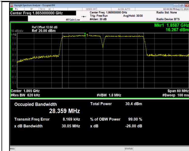
2-2-15MHz-15MHz-QPSK-QPSK-18675-18825-75RB#0-7 5RB#0-PASS
