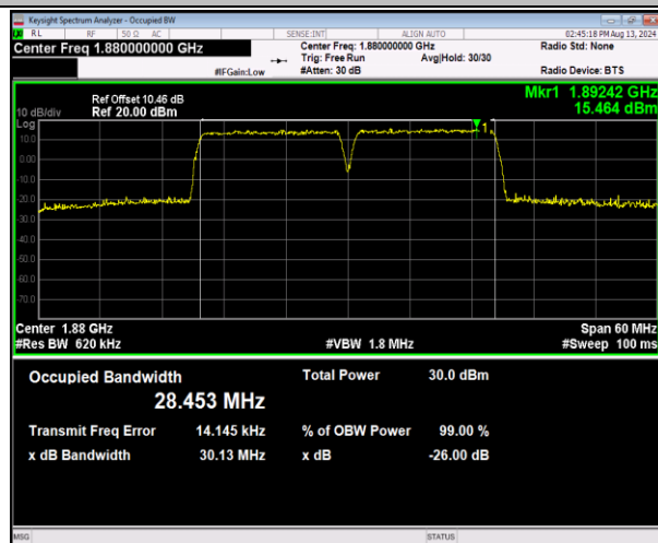
2-2-15MHz-15MHz-16QAM-16QAM-18825-18975-75RB#0-7 0-75RB#0-PASS
