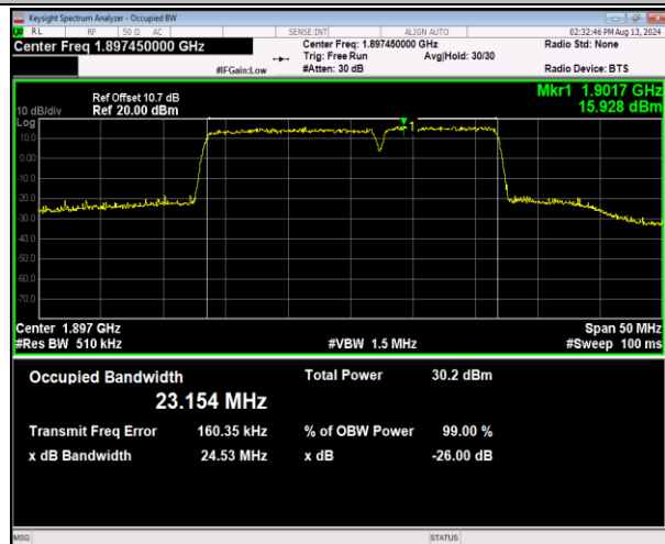
2-2-15MHz-10MHz-16QAM-16QAM-19027-19147-75RB#0-50RB#0-PASS
