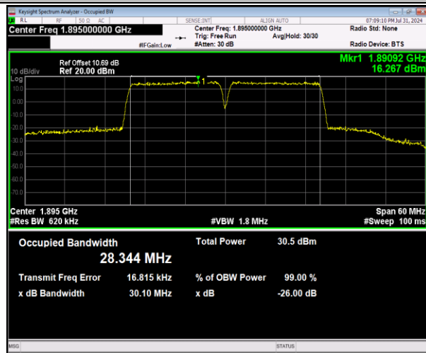
2-2-15MHz-15MHz-64QAM-64QAM-18975-19125-75RB#0-7 0-75RB#0-PASS
