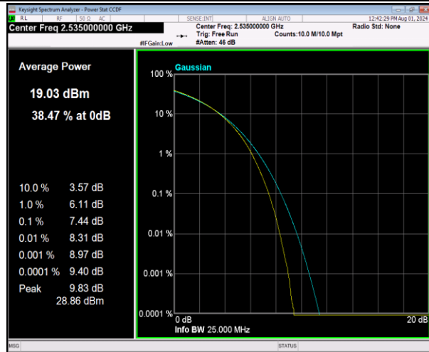
7-7-20MHz-20MHz-64QAM-64QAM-21001-21199-100RB#0-100RB#0-PASS
