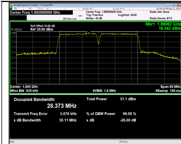
2-2-15MHz-15MHz-QPSK-QPSK-18975-19125-75RB#0-7 5RB#0-PASS
