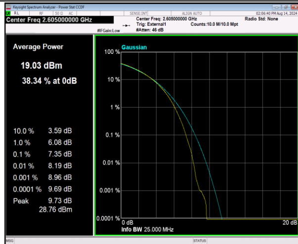
41-41-20MHz-20MHz-16QAM-16QAM-40641-40839-100RB#0-100RB#0-PASS
