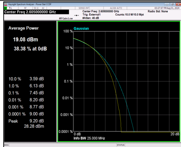
41-41-20MHz-20MHz-64QAM-64QAM-40641-40839-100RB#0-100RB#0-PASS
