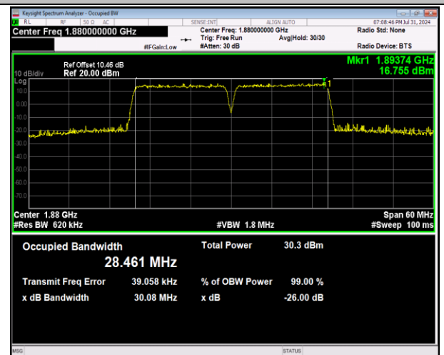
2-2-15MHz-15MHz-64QAM-64QAM-18825-18975-75RB#0-7 #0-75RB#0-PASS
