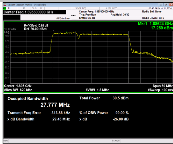
2-2-10MHz-20MHz-64QAM-64QAM-18956-19100-50RB#0-100RB#0-PASS
