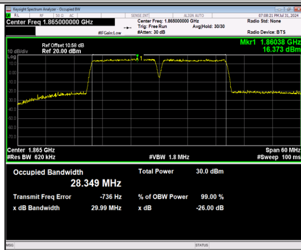
2-2-15MHz-15MHz-64QAM-64QAM-18675-18825-75RB#0-7 0-75RB#0-PASS
