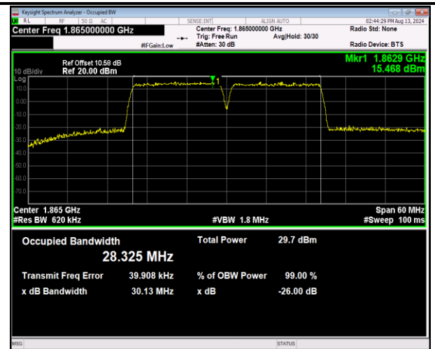
2-2-15MHz-15MHz-16QAM-16QAM-18675-18825-75RB#0-7 #0-75RB#0-PASS
