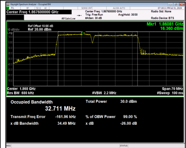
2-2-15MHz-20MHz-64QAM-64QAM-18678-18849-75RB#0-100 #0-100RB#0-PASS
