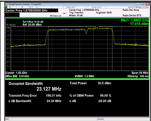
2-2-15MHz-10MHz-16QAM-16QAM-18851-18971-75RB#0-50RB#0-PASS
