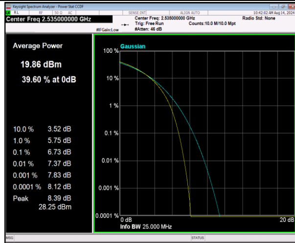
7-7-20MHz-20MHz-QPSK-QPSK-21001-21199-100RB#0-100RB#0-PASS
