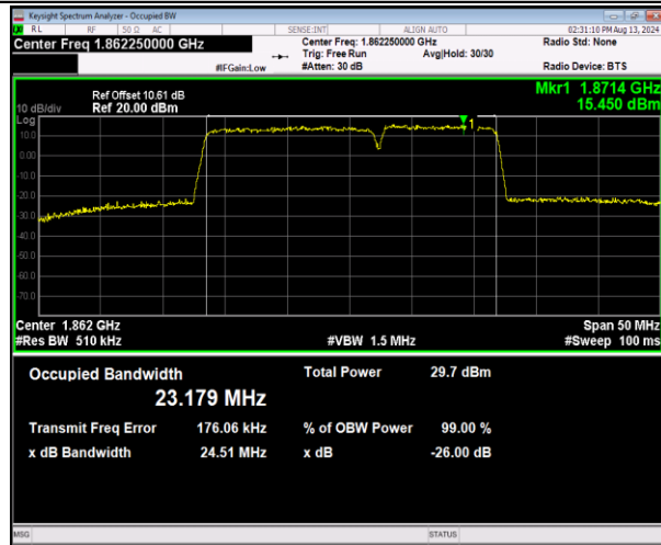
2-2-15MHz-10MHz-16QAM-16QAM-18675-18795-75RB#0-50RB#0-PASS
