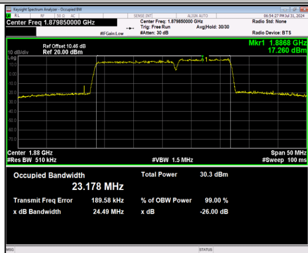
2-2-15MHz-10MHz-64QAM-64QAM-18851-18971-75RB#0-50RB#0-PASS
