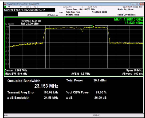
2-2-15MHz-10MHz-QPSK-QPSK-18675-18795-75RB#0-50RB#0-PASS
