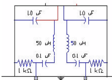
Figure 5. LISN Schematic Diagram
