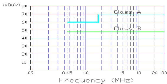
Fig. 11. Line-Conducted Limits
