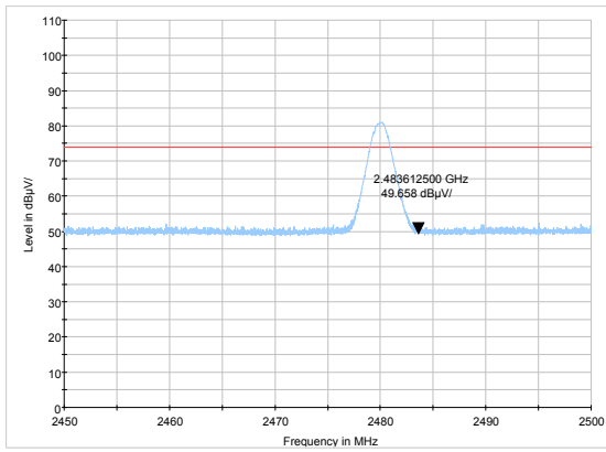
3DH5-Channel 78: Peak
