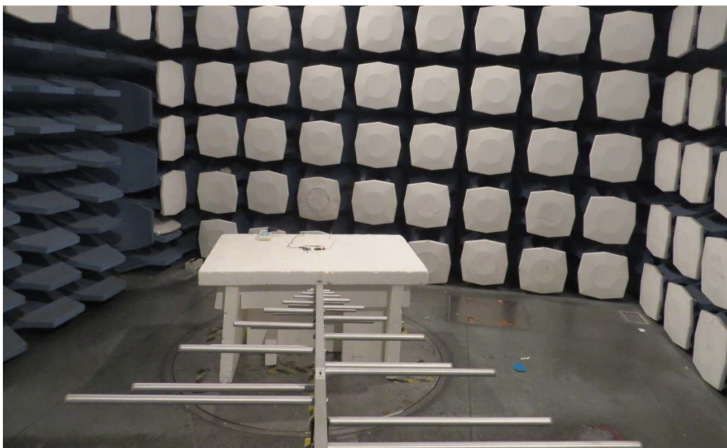
Below 1GHz
