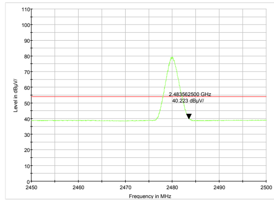
3DH5-Channel 78: Average
