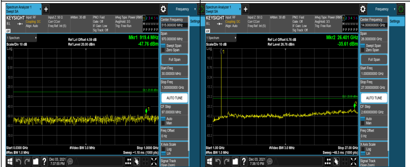
Band7-5MHz-QPSK-21425-1RB#0-Range1:30~100 OOMHz
