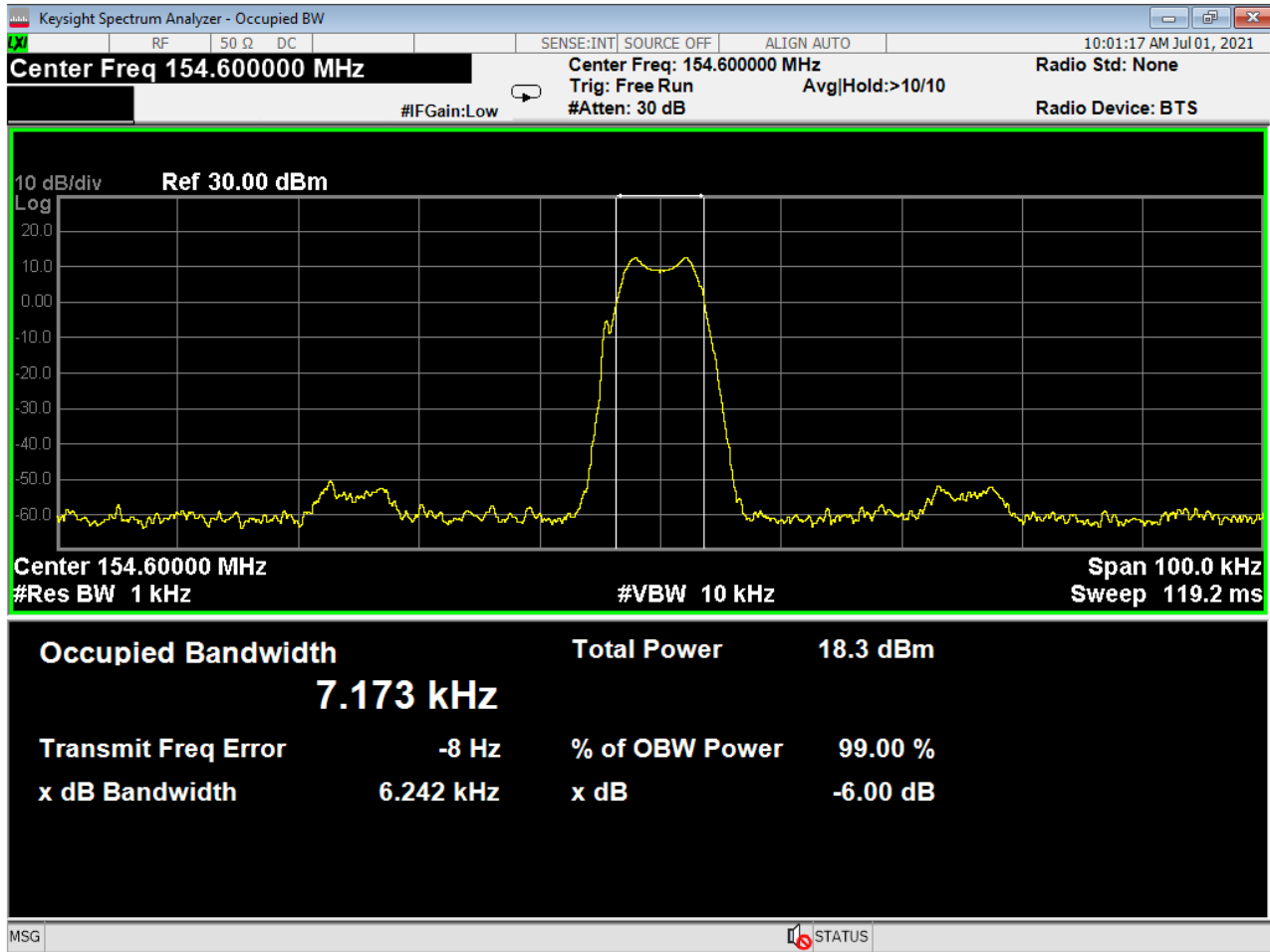
Figure 13 - Bandwidth, 154.600 MHz
