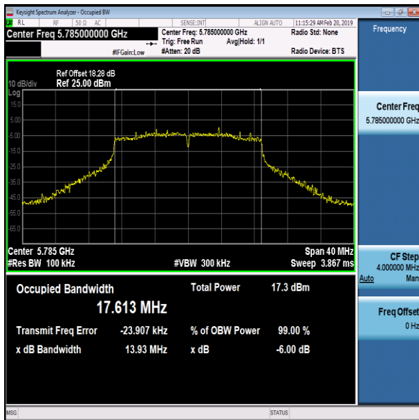
11N20SISO-Ant1-5785
