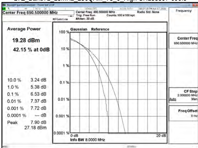
LTE Band71 15MHz 256QAM 75 0 High CH133397-690.5
