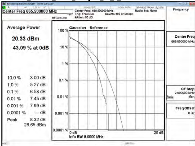
LTE Band71 5MHz 256QAM 25 0 Low CH133147-665.5
