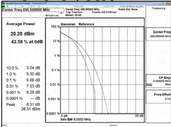
LTE Band71 5MHz 256QAM 25 0 High CH133447-695.5
