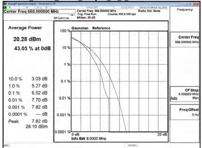
LTE Band71 10MHz 256QAM 50 0 Low CH133172-668
