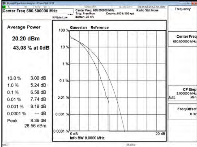
LTE Band71 5MHz 256QAM 25 0 Mid CH133297-680.5
