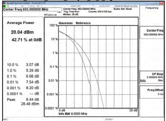
LTE Band71 10MHz 256QAM 50 0 High CH133422-693
