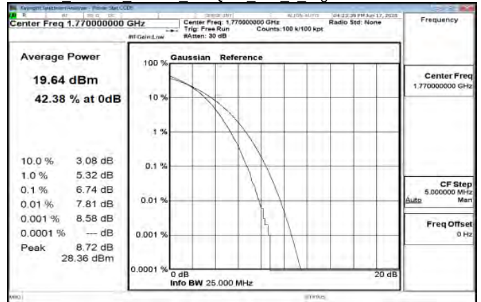
LTE Band66 20MHz 256QAM 100 0 HighCH132572-1770
