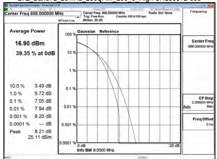
LTE Band71 20MHz 256QAM 100 0 High CH133372-688
