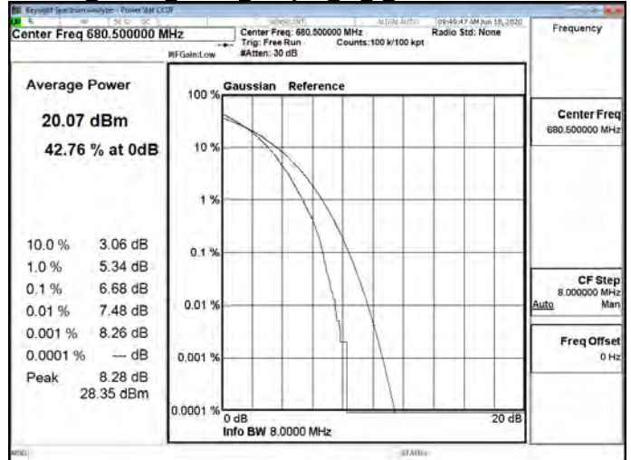
LTE Band71 10MHz 256QAM 50 0 Mid CH133297-680.5
