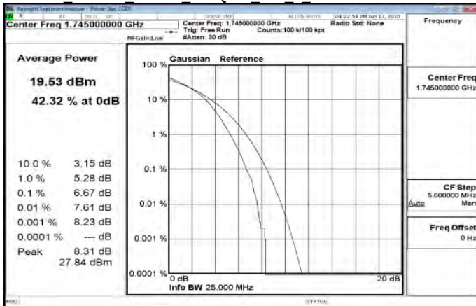
LTE Band66 20MHz 256QAM 100 0 MidCH132322-1745
