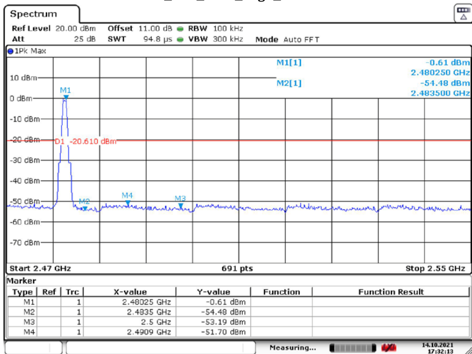
BLE_1M_Ant1_High_2480MHz
