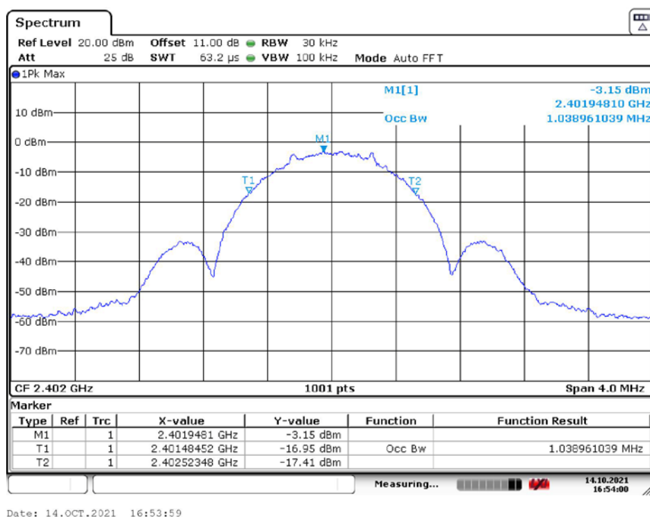
99% Bandwidth, BLE_1M Low Channel
