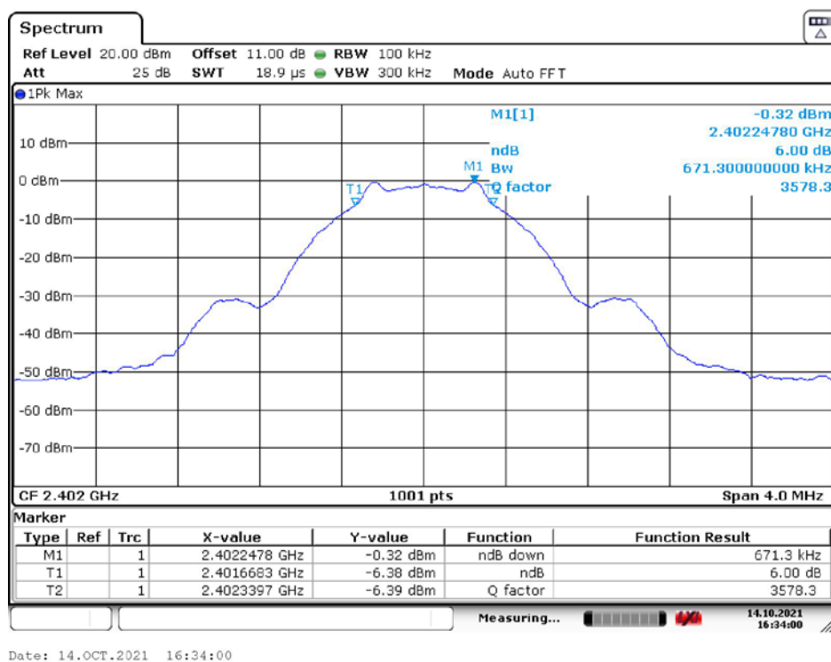
6dB Bandwidth, BLE_1M Low Channel
