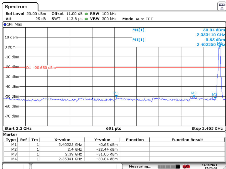
BLE_1M_Ant1_Low_2402MHz
