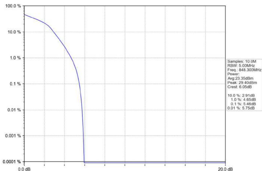
Band26b_1.4MHz_16QAM_HCH_848.3MHz_RB_6_0_NTNV
