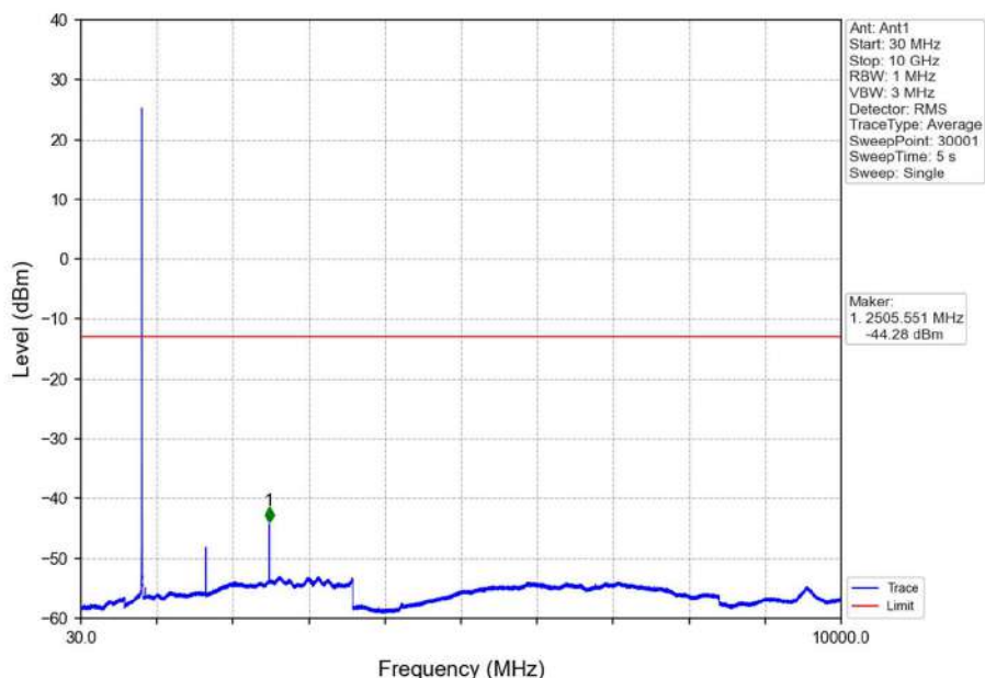
Band26b_3MHz_QPSK_MCH_836.5MHz_RB_1_0_NTNV
