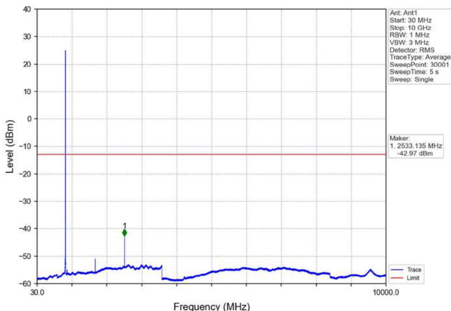
Band26b_5MHz_QPSK_HCH_846.5MHz_RB_1_0_NTNV
