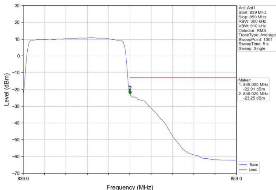
Band26b_10MHz_QPSK_HCH_844MHz_RB_50_0_NTNV
