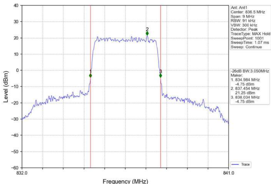
Band26b_3MHz_QPSK_MCH_836.5MHz_RB_15_0_NTNV
