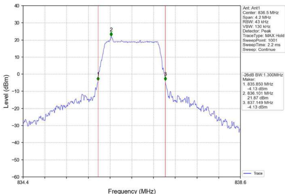
Band26b_1.4MHz_16QAM_MCH_836.5MHz_RB_6_0_NTNV
