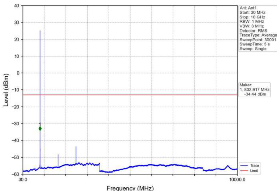
Band26b_1.4MHz_QPSK_MCH_836.5MHz_RB_1_0_NTNV
