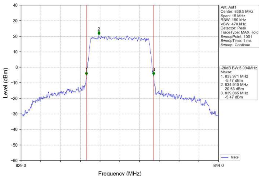
Band26b_5MHz_QPSK_MCH_836.5MHz_RB_25_0_NTNV
