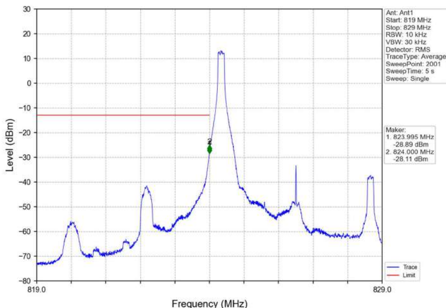
Band26b_5MHz_16QAM_LCH_826.5MHz_RB_1_0_NTNV
