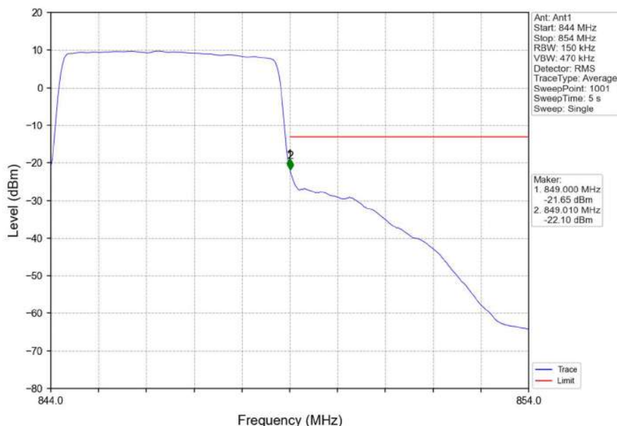
Band26b_5MHz_16QAM_HCH_846.5MHz_RB_25_0_NTNV
