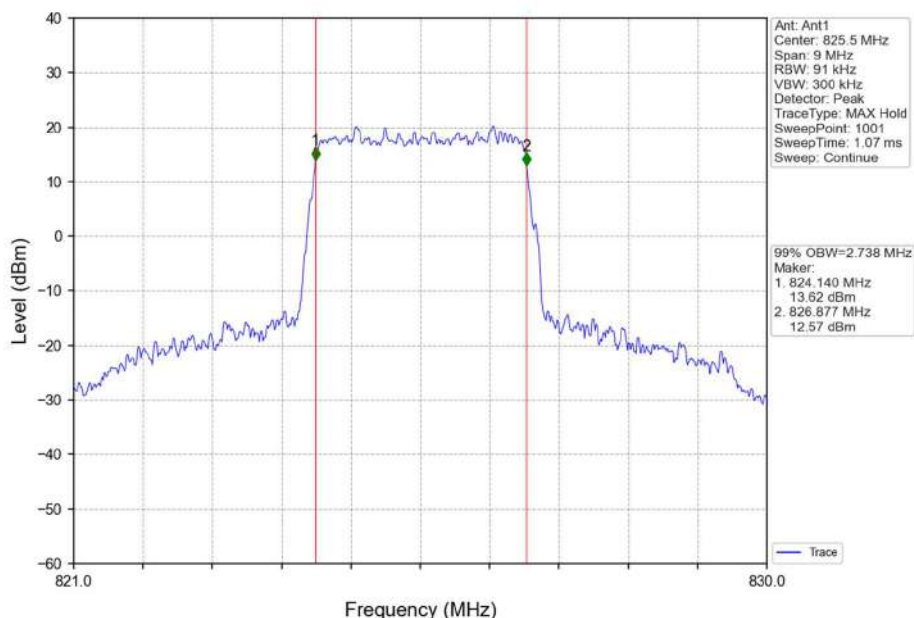
Band26b_3MHz_16QAM_LCH_825.5MHz_RB_15_0_NTNV
