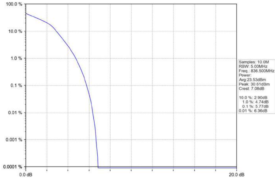
Band26b_3MHz_16QAM_MCH_836.5MHz_RB_15_0_NTNV
