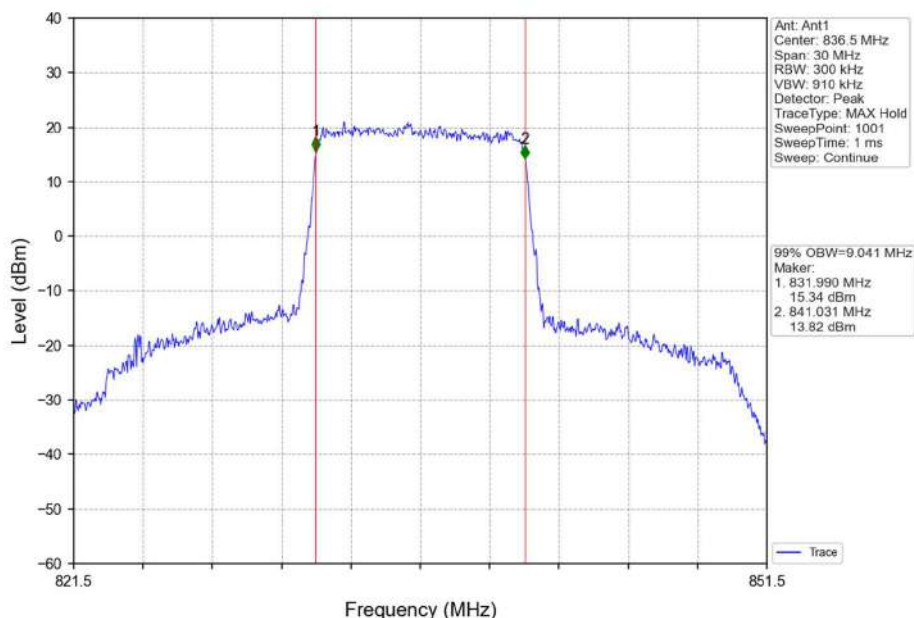
Band26b_10MHz_QPSK_MCH_836.5MHz_RB_50_0_NTNV
