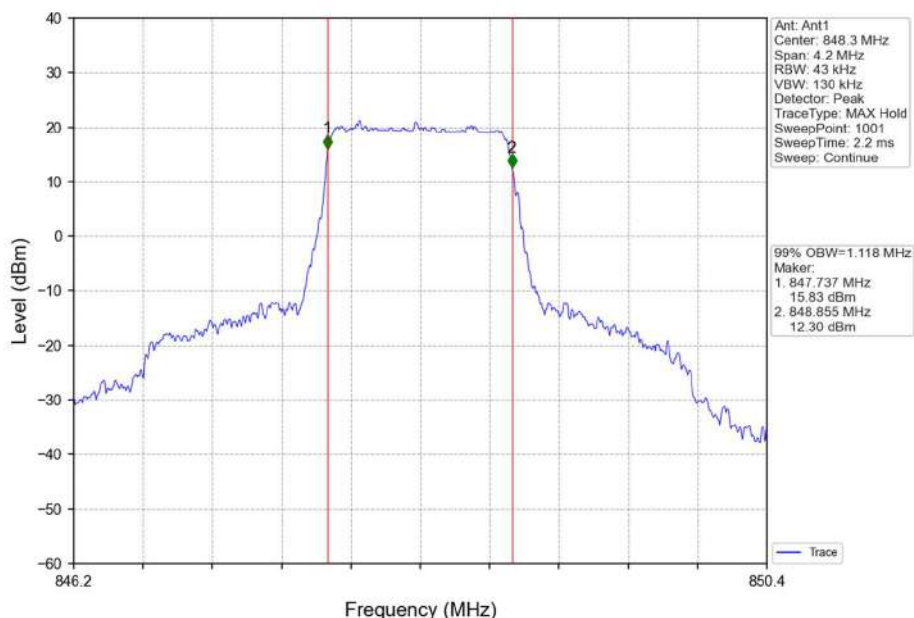
Band26b_1.4MHz_QPSK_HCH_848.3MHz_RB_6_0_NTNV
