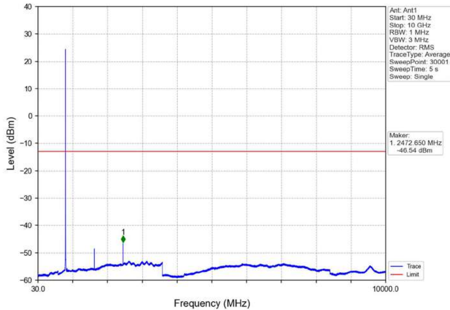
Band26b_3MHz_16QAM_LCH_825.5MHz_RB_1_0_NTNV
