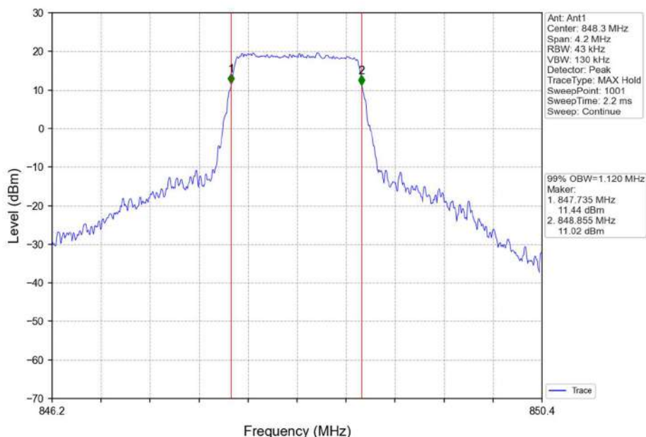
Band26b_1.4MHz_16QAM_HCH_848.3MHz_RB_6_0_NTNV
