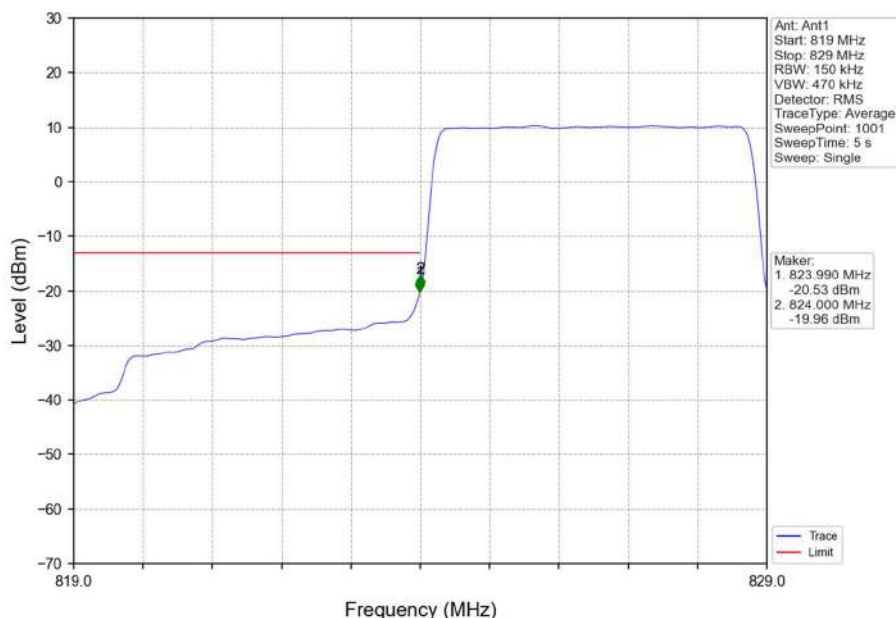
Band26b_5MHz_QPSK_LCH_826.5MHz_RB_25_0_NTNV
