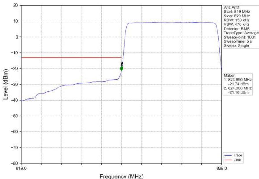
Band26b_5MHz_16QAM_LCH_826.5MHz_RB_25_0_NTNV
