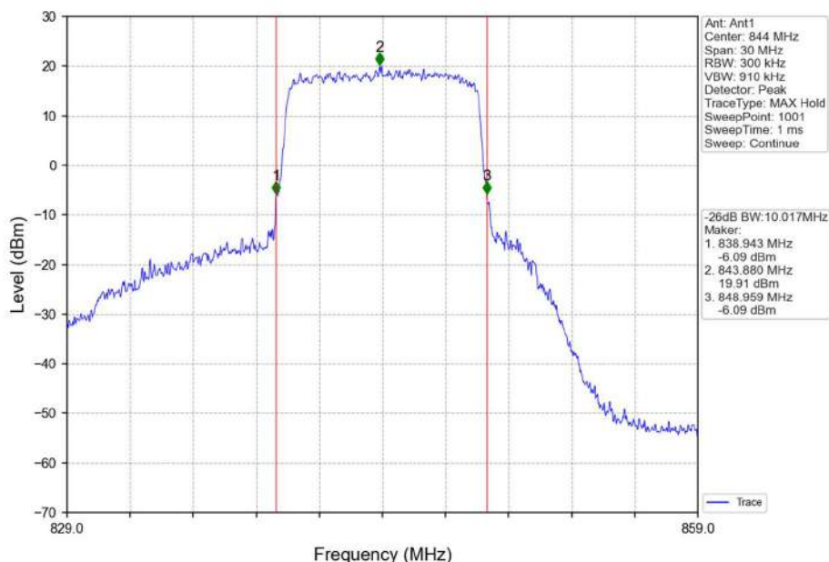
Band26b_10MHz_16QAM_HCH_844MHz_RB_50_0_NTNV
