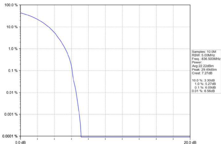
Band26b_10MHz_QPSK_MCH_836.5MHz_RB_50_0_NTNV
