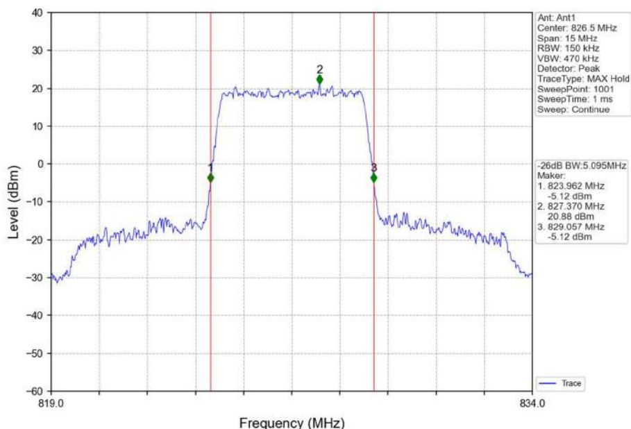
Band26b_5MHz_QPSK_LCH_826.5MHz_RB_25_0_NTNV
