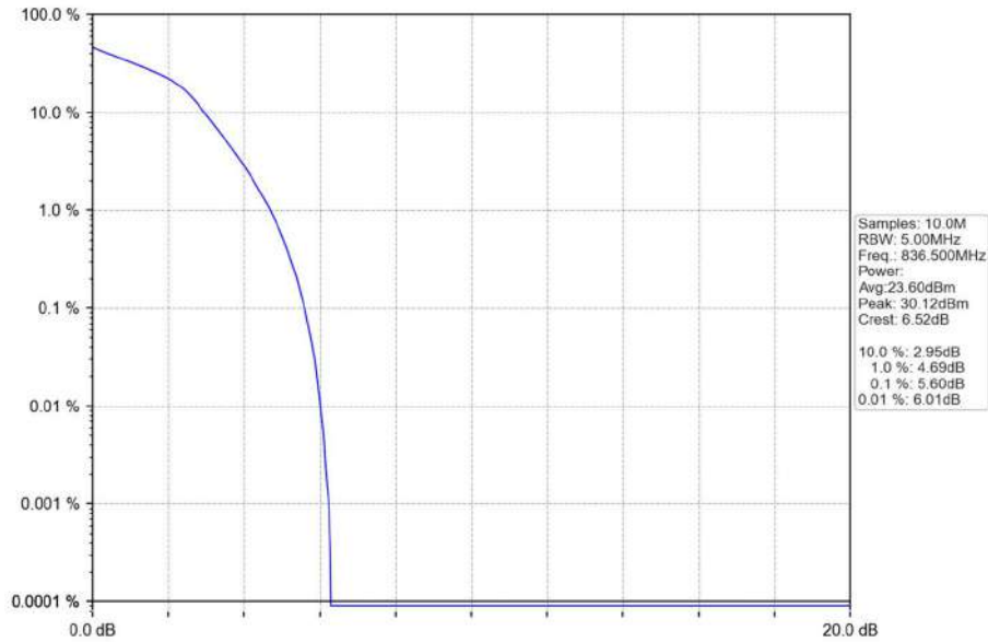
Band26b_1.4MHz_16QAM_MCH_836.5MHz_RB_6_0_NTNV
