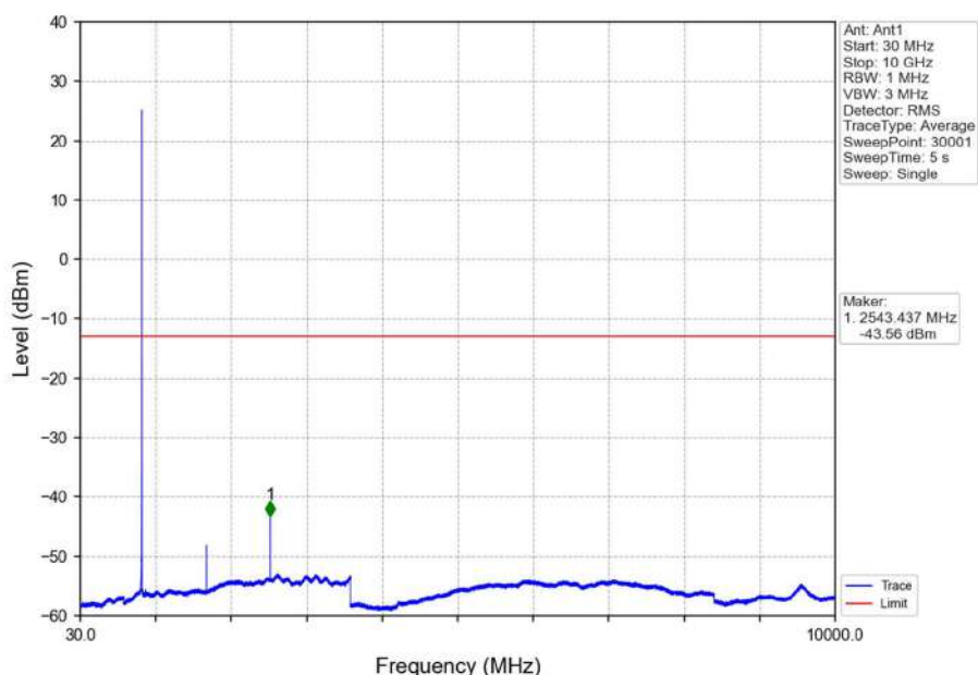
Band26b_1.4MHz_QPSK_HCH_848.3MHz_RB_1_0_NTNV
