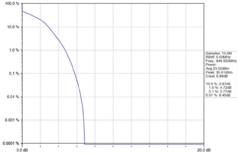
Band26b_5MHz_16QAM_HCH_846.5MHz_RB_25_0_NTNV
