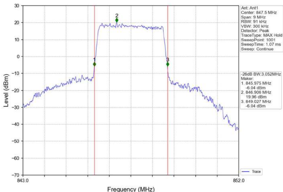
Band26b_3MHz_16QAM_HCH_847.5MHz_RB_15_0_NTNV
