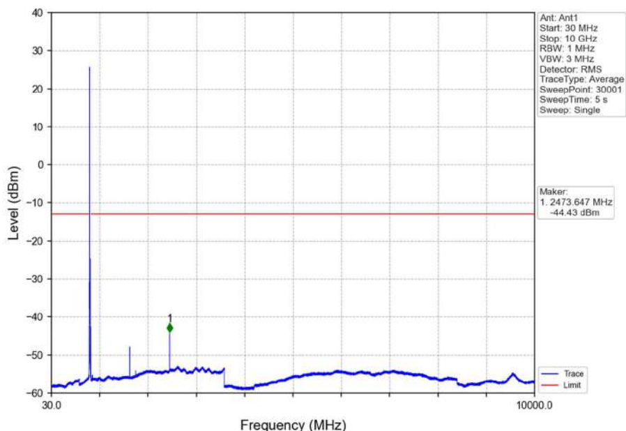
Band26b_10MHz_QPSK_LCH_829MHz_RB_1_0_NTNV
