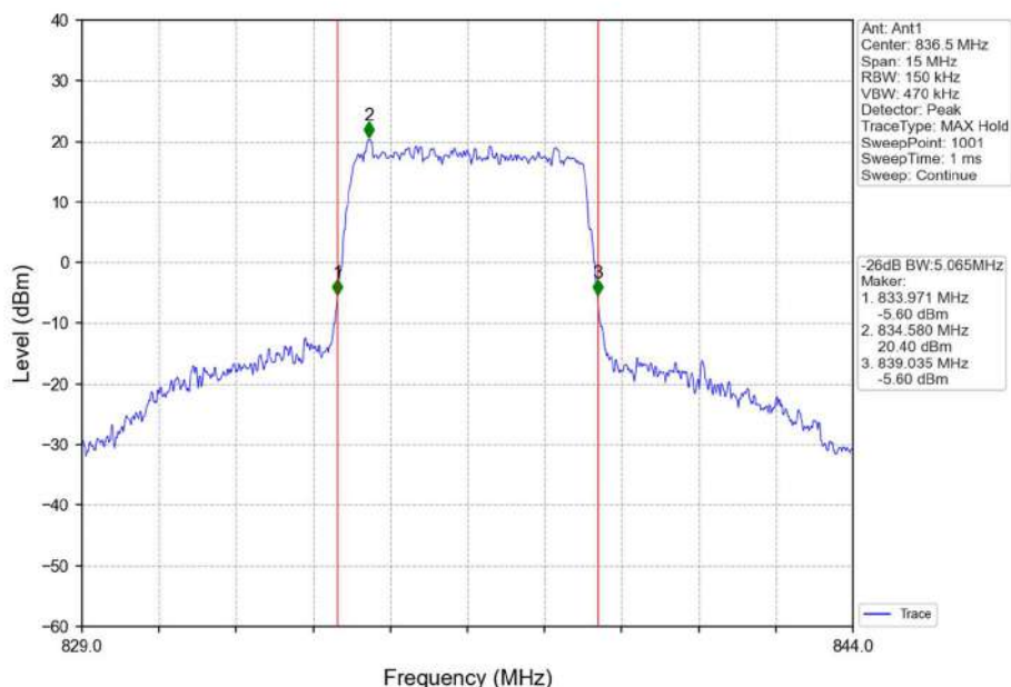
Band26b_5MHz_16QAM_MCH_836.5MHz_RB_25_0_NTNV
