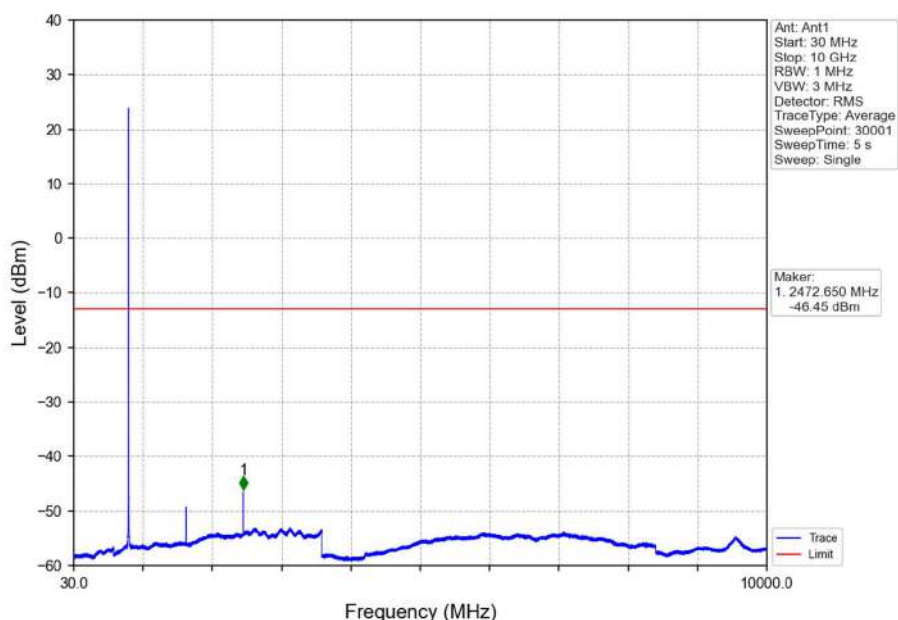
Band26b_1.4MHz_16QAM_LCH_824.7MHz_RB_1_0_NTNV
