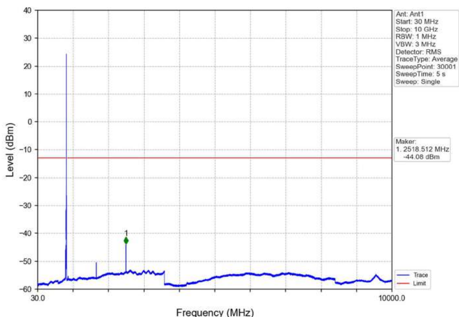
Band26b_10MHz_16QAM_HCH_844MHz_RB_1_0_NTNV
