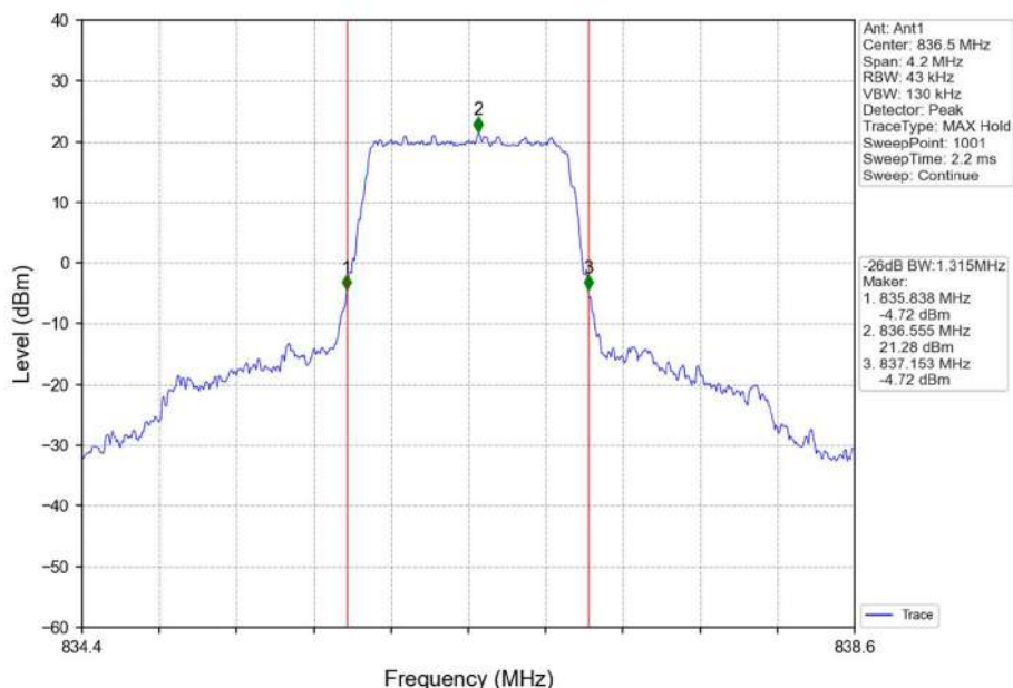
Band26b_1.4MHz_QPSK_MCH_836.5MHz_RB_6_0_NTNV
