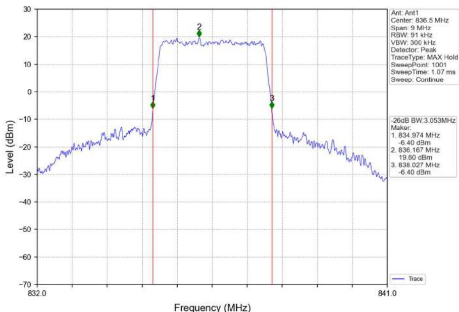
Band26b_3MHz_16QAM_MCH_836.5MHz_RB_15_0_NTNV
