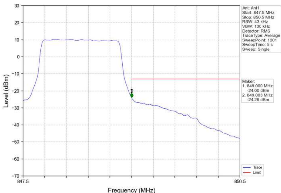
Band26b_1.4MHz_16QAM_HCH_848.3MHz_RB_6_0_NTNV
