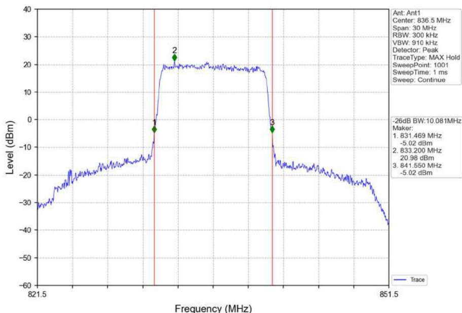
Band26b_10MHz_QPSK_MCH_836.5MHz_RB_50_0_NTNV
