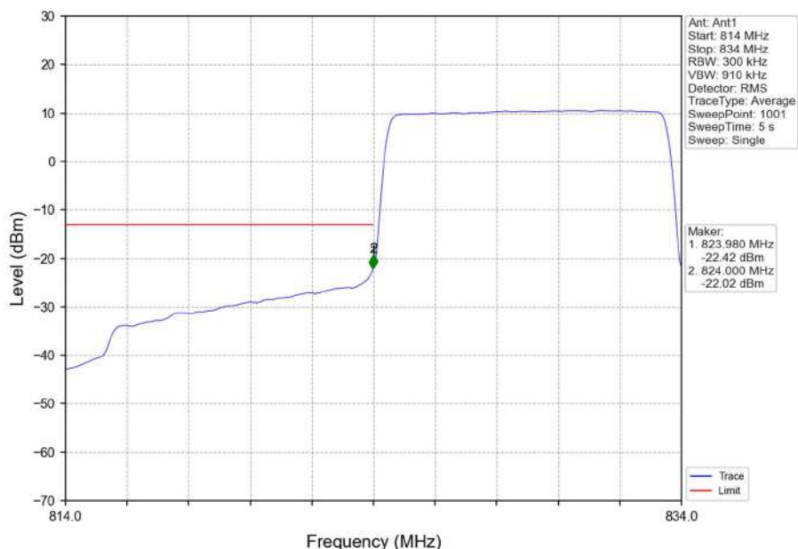
Band26b_10MHz_QPSK_LCH_829MHz_RB_50_0_NTNV
