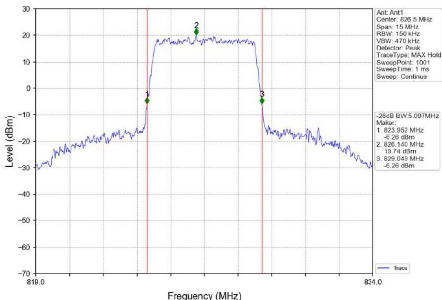
Band26b_5MHz_16QAM_LCH_826.5MHz_RB_25_0_NTNV
