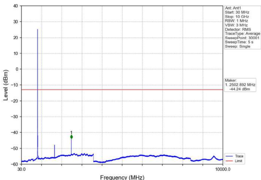
Band26b_5MHz_QPSK_MCH_836.5MHz_RB_1_0_NTNV
