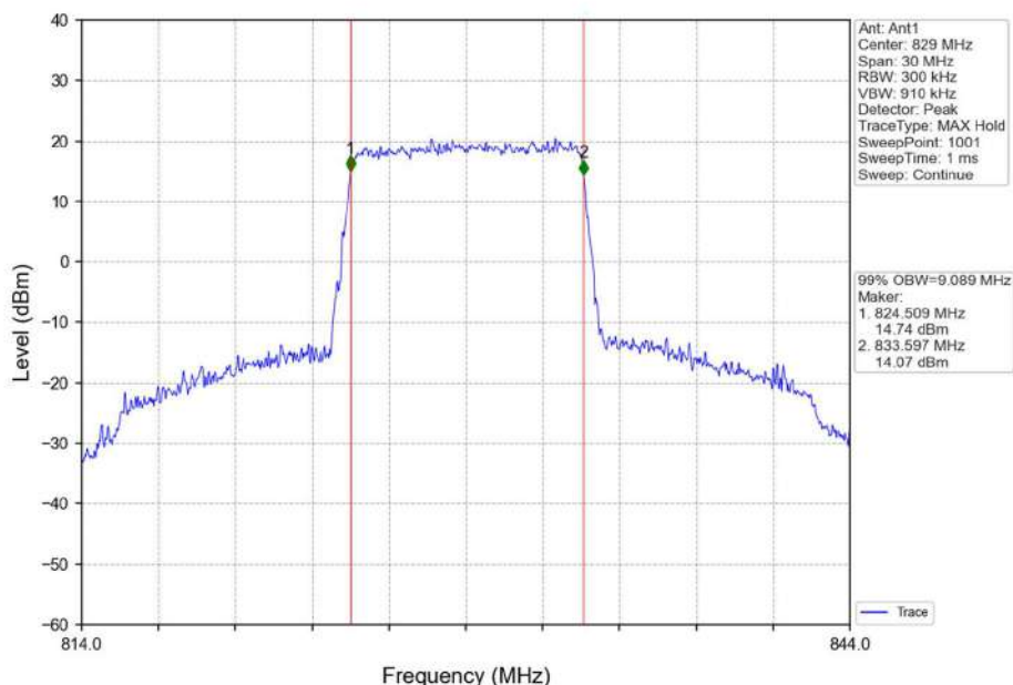
Band26b_10MHz_QPSK_LCH_829MHz_RB_50_0_NTNV
