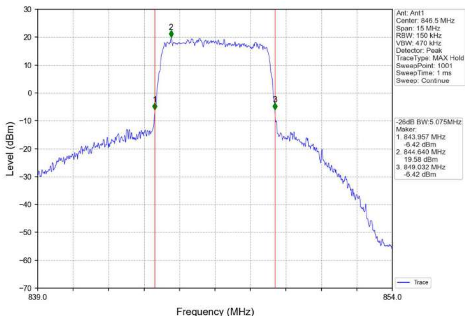
Band26b_5MHz_16QAM_HCH_846.5MHz_RB_25_0_NTNV
