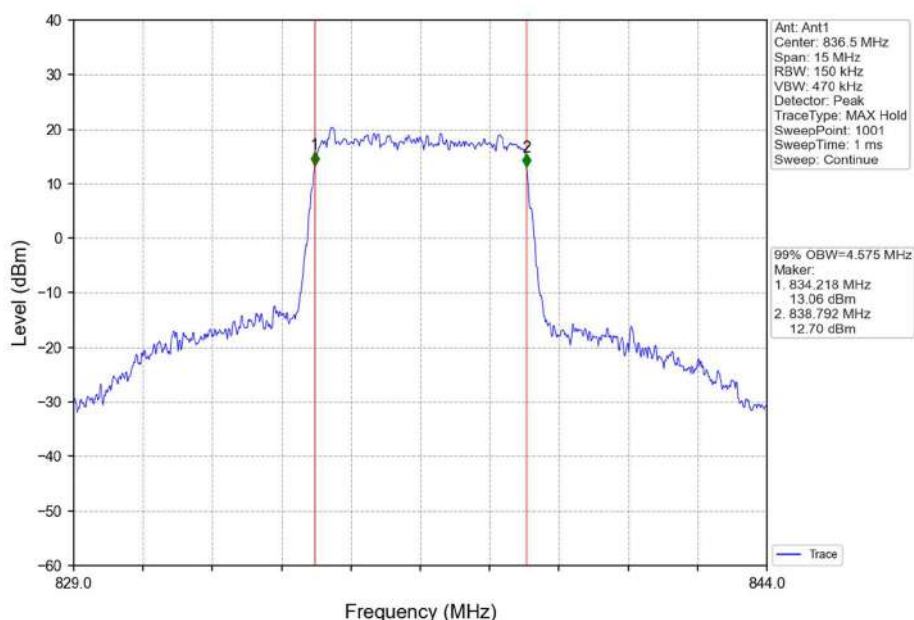
Band26b_5MHz_16QAM_MCH_836.5MHz_RB_25_0_NTNV
