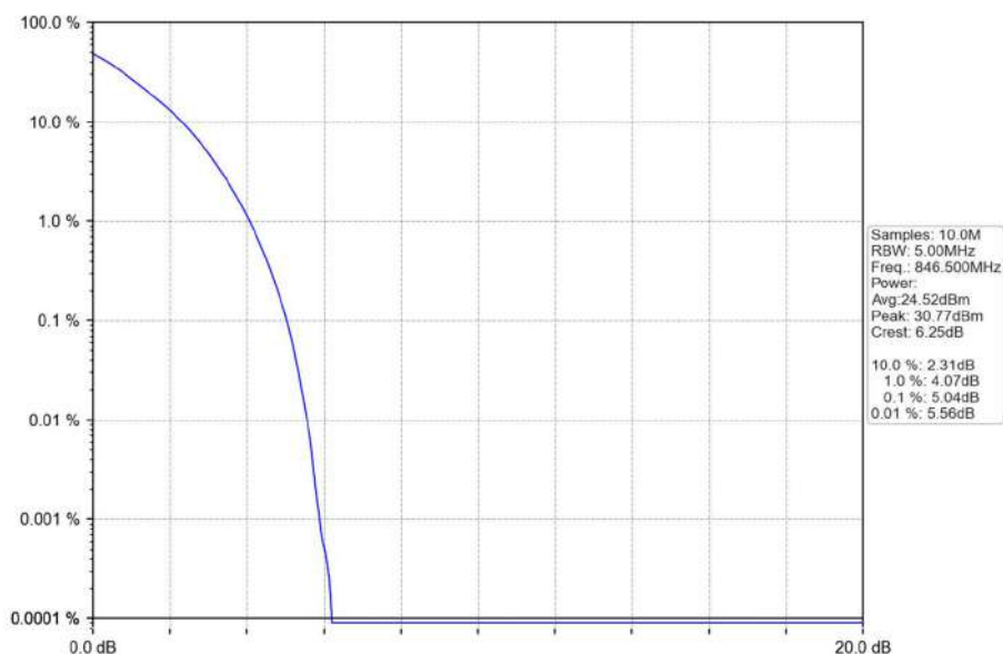
Band26b_5MHz_QPSK_HCH_846.5MHz_RB_25_0_NTNV
