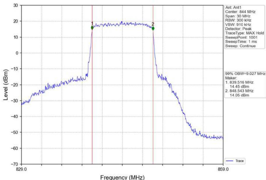
Band26b_10MHz_16QAM_HCH_844MHz_RB_50_0_NTNV
