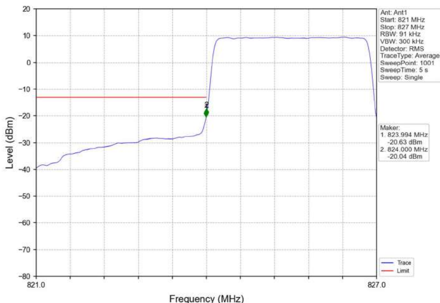
Band26b_3MHz_16QAM_LCH_825.5MHz_RB_15_0_NTNV
