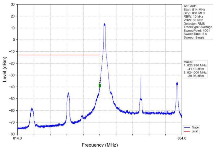
Band26b_10MHz_16QAM_LCH_829MHz_RB_1_0_NTNV
