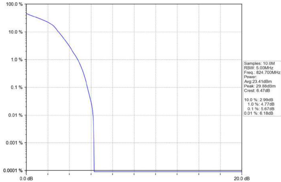
Band26b_1.4MHz_16QAM_LCH_824.7MHz_RB_6_0_NTNV
