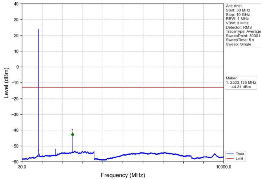
Band26b_5MHz_16QAM_HCH_846.5MHz_RB_1_0_NTNV
