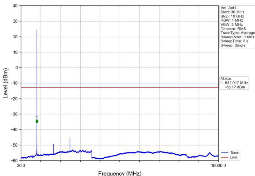
Band26b_1.4MHz_16QAM_MCH_836.5MHz_RB_1_0_NTNV
