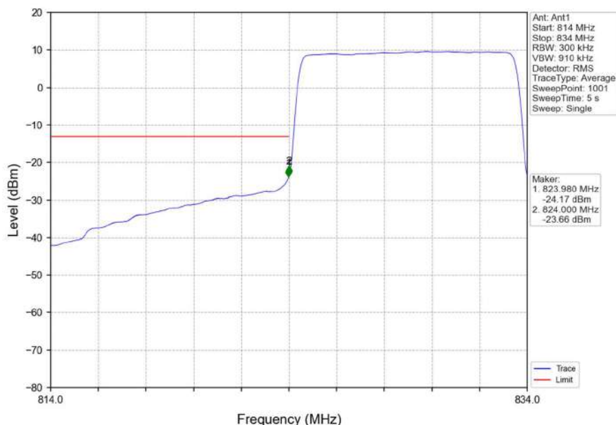
Band26b_10MHz_16QAM_LCH_829MHz_RB_50_0_NTNV
