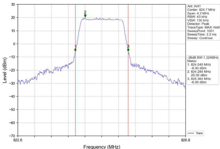
Band26b_1.4MHz_16QAM_LCH_824.7MHz_RB_6_0_NTNV
