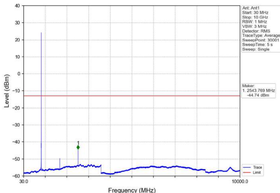
Band26b_1.4MHz_16QAM_HCH_848.3MHz_RB_1_0_NTNV
