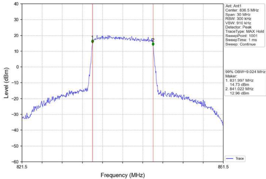
Band26b_10MHz_16QAM_MCH_836.5MHz_RB_50_0_NTNV
