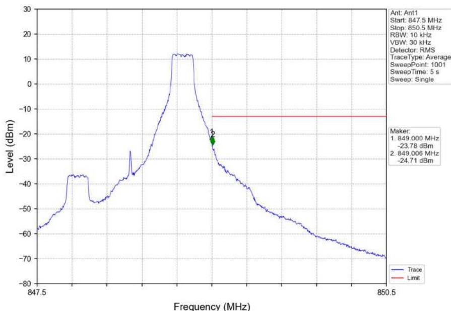
Band26b_1.4MHz_16QAM_HCH_848.3MHz_RB_1_5_NTNV
