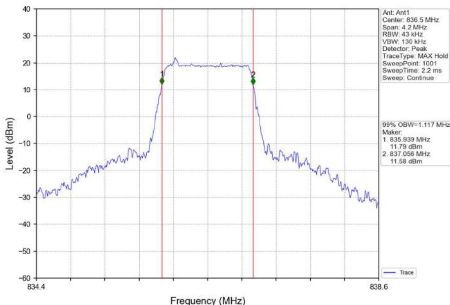
Band26b_1.4MHz_16QAM_MCH_836.5MHz_RB_6_0_NTNV
