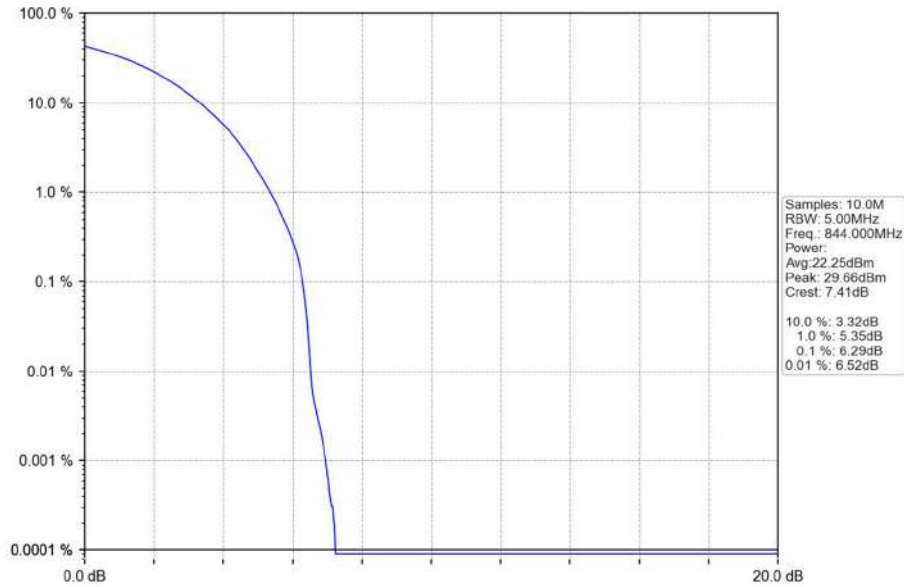
Band26b_10MHz_QPSK_HCH_844MHz_RB_50_0_NTNV
