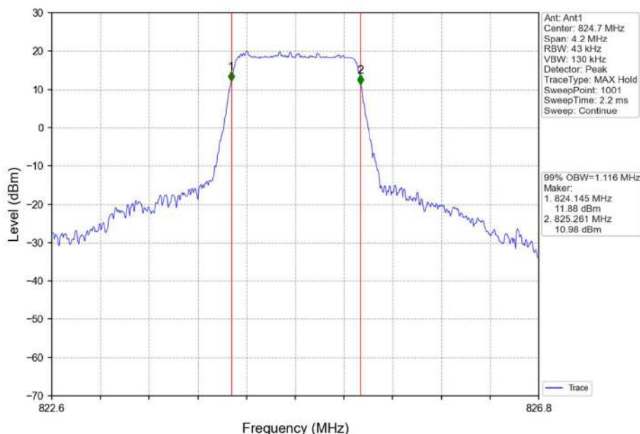
Band26b_1.4MHz_16QAM_LCH_824.7MHz_RB_6_0_NTNV
