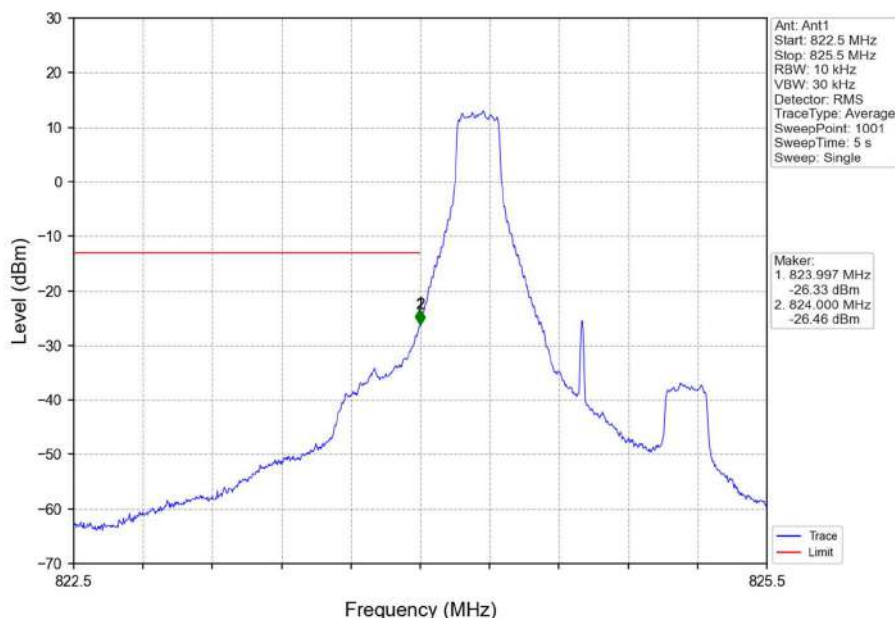
Band26b_1.4MHz_16QAM_LCH_824.7MHz_RB_1_0_NTNV
