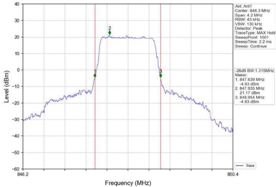
Band26b_1.4MHz_QPSK_HCH_848.3MHz_RB_6_0_NTNV
