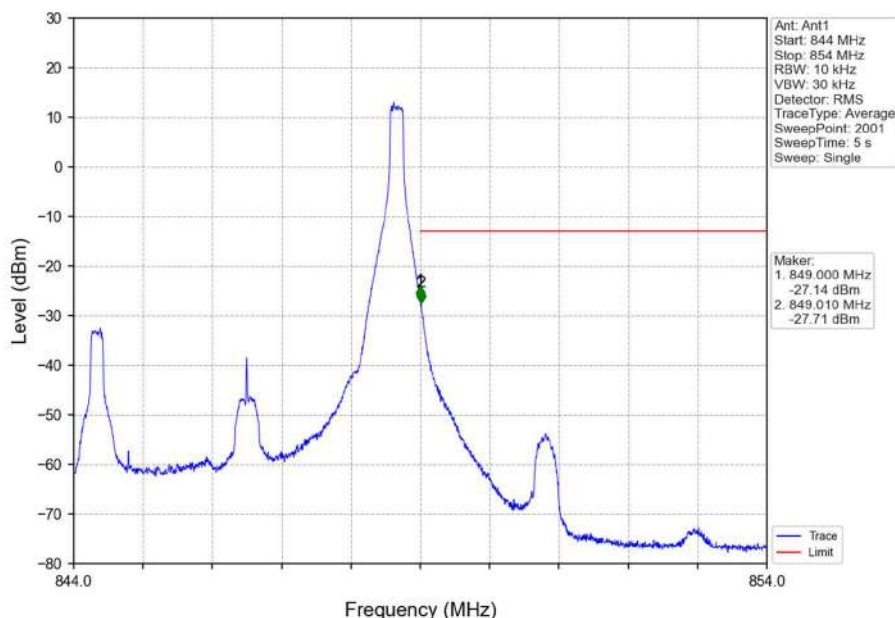
Band26b_5MHz_16QAM_HCH_846.5MHz_RB_1_24_NTNV
