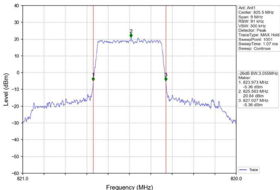
Band26b_3MHz_QPSK_LCH_825.5MHz_RB_15_0_NTNV
