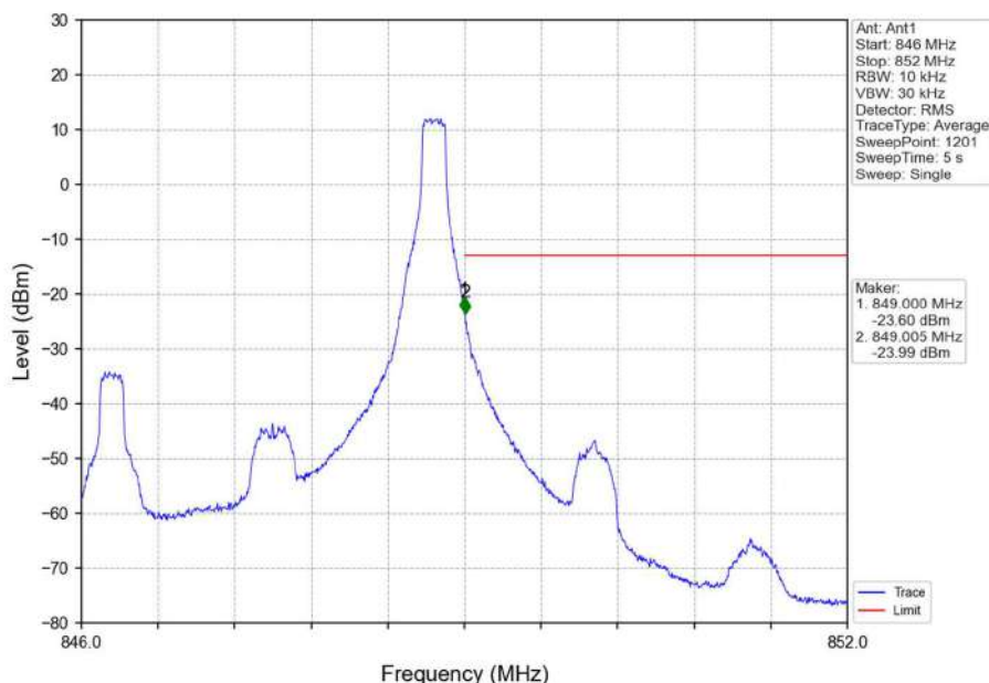
Band26b_3MHz_16QAM_HCH_847.5MHz_RB_1_14_NTNV
