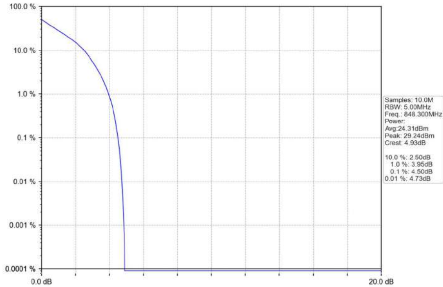
Band26b_1.4MHz_QPSK_HCH_848.3MHz_RB_6_0_NTNV
