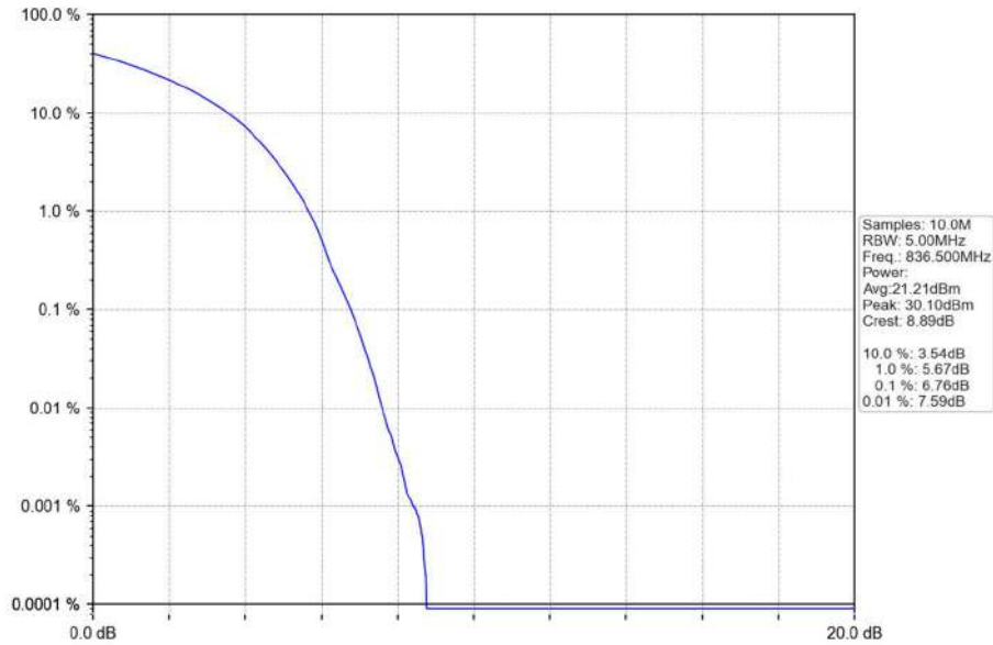
Band26b_10MHz_16QAM_MCH_836.5MHz_RB_50_0_NTNV
