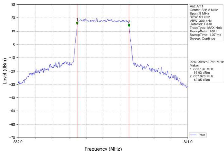
Band26b_3MHz_16QAM_MCH_836.5MHz_RB_15_0_NTNV
