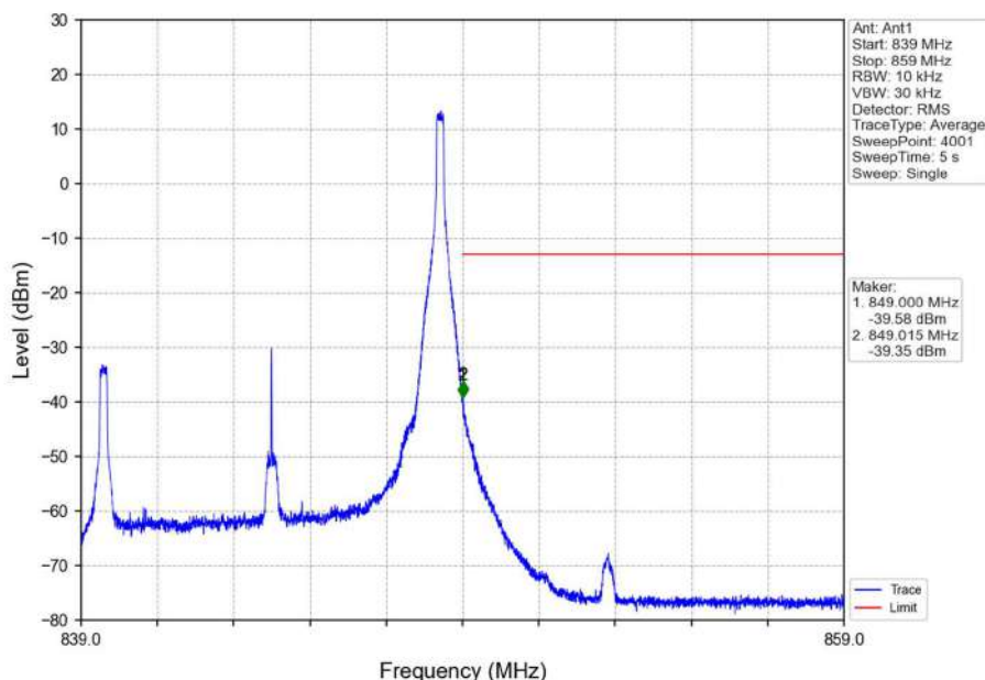
Band26b_10MHz_16QAM_HCH_844MHz_RB_1_49_NTNV
