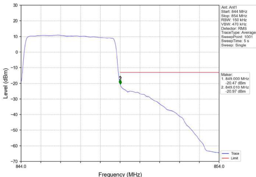
Band26b_5MHz_QPSK_HCH_846.5MHz_RB_25_0_NTNV
