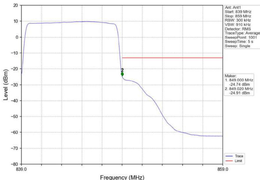
Band26b_10MHz_16QAM_HCH_844MHz_RB_50_0_NTNV
