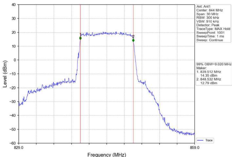
Band26b_10MHz_QPSK_HCH_844MHz_RB_50_0_NTNV
