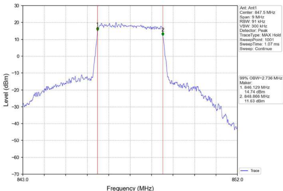
Band26b_3MHz_16QAM_HCH_847.5MHz_RB_15_0_NTNV
