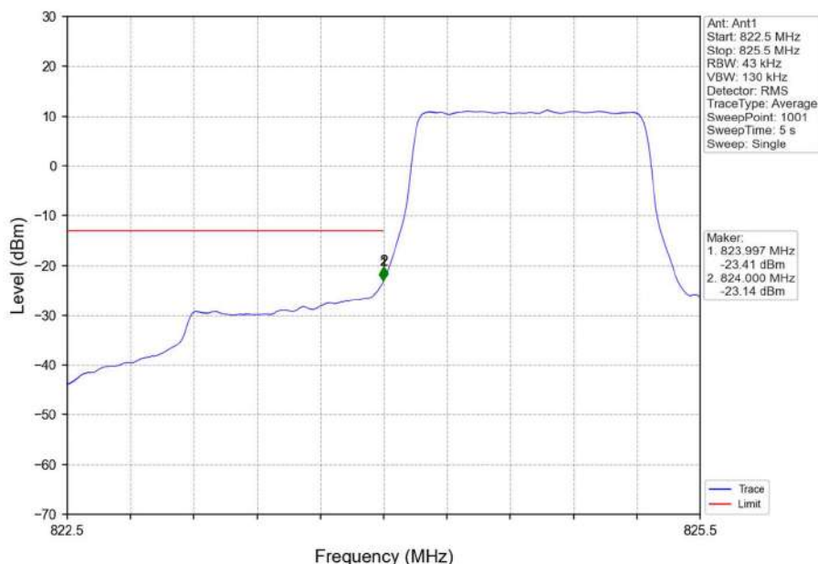
Band26b_1.4MHz_QPSK_LCH_824.7MHz_RB_6_0_NTNV
