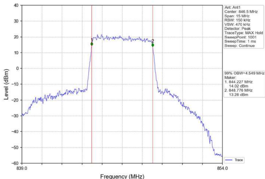
Band26b_5MHz_QPSK_HCH_846.5MHz_RB_25_0_NTNV
