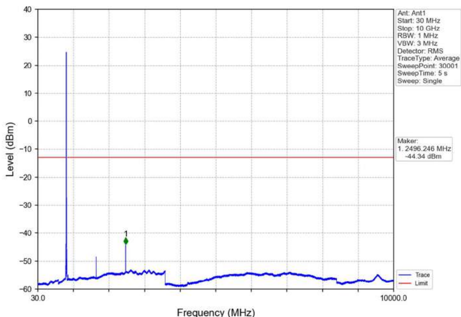
Band26b_10MHz_16QAM_MCH_836.5MHz_RB_1_0_NTNV
