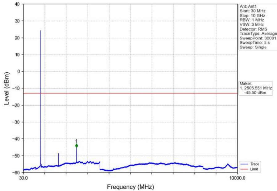
Band26b_3MHz_16QAM_MCH_836.5MHz_RB_1_0_NTNV
