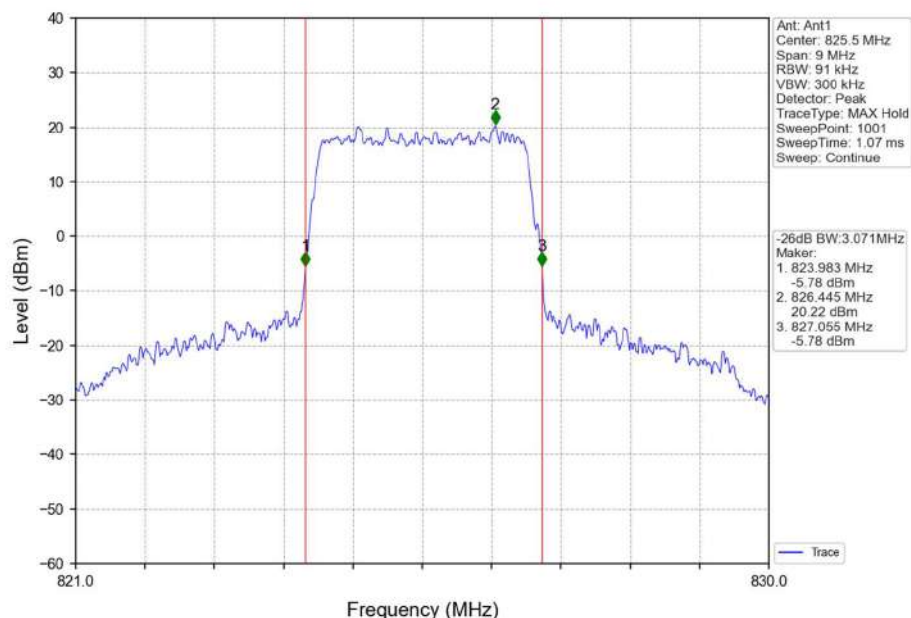
Band26b_3MHz_16QAM_LCH_825.5MHz_RB_15_0_NTNV
