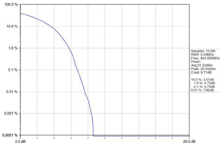
Band26b_10MHz_16QAM_HCH_844MHz_RB_50_0_NTNV
