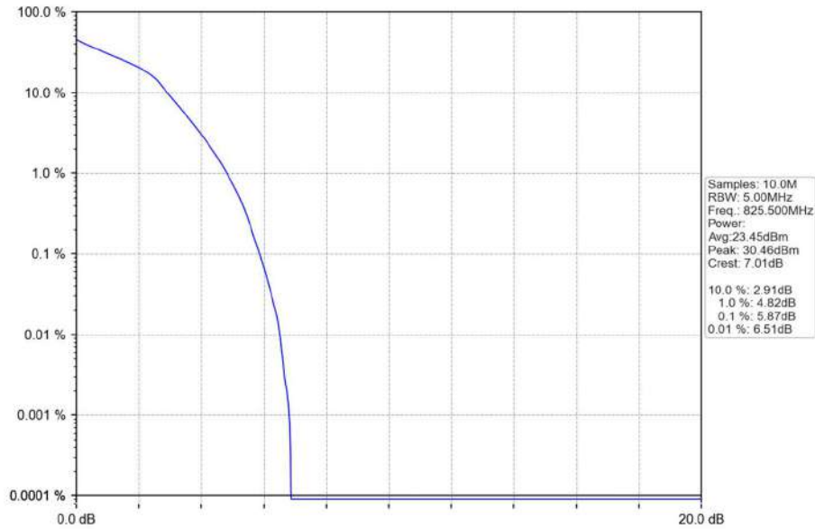
Band26b_3MHz_16QAM_LCH_825.5MHz_RB_15_0_NTNV
