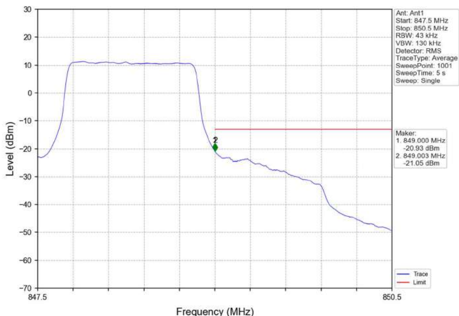
Band26b_1.4MHz_QPSK_HCH_848.3MHz_RB_6_0_NTNV
