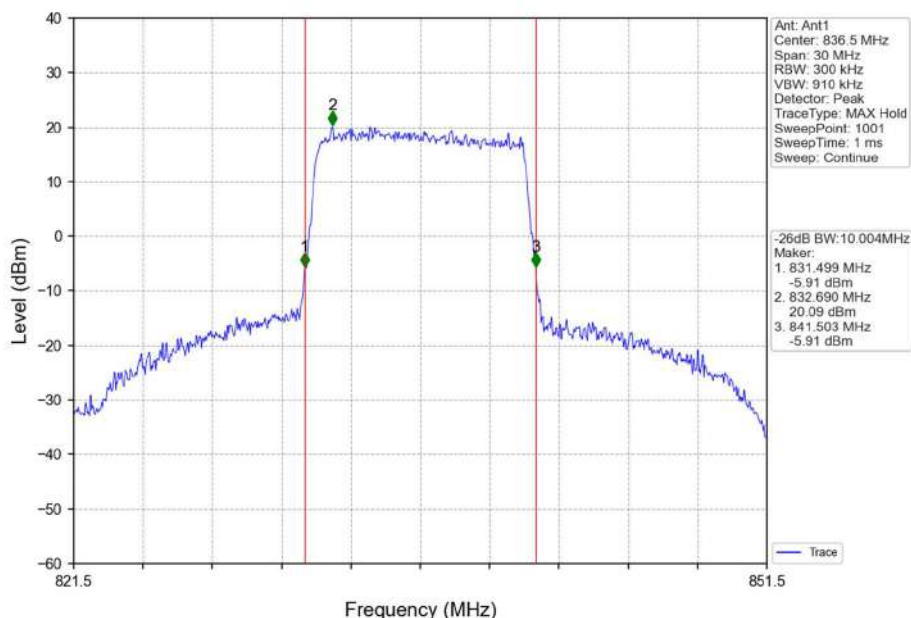
Band26b_10MHz_16QAM_MCH_836.5MHz_RB_50_0_NTNV
