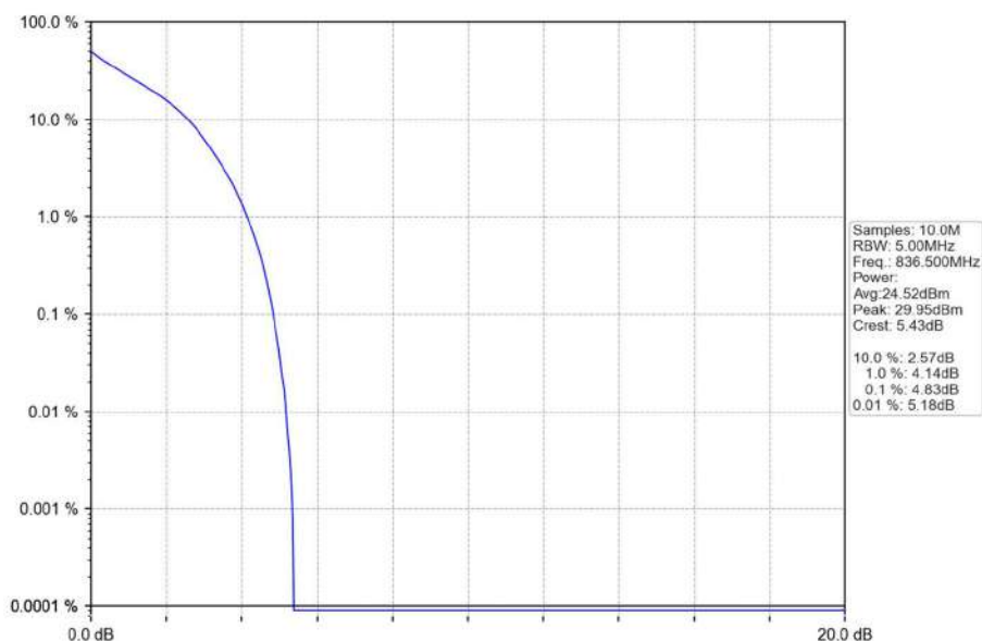
Band26b_1.4MHz_QPSK_MCH_836.5MHz_RB_6_0_NTNV
