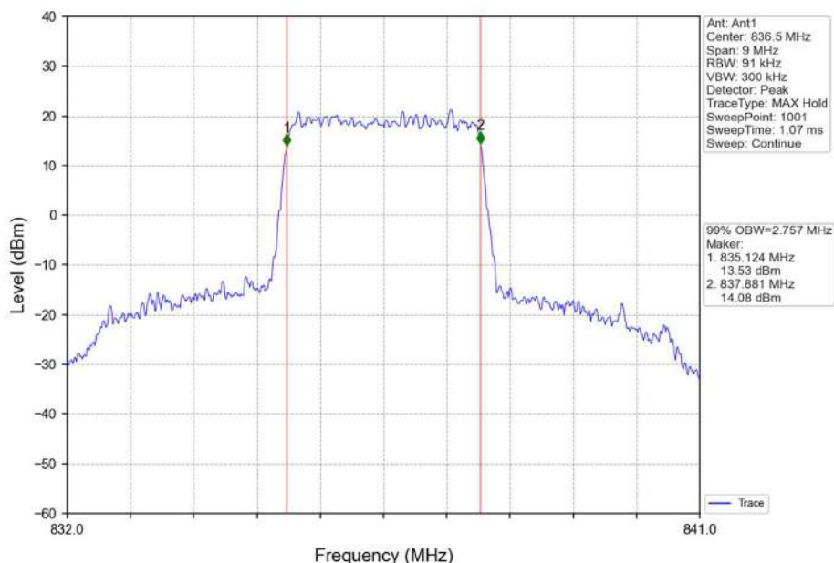
Band26b_3MHz_QPSK_MCH_836.5MHz_RB_15_0_NTNV
