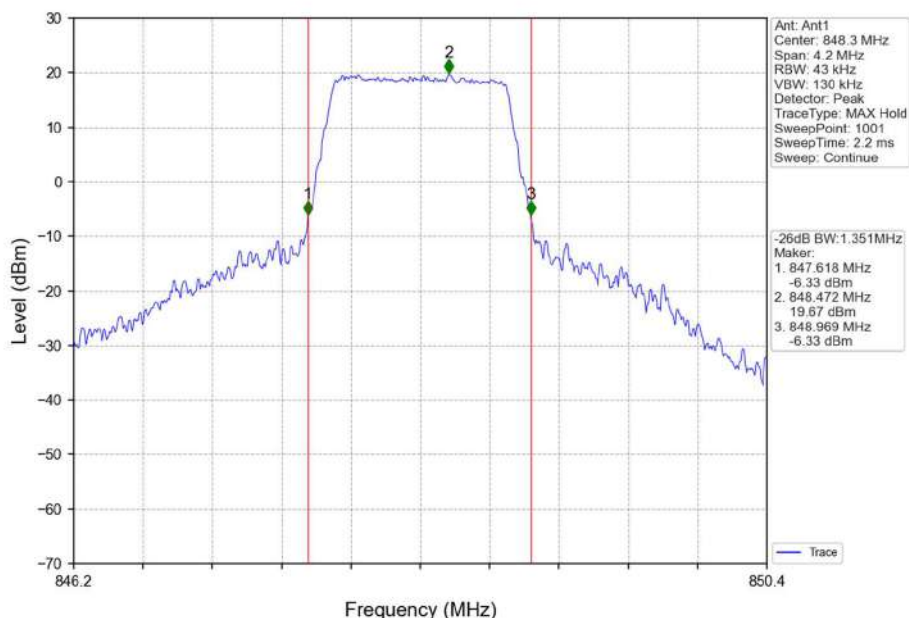
Band26b_1.4MHz_16QAM_HCH_848.3MHz_RB_6_0_NTNV
