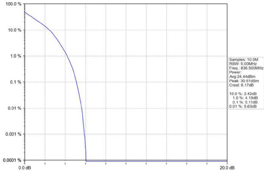
Band26b_3MHz_QPSK_MCH_836.5MHz_RB_15_0_NTNV
