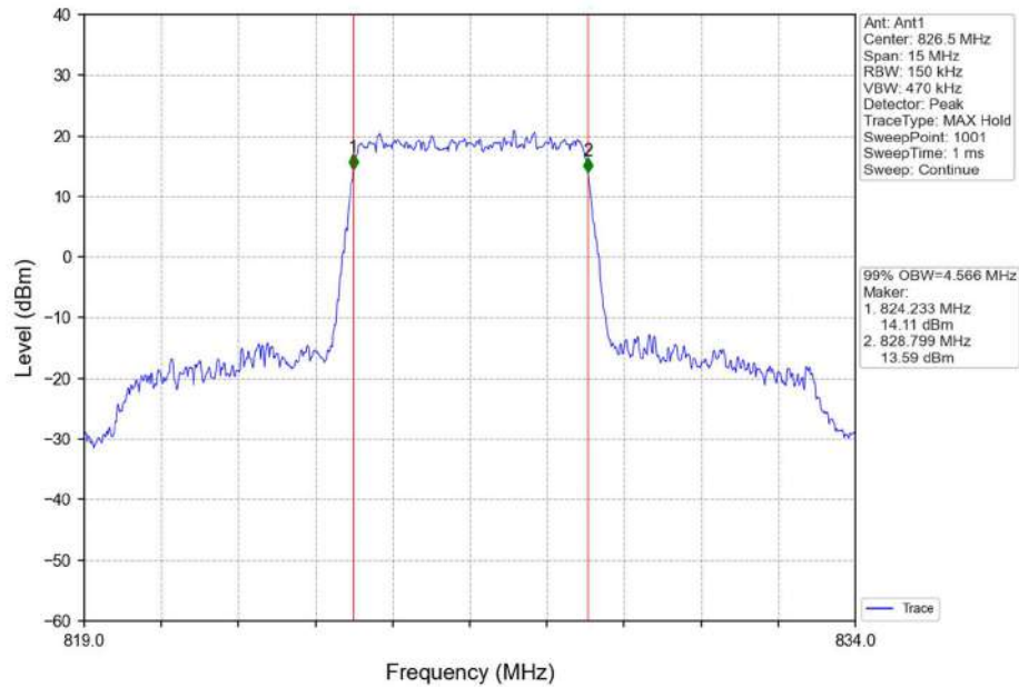
Band26b_5MHz_QPSK_LCH_826.5MHz_RB_25_0_NTNV
