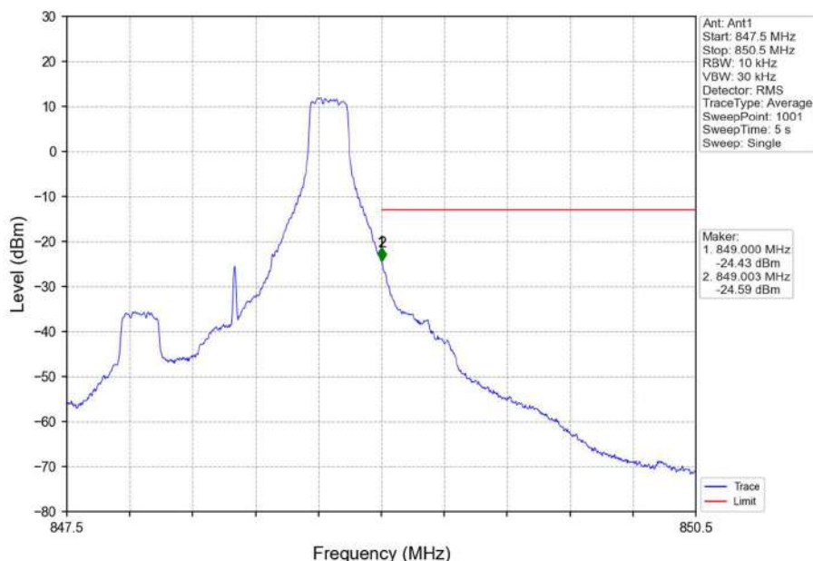
Band26b_1.4MHz_QPSK_HCH_848.3MHz_RB_1_5_NTNV
