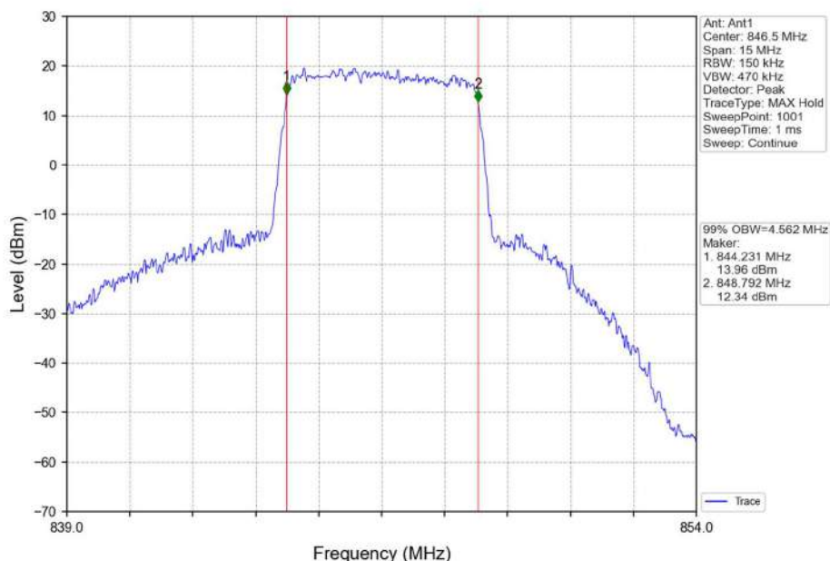
Band26b_5MHz_16QAM_HCH_846.5MHz_RB_25_0_NTNV
