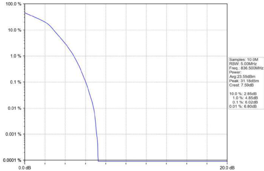
Band26b_5MHz_16QAM_MCH_836.5MHz_RB_25_0_NTNV
