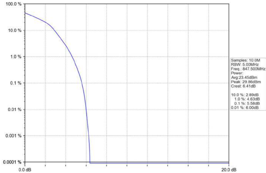
Band26b_3MHz_16QAM_HCH_847.5MHz_RB_15_0_NTNV
