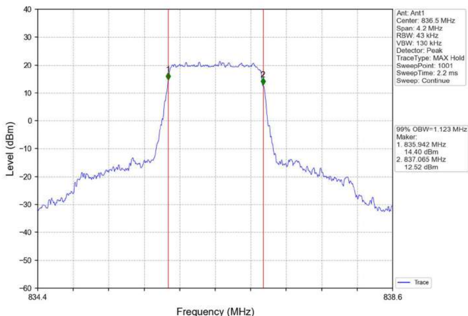
Band26b_1.4MHz_QPSK_MCH_836.5MHz_RB_6_0_NTNV
