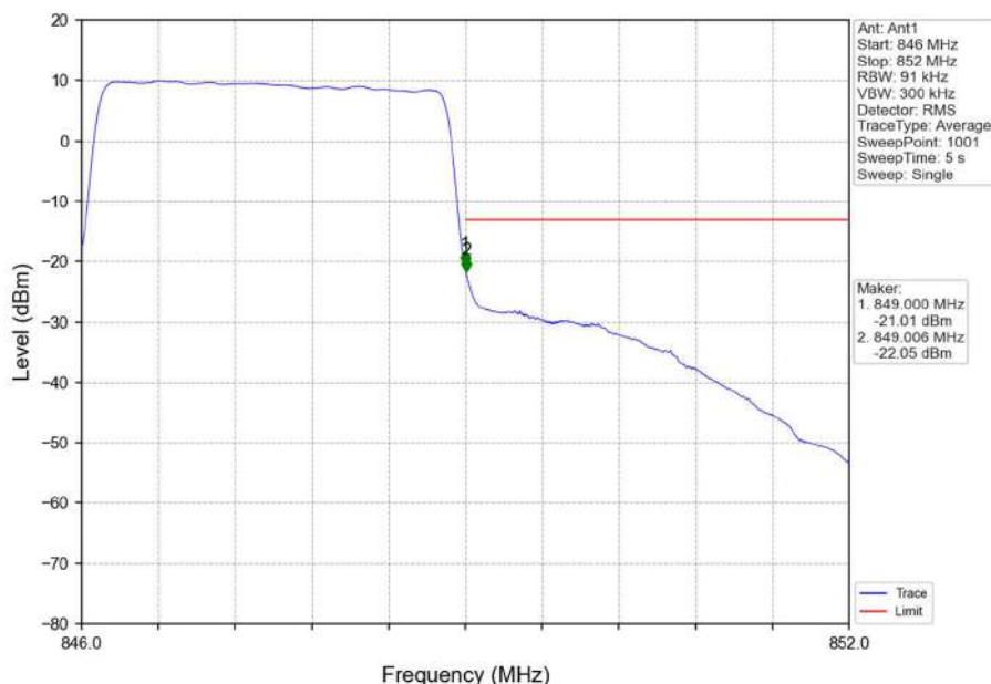
Band26b_3MHz_16QAM_HCH_847.5MHz_RB_15_0_NTNV
