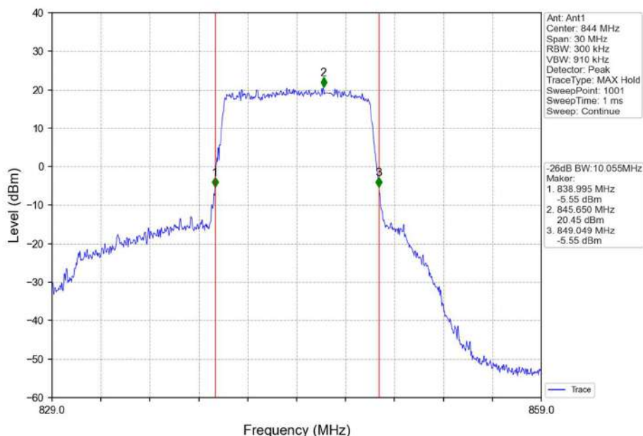
Band26b_10MHz_QPSK_HCH_844MHz_RB_50_0_NTNV
