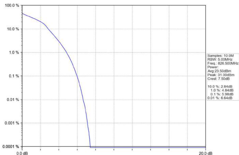
Band26b_5MHz_16QAM_LCH_826.5MHz_RB_25_0_NTNV
