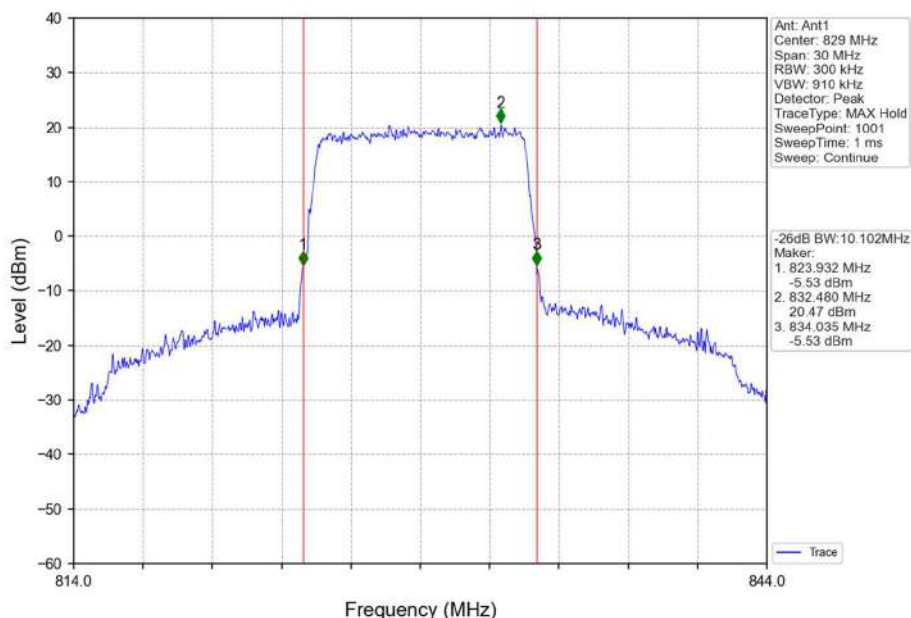
Band26b_10MHz_QPSK_LCH_829MHz_RB_50_0_NTNV
