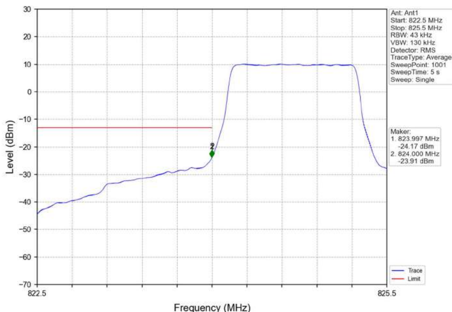
Band26b_1.4MHz_16QAM_LCH_824.7MHz_RB_6_0_NTNV
