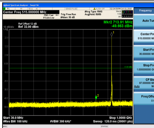
Band26_3MHz_16QAM_20525_1RB#0
