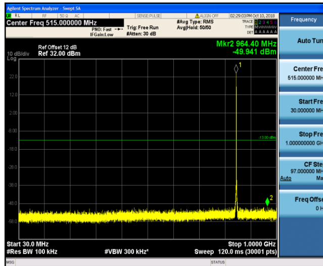
Band26_1.4MHz_16QAM_20643_1RB#0
