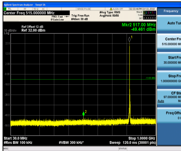
Band26_3MHz_16QAM_20415_1RB#0
