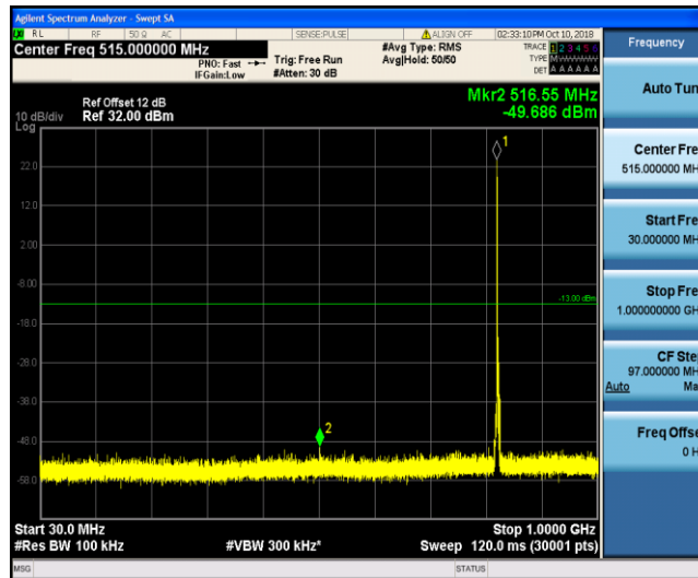
Band26_3MHz_QPSK_20415_1RB#0
