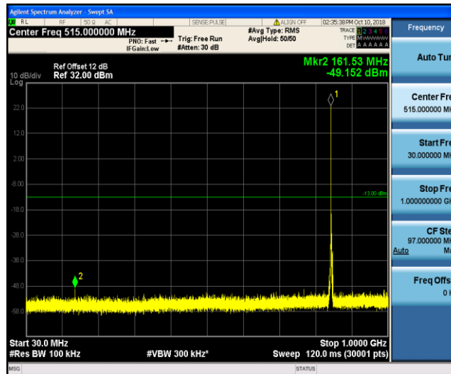
Band26_3MHz_QPSK_20635_1RB#0
