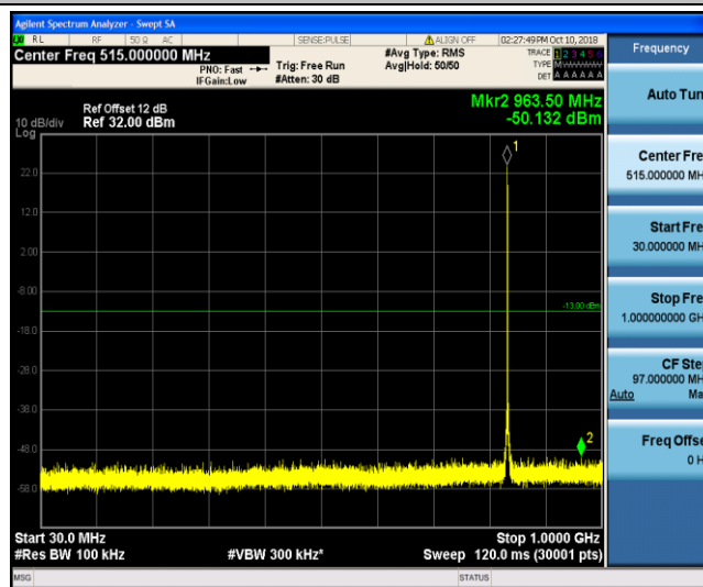
Band26_1.4MHz_16QAM_20525_1RB#0
