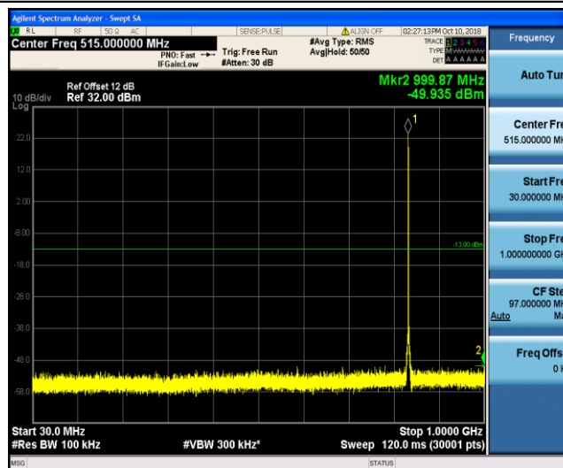
Band26_1.4MHz_QPSK_20525_1RB#0
