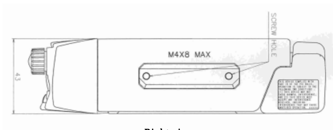
Right view
