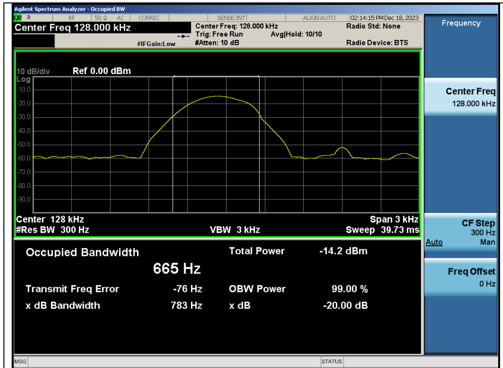
Test_Graph_ASK_Coil ANT_ 128kHz _ -20dB Bandwidth
