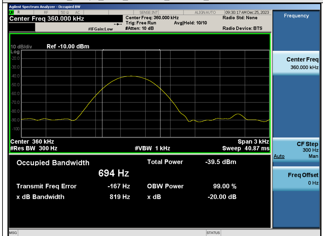
Test_Graph_ASK_Coil ANT_ 360kHz _ -20dB Bandwidth
