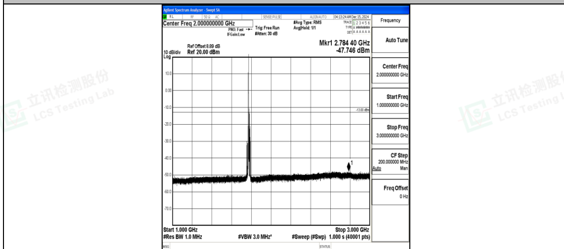
Band66_10MHz_QPSK_132622_1RB#0_1000~3000.01000~3000
