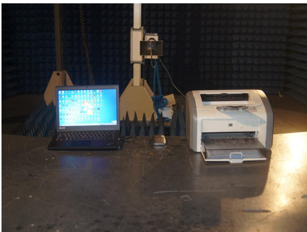
Photograph 6: Set-up for Radiated emissions above 1GHz, Battery Charging with PC
