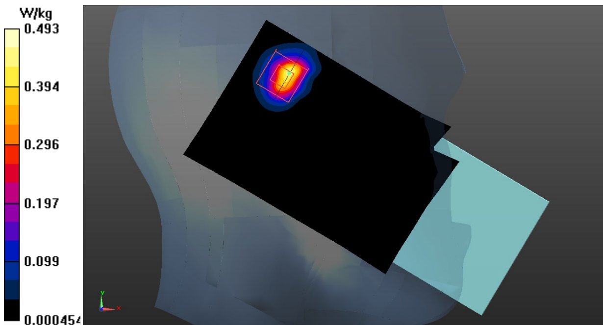
Fig.33 Bluetooth Head
