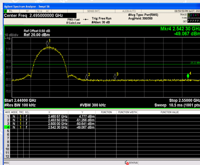
802.11b_High Channel
