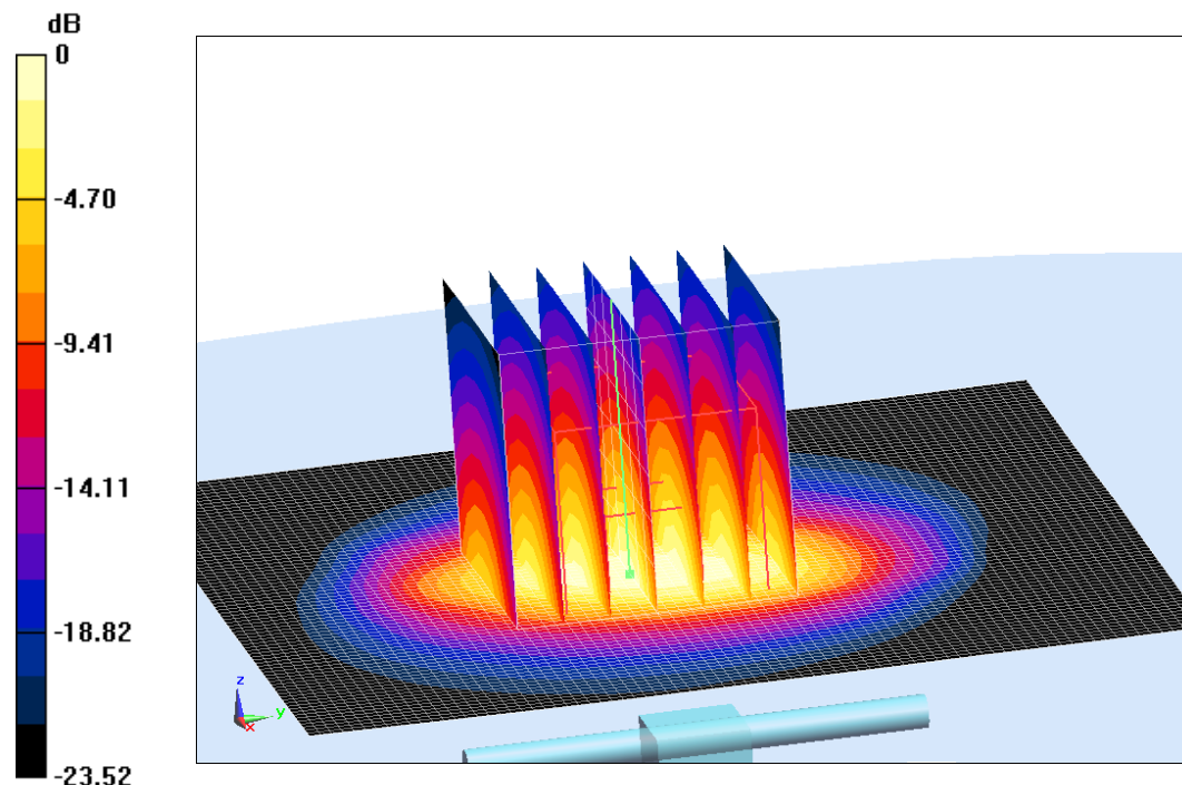
Fig.B.5 validation 2550 MHz 250mW
