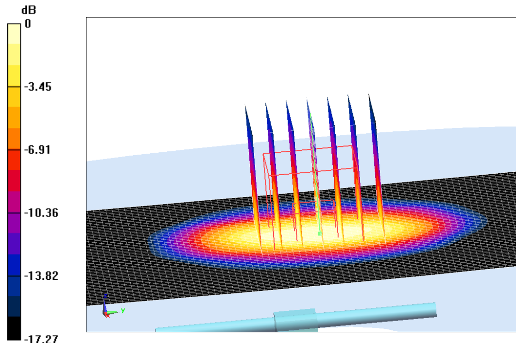
Fig.B.3 validation 1900 MHz 250mW
