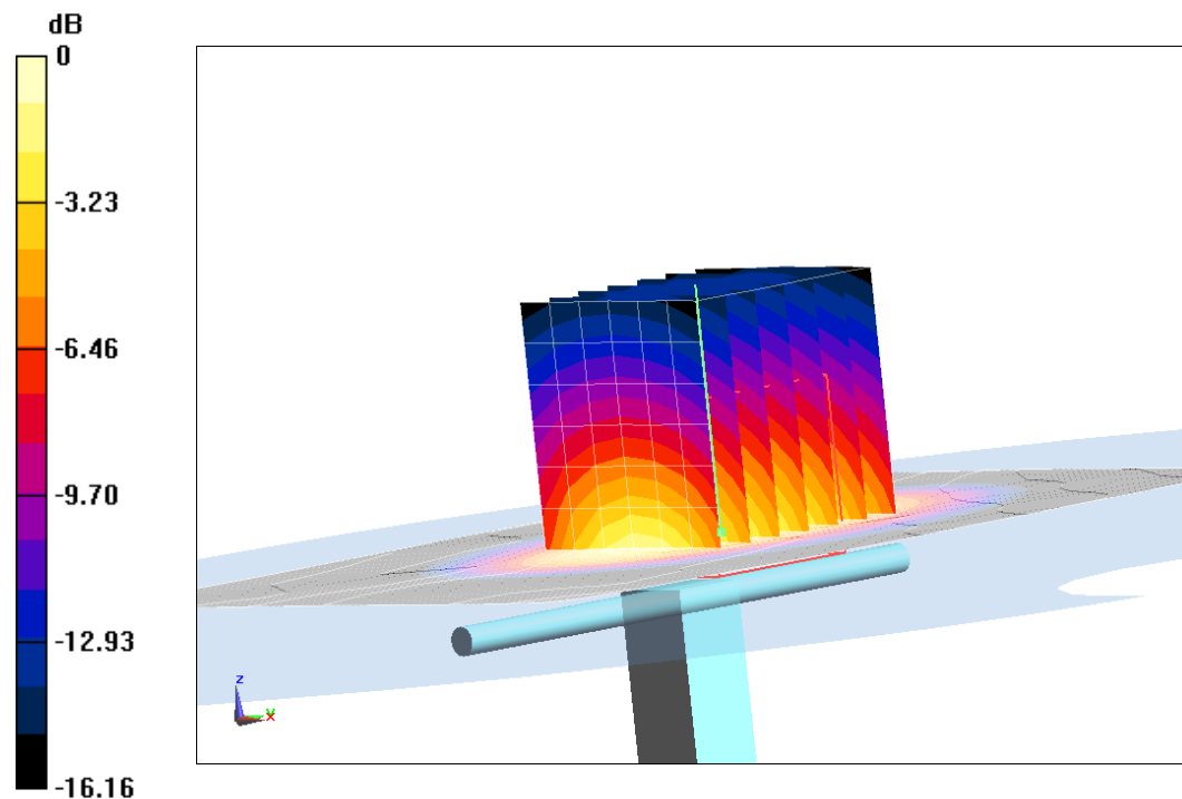
Fig.B.2 validation 1750 MHz 250mW
