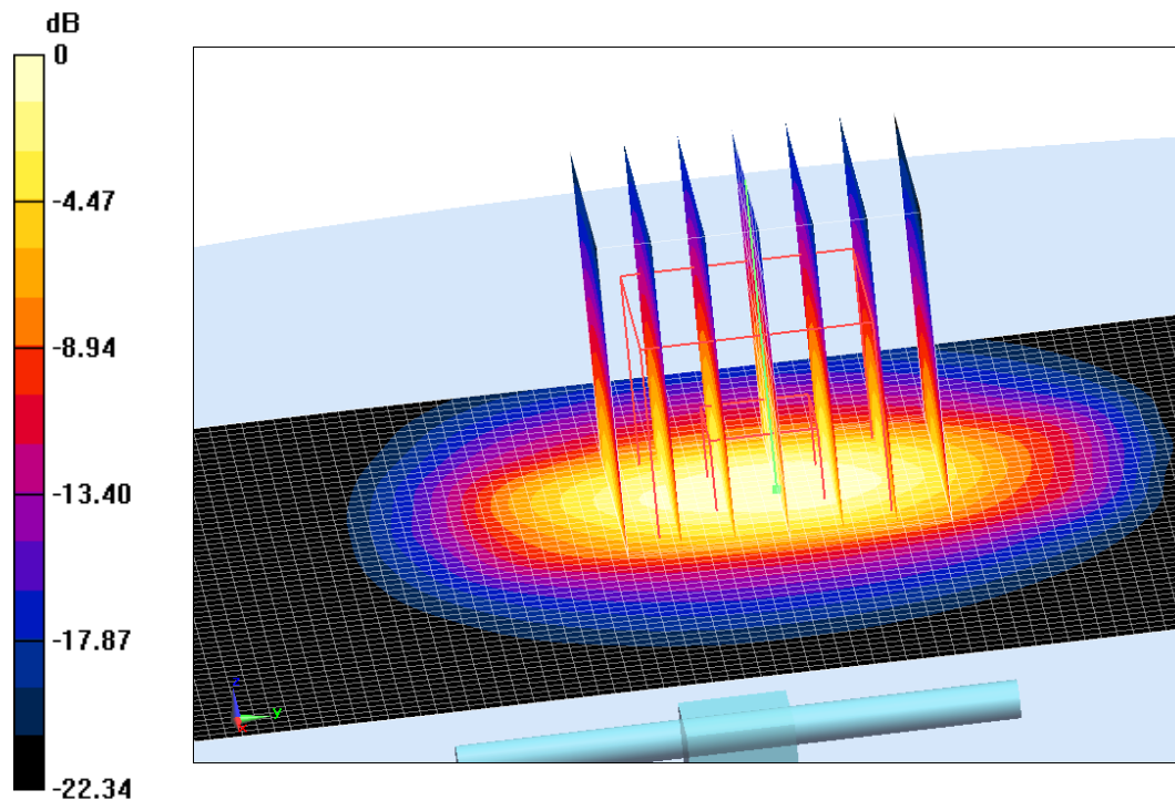
Fig.B.4 validation 2450 MHz 250mW
