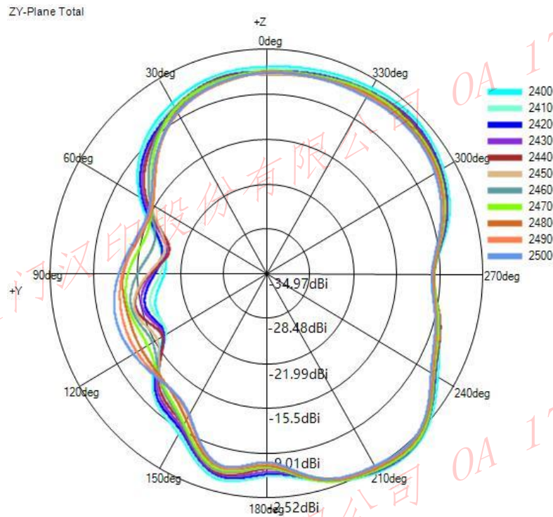
(2) Y-Z Plane(unit:dBi):
