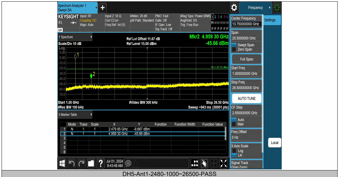
DH5-Ant1-2480-1000~26500-PASS
