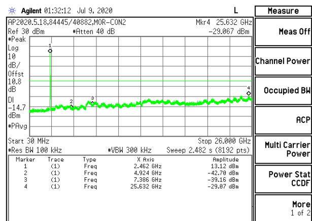
OUT-OF-BAND HIGH CHANNEL 11 CHAIN 0
