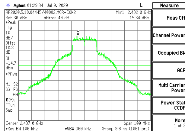
IN-BAND REFERENCE LEVEL CHAIN 0
