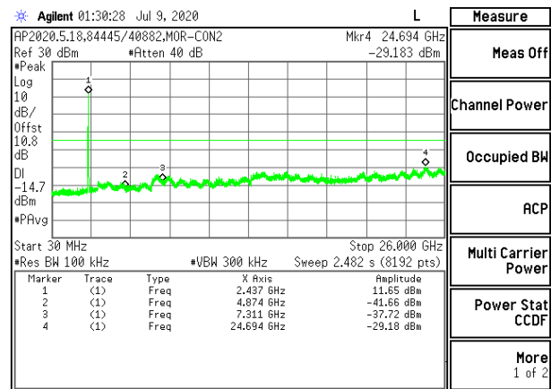
OUT-OF-BAND MID CHANNEL CHAIN 0
