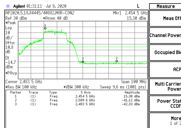
HIGH CHANNEL 11 BANDEDGE CHAIN 0
