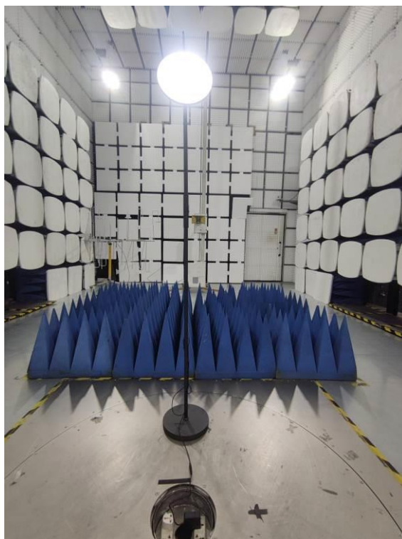
Above 1 GHz
