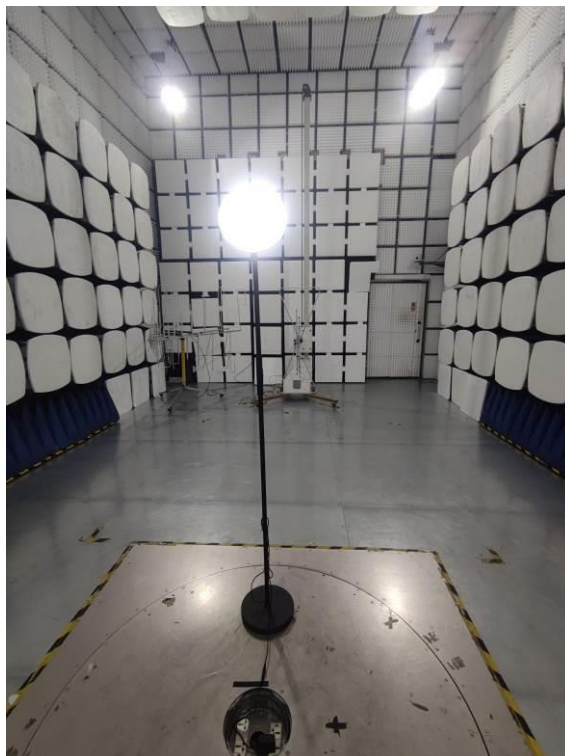
Below 1 GHz
