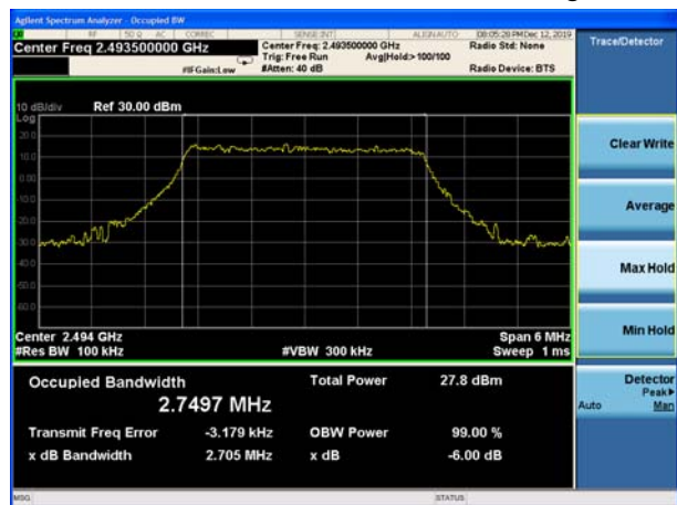
LTE Band 53 3MHz 64QAM CH-High
