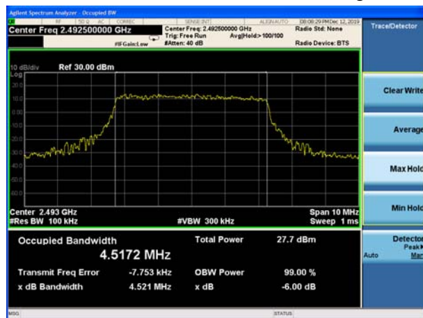
LTE Band 53 5MHz 64QAM CH-High
