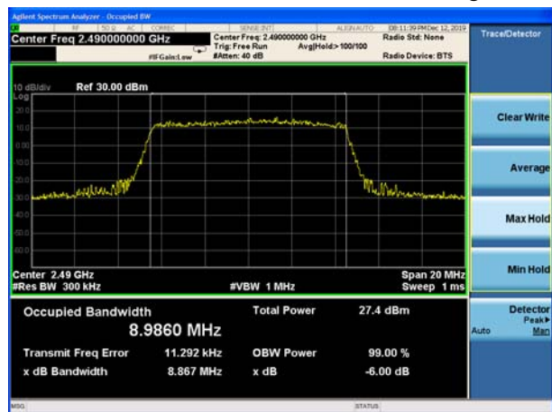
LTE Band 53 10MHz 64QAM CH-High
