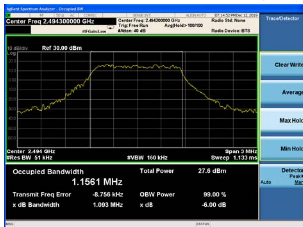
LTE Band 53 1.4MHz 64QAM CH-High
