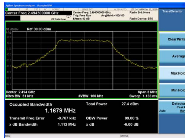
LTE Band 53 1.4MHz QPSK CH-High
