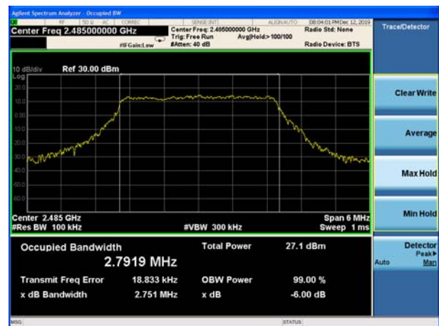
LTE Band 53 3MHz QPSK CH-Middle
