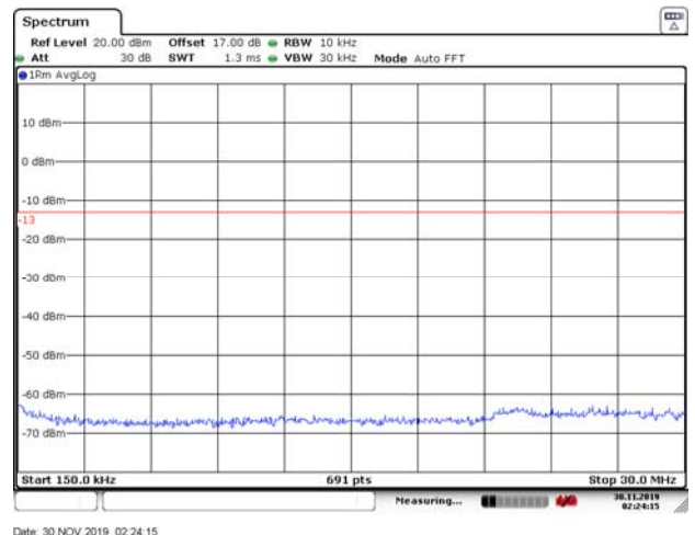
LTE Band 53 1.4MHz CH-Middle 150kHz~30MHz
