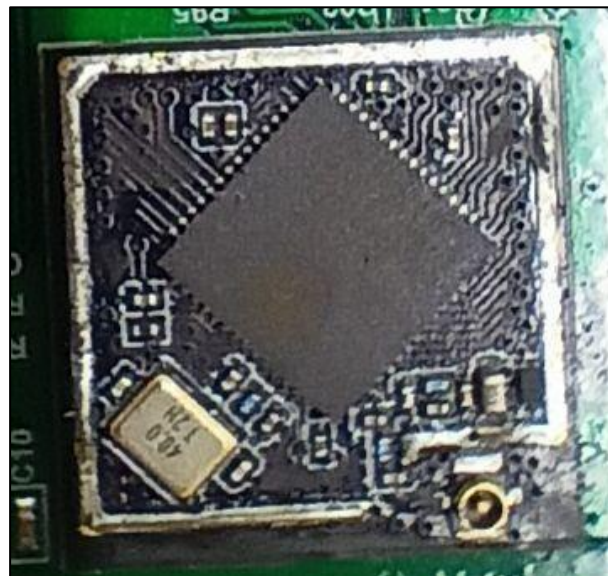
Wi-Fi Module Without Shield
