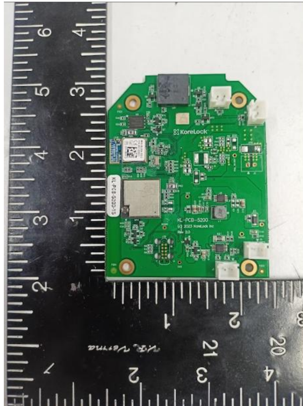
PCB front View with Dimension
