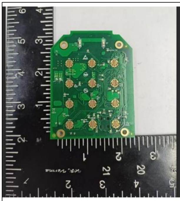
PCB_Rear View with Dimension
