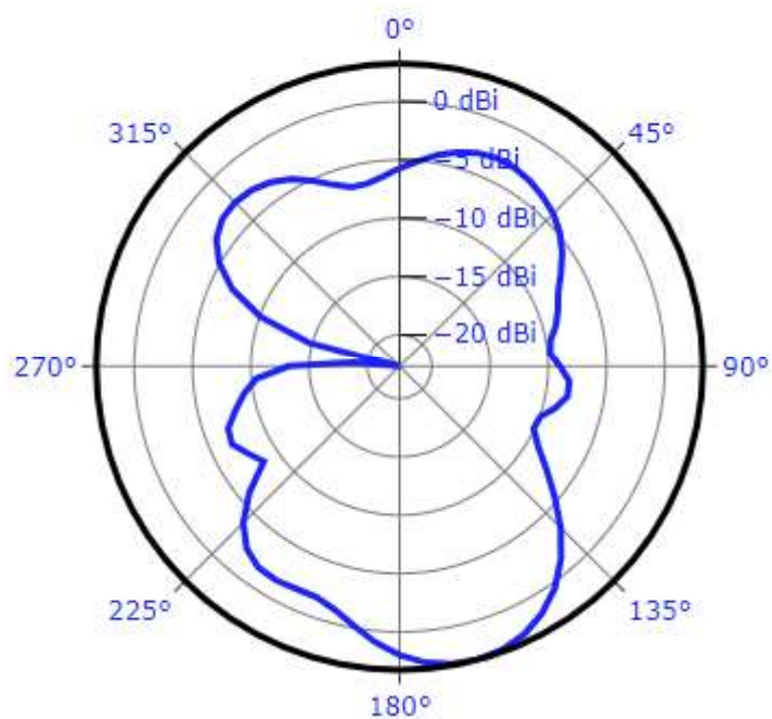
Polar radiation pattern at \phi = 216^\circ
