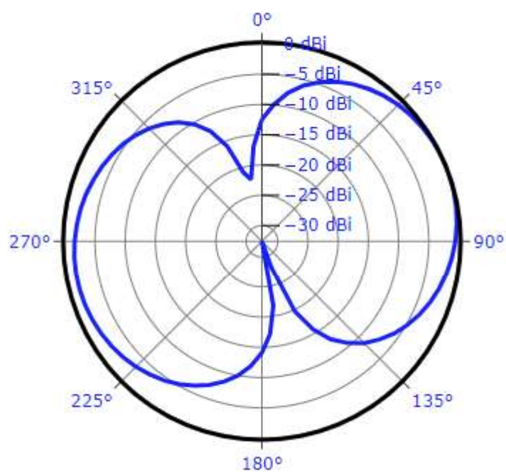
Polar radiation pattern at \phi = 106^\circ
