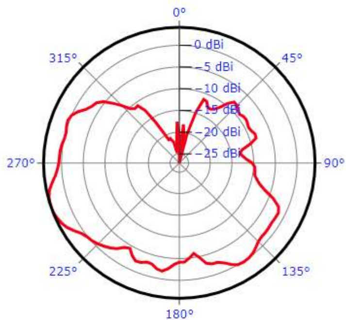
Polar radiation pattern at \theta = 67^\circ
