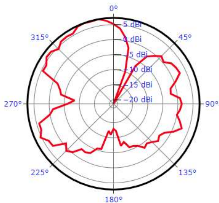
Polar radiation pattern at \theta = 129^\circ
