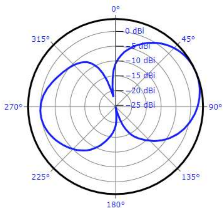
Polar radiation pattern at \phi = 250^\circ
