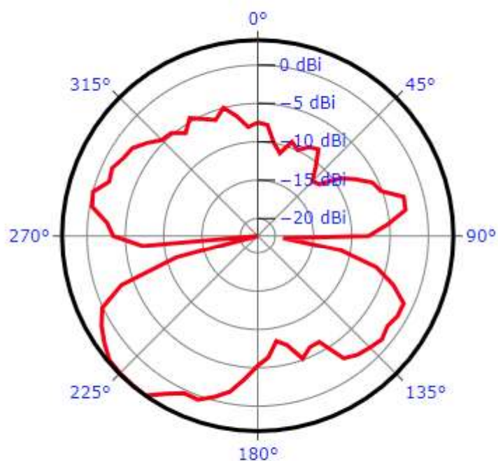
Polar radiation pattern at \theta = 165^\circ
