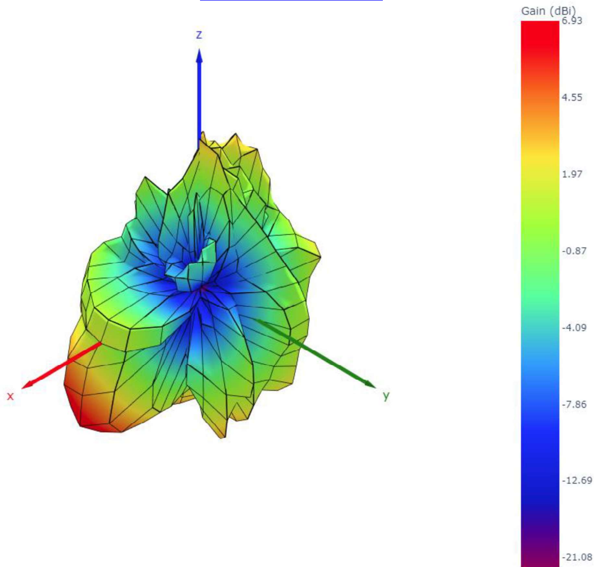
UWB1-6.5GHz-Horizontal-3D
