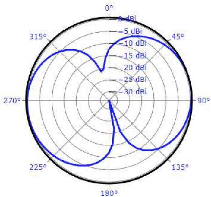
Polar radiation pattern at \phi = 92^\circ
