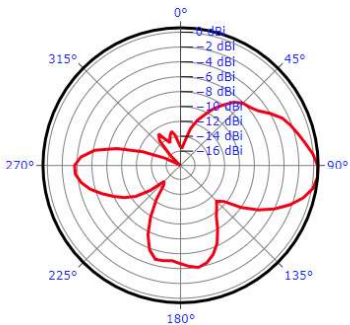
Polar radiation pattern at \theta = 76^\circ
