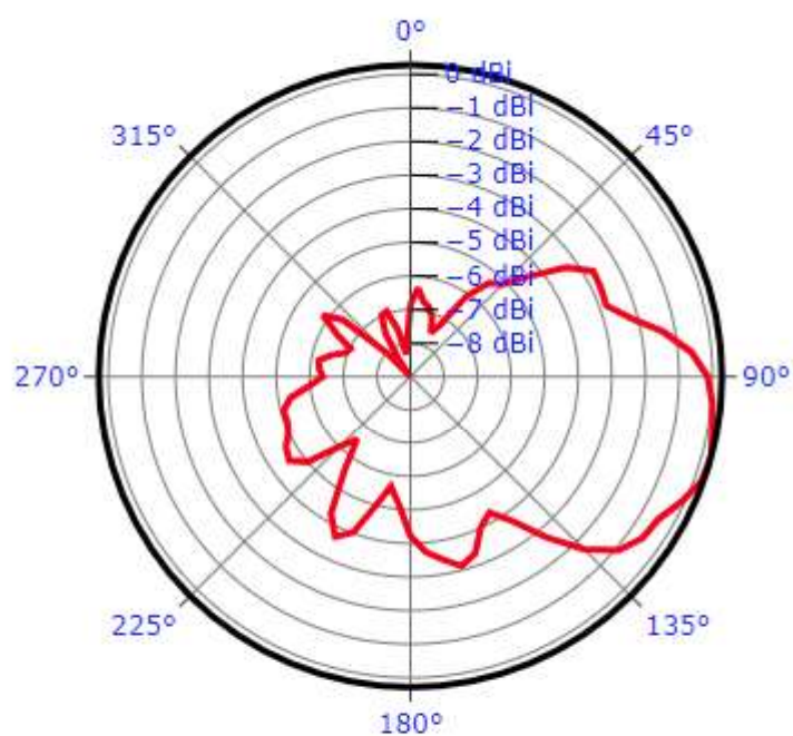
Polar radiation pattern at \theta = 69^\circ
