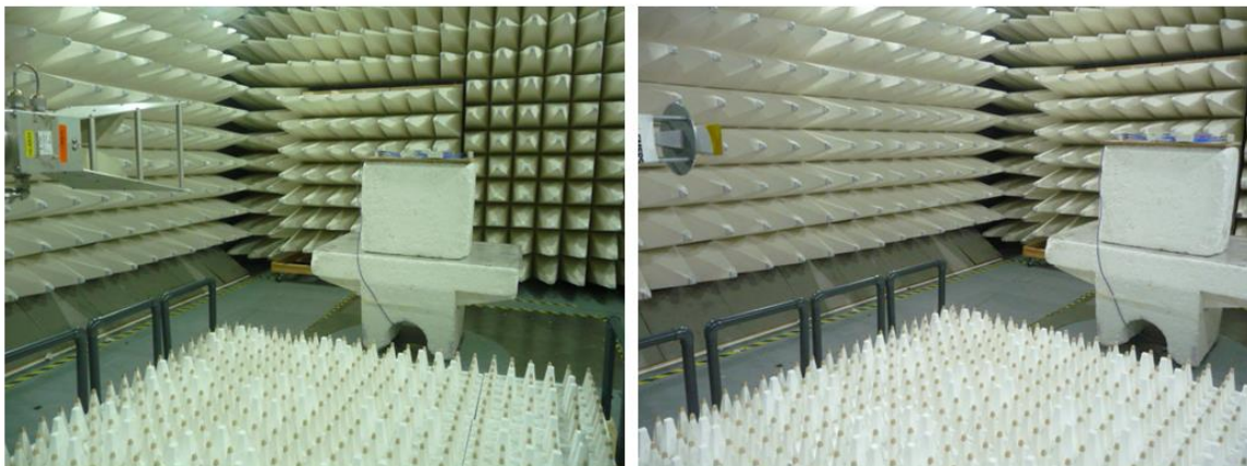
Photograph No.4 Spurious emissions measurement setup in the anechoic chamber in 1000 - 4000 MHz
