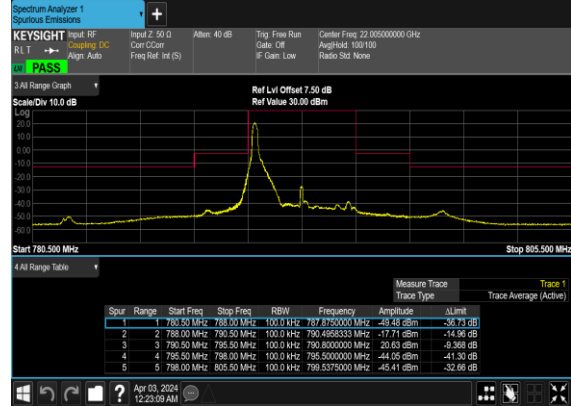
N14(5M)_DFT-s- OFDM_QPSK_Edge_1RB_Left_Mid_CH
