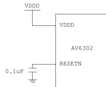
Reset Diagram
