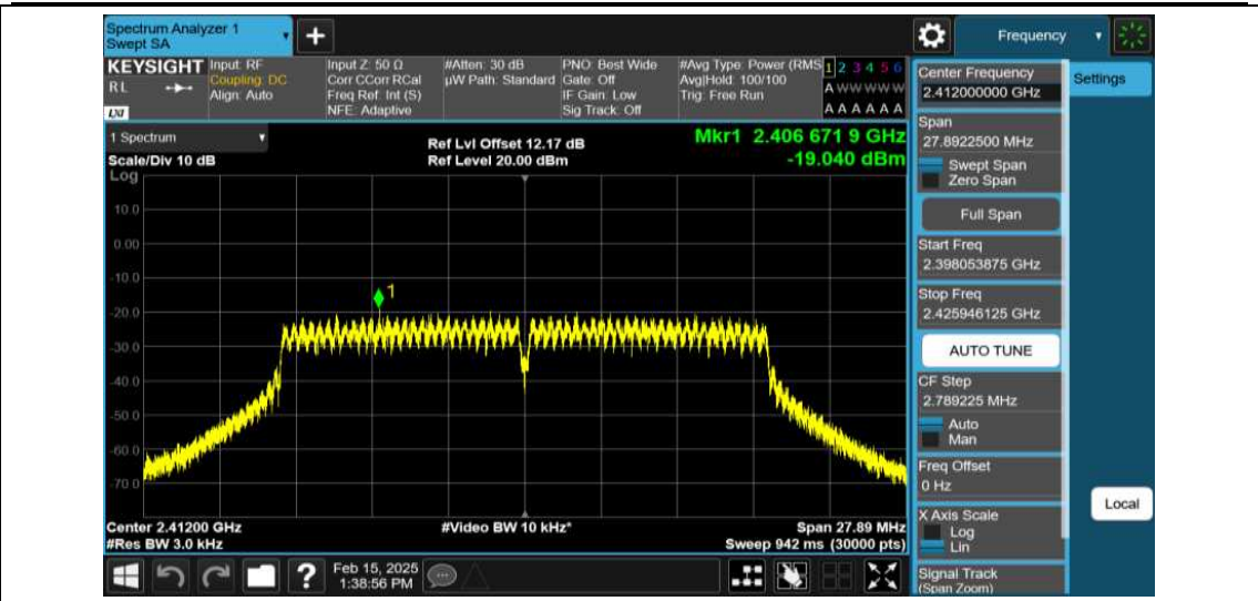
11N20SISO-Ant1-2412-PASS
