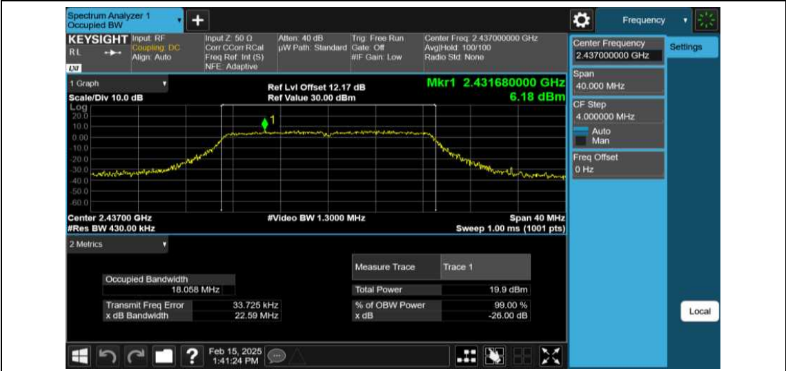
11N20SISO-Ant1-2437
