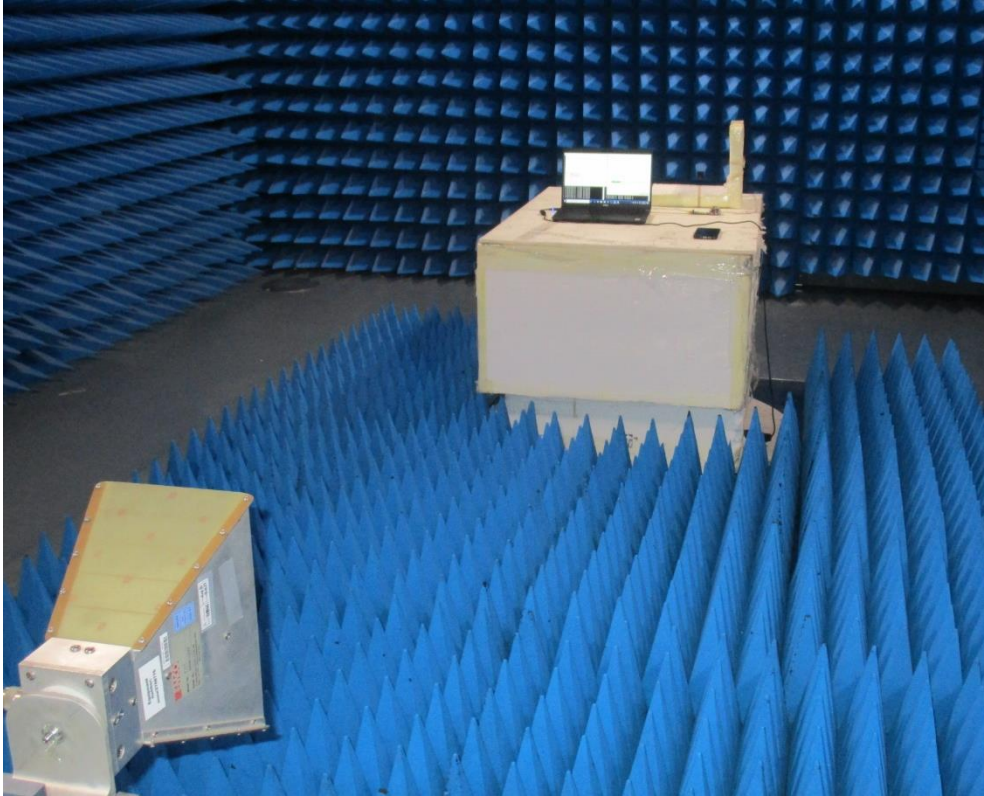
Photo 2 Photograph radiated emissions 1 – 18 GHz
