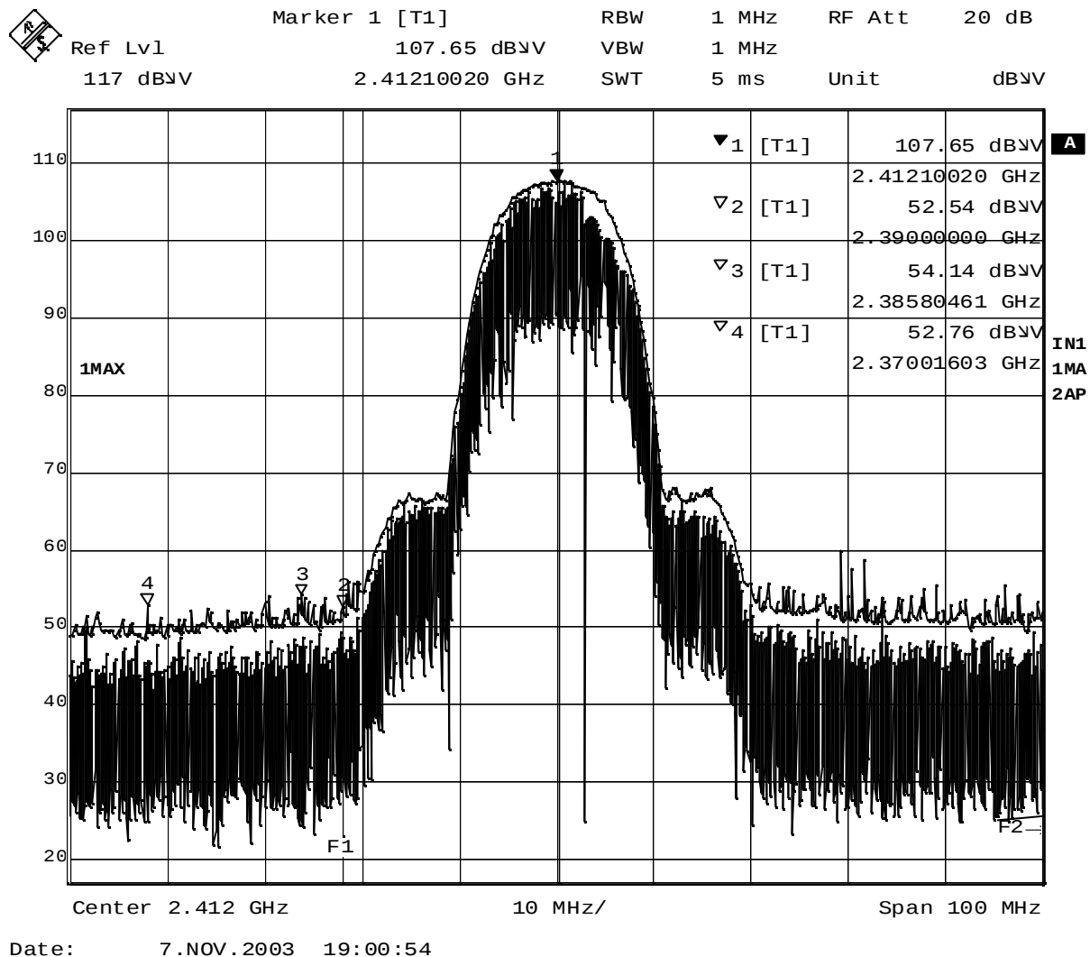
Plot 8-1 Ch.1 2412MHz TX, DSSS 11Mbps (Peak)
