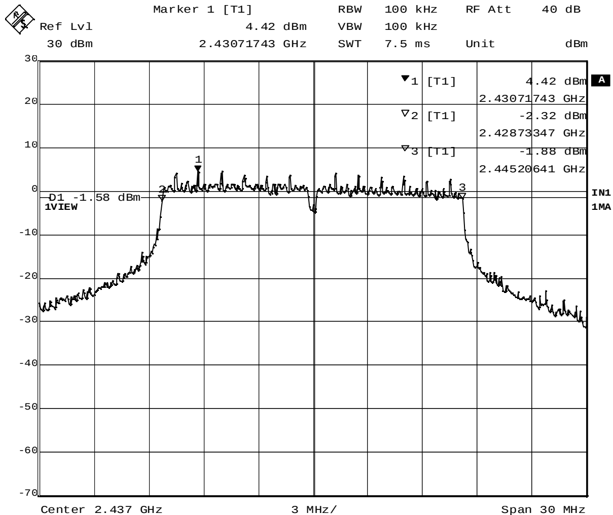
Plot 1-4. 6dB BW at 2437MHz (OFDM, 18Mbps)
