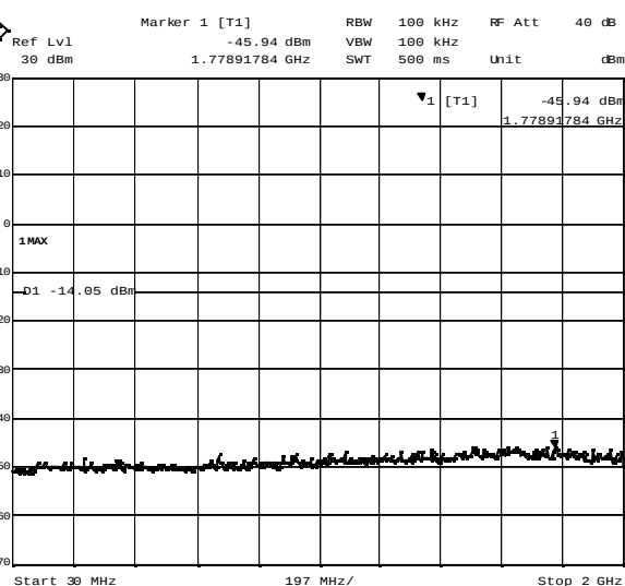
Plot 4-2. Out of band emissions around 2437MHz (DSSS, 11Mbps)
