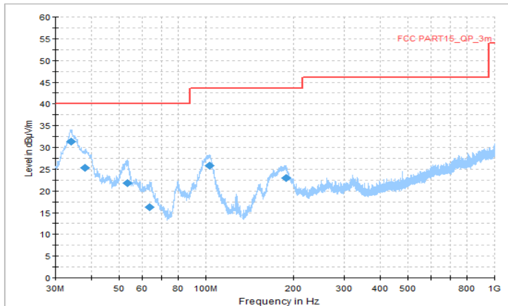
Figure A.10.1.25.Radiated Emission (Camera, 30MHz to 1GHz)
