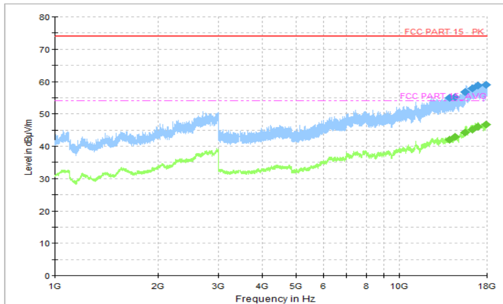
Figure A.10.1.29. Radiated Emission (Camera, 1GHz to 18GHz)
