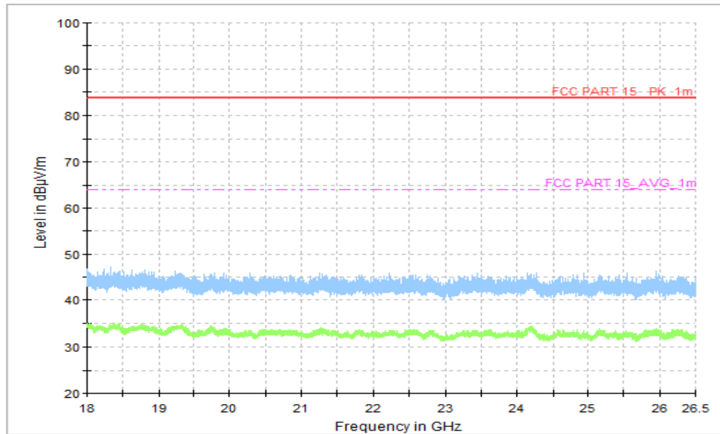
Figure A.10.1.24.Radiated Emission (Video Player,18GHz to 26.5GHz)
