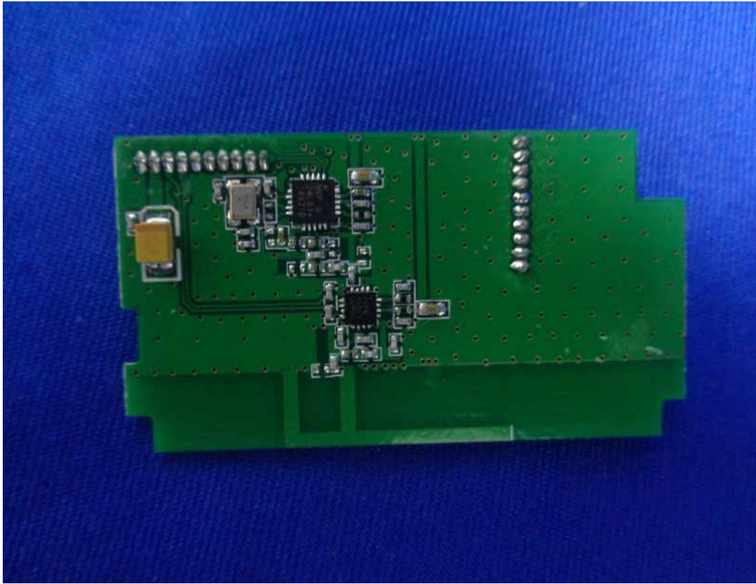
Figure 16 Inside of the EUT
