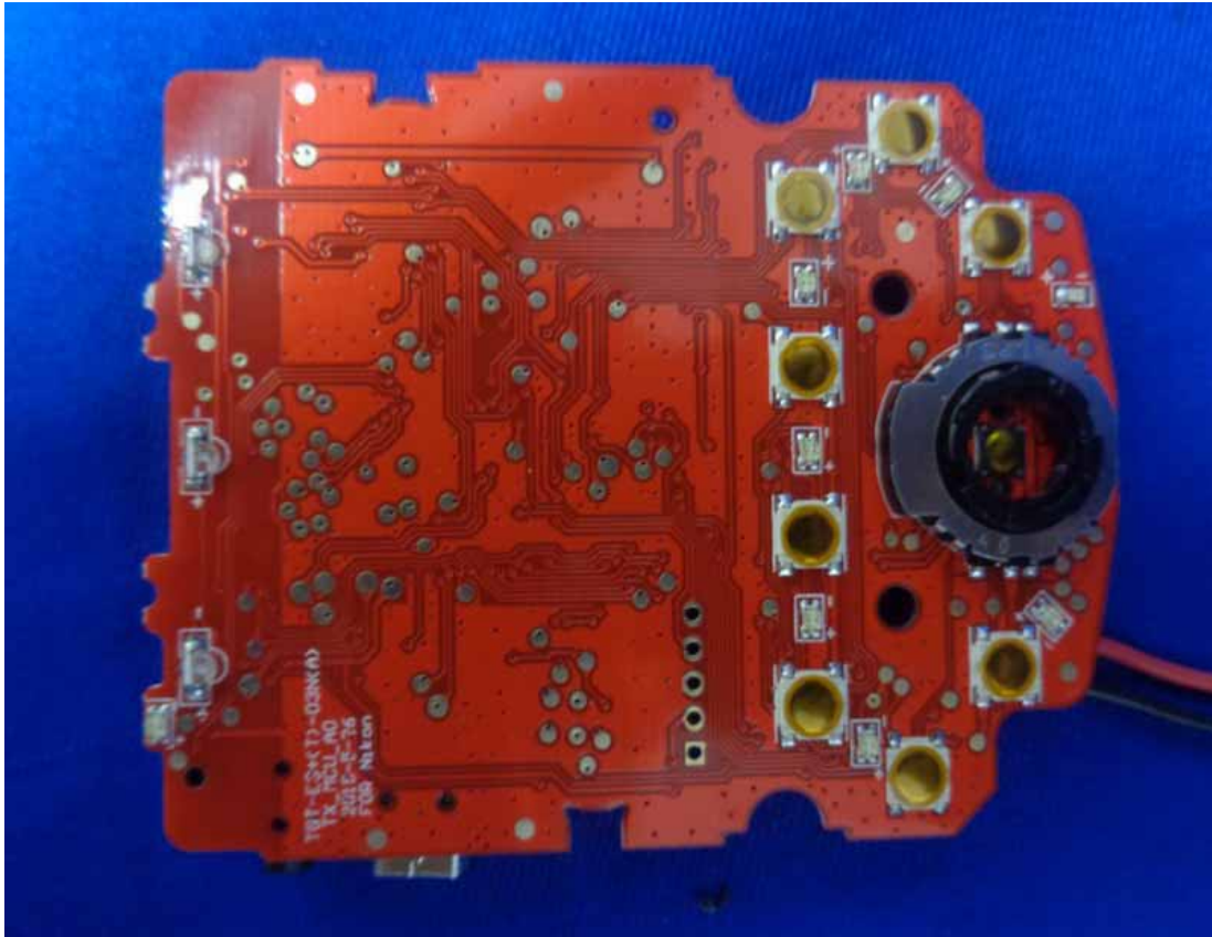
Figure 17 Inside of the EUT
