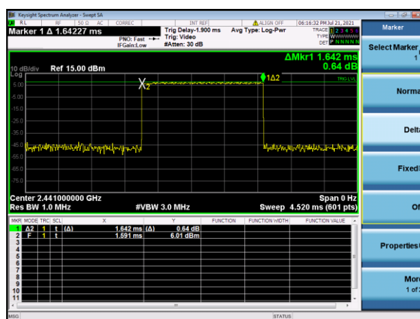
8-DPSK DH3
