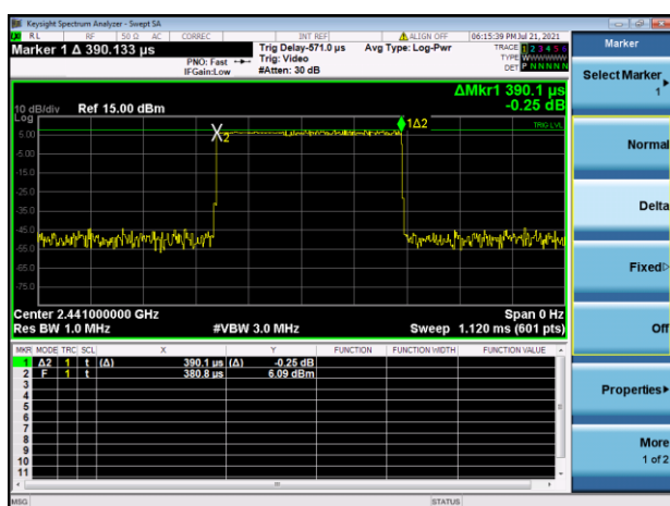
8-DPSK DH1
