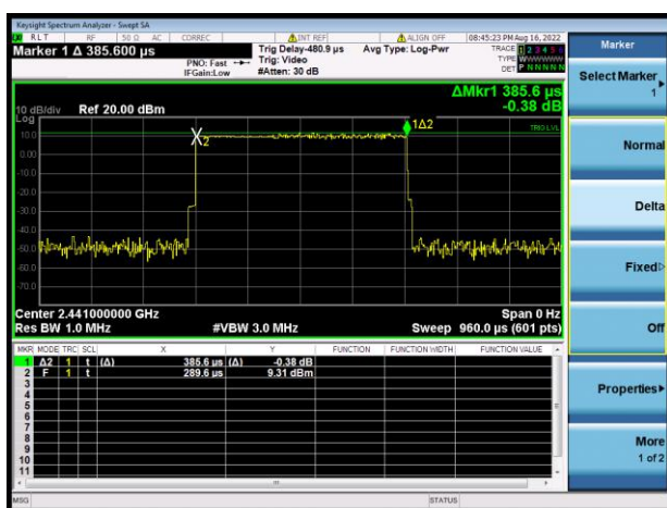
8-DPSK 3DH-1
