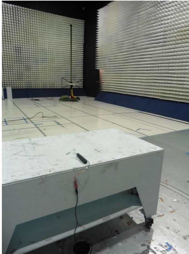
Test Setup Photo 15.247
