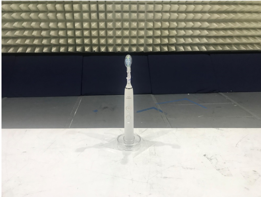
Test Setup Photo - FCC Part 15, Subpart B
