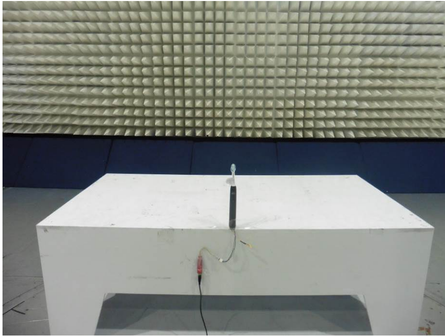
Test Setup Photo 15.225
