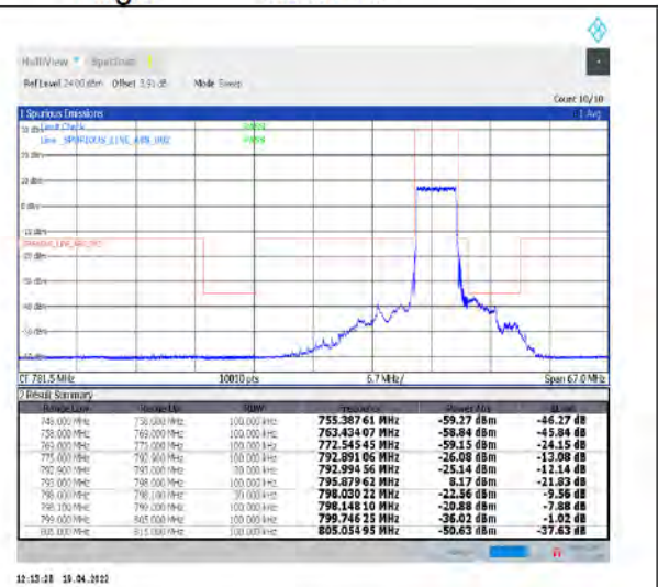
1-N14--15-5-H-3-DFT-PI2BPSK-Outer_Full-25@0-Ant1-PASS-see graph
