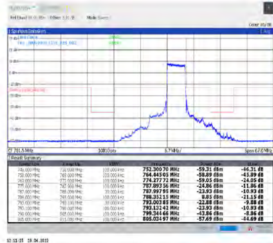
1-N14--15-5-L-3-DFT-PI2BPSK-Outer_Full-25@0-Ant1-PASS-see graph
