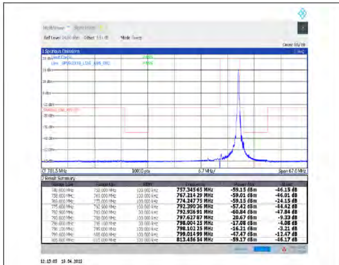
1-N14--15-5-H-2-DFT-PI2BPSK-Edge_1RB_Right-1@24-Ant1-PASS-see graph
