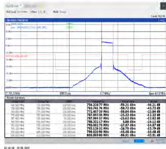
1-N14--15-5-L-6-CP-QPSK-Outer_Full-25@0-Ant1-PASS-see graph
