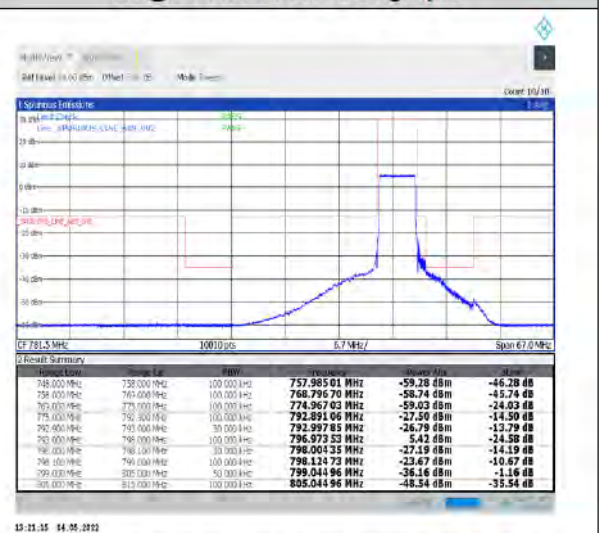
1-N14--15-5-H-6-CP-QPSK-Outer_Full-25@0-Ant1-PASS-see graph
