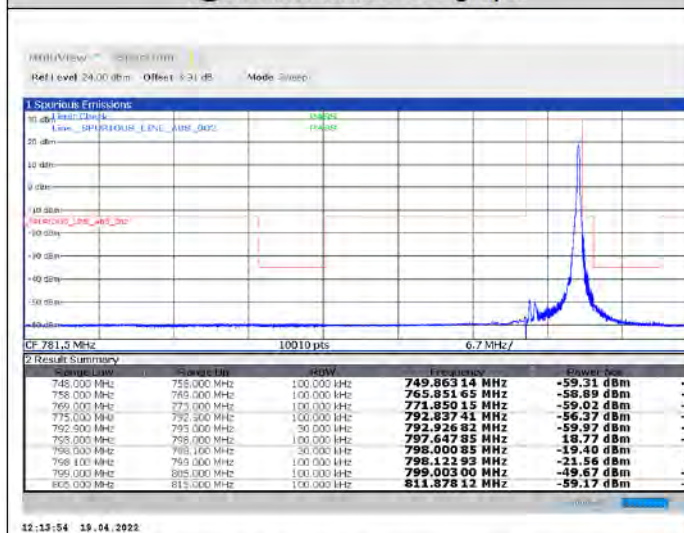
1-N14--15-5-H-5-CP-QPSK-Edge_1RB_Right-1@24-Ant1-PASS-see graph
