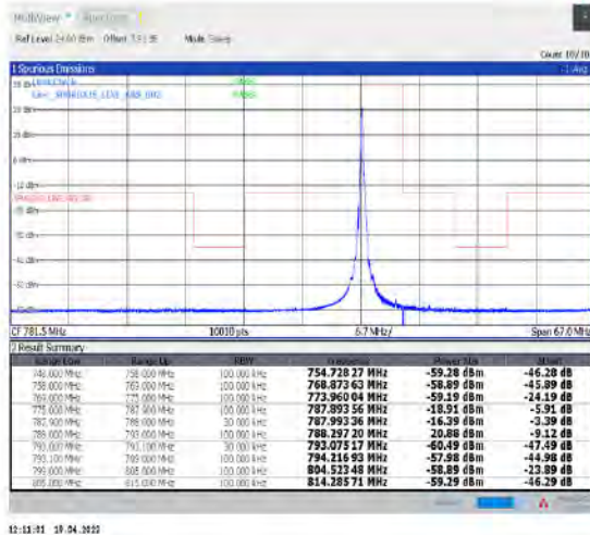
1-N14--15-5-L-1-DFT-PI2BPSK-Edge_1RB_Left-1@0-Ant1-PASS-see graph
