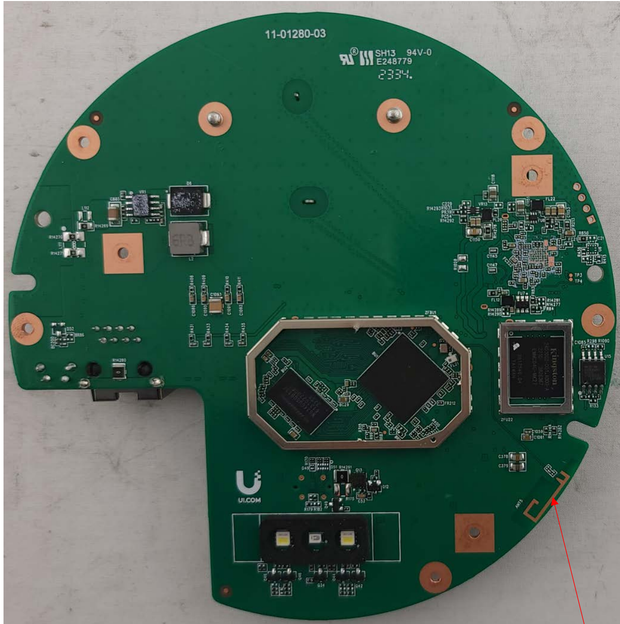
Photograph 4: Internal View of Main PCB Bottom
