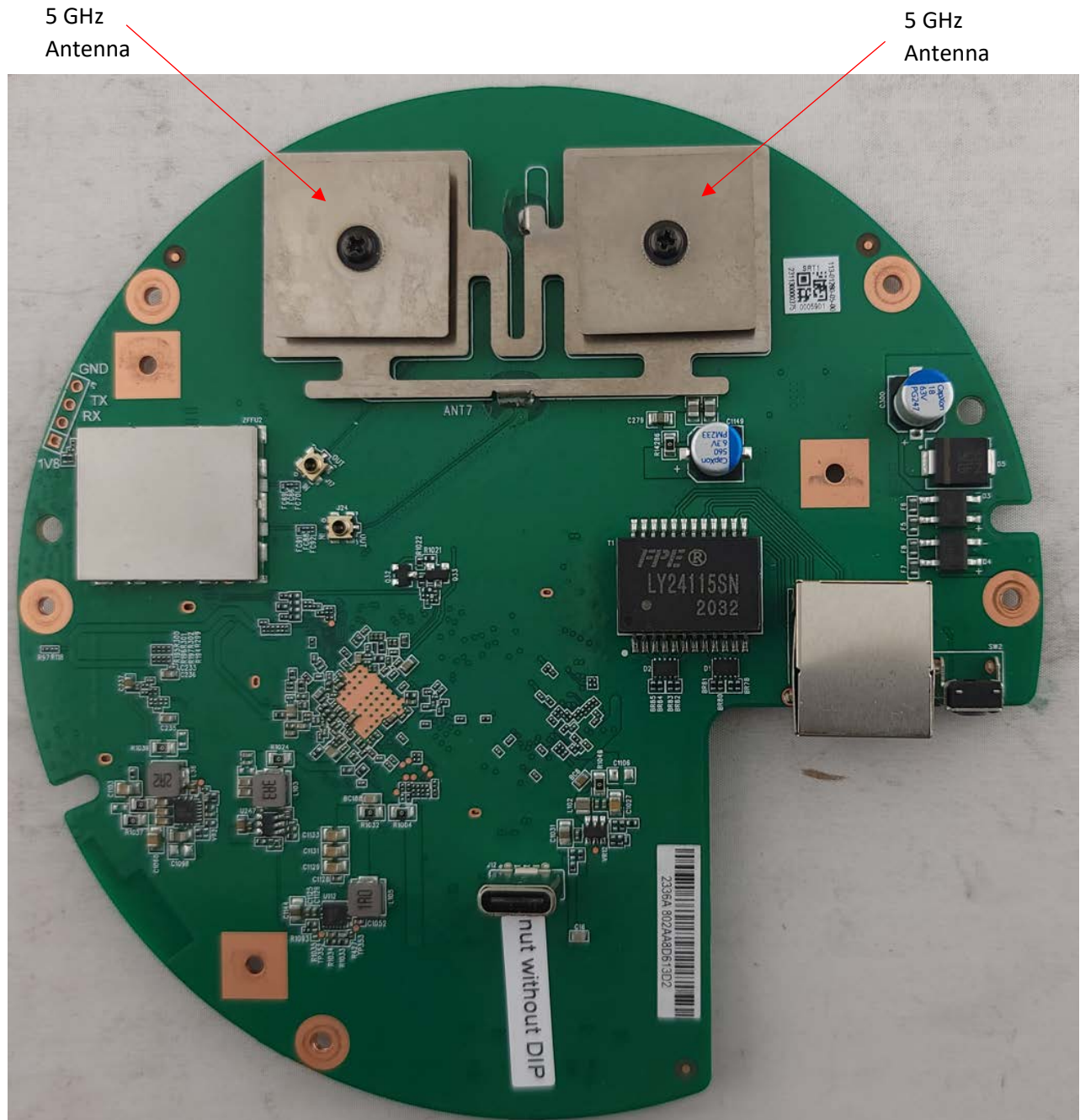
Photograph 2: Internal View of Main PCB Top
