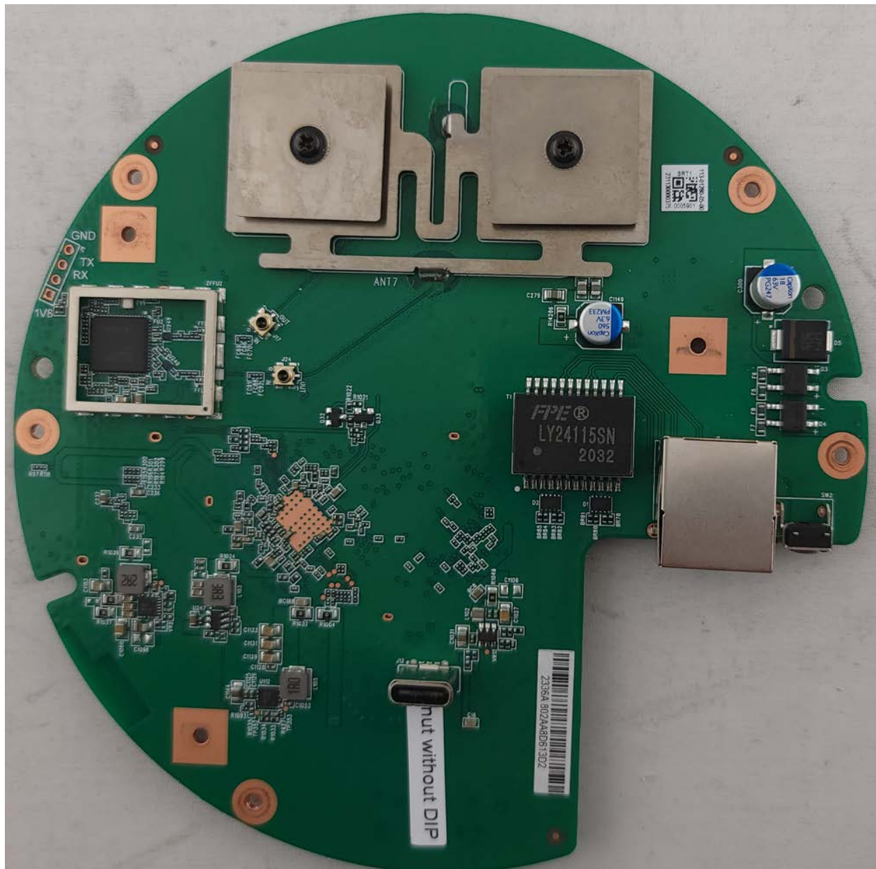
Photograph 3: Internal View of Main PCB Top with Cans Off
