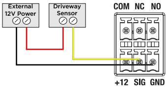
Wire the contact to an externally powered sensor (Driveway sensor)
