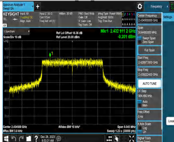
5M_Ant1_2434.5
