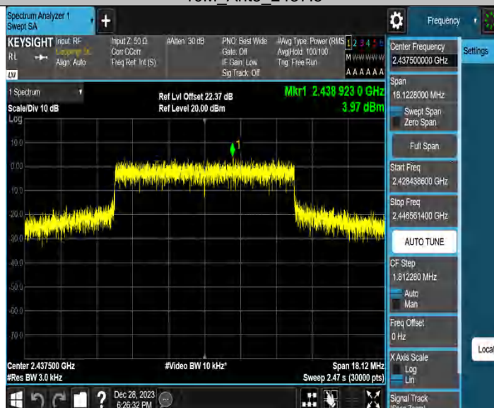
10M_Ant3_2437.5
