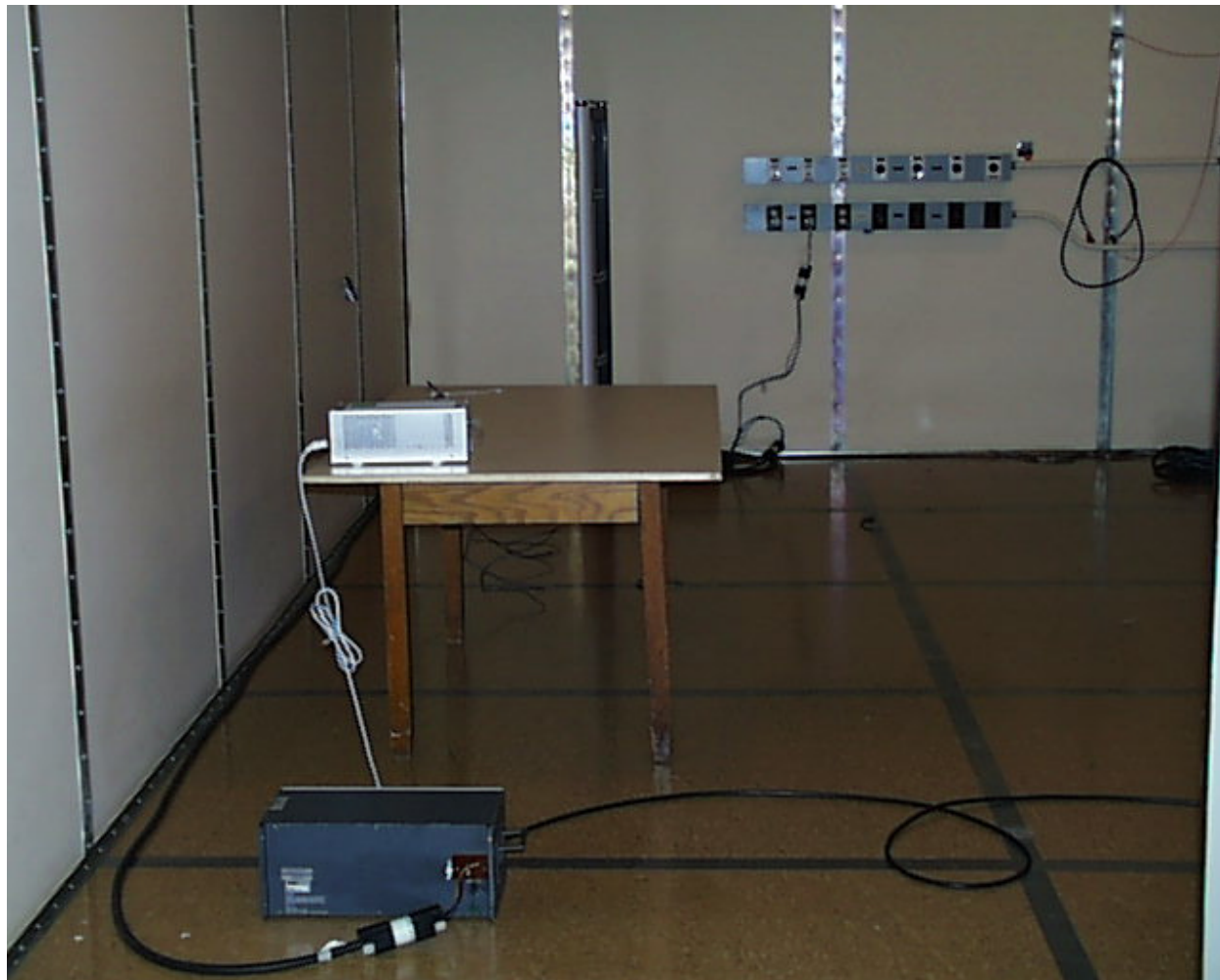
Photo 7 – Strata PX w/TR4024/22 Control Board Conducted Emissions Test Setup
