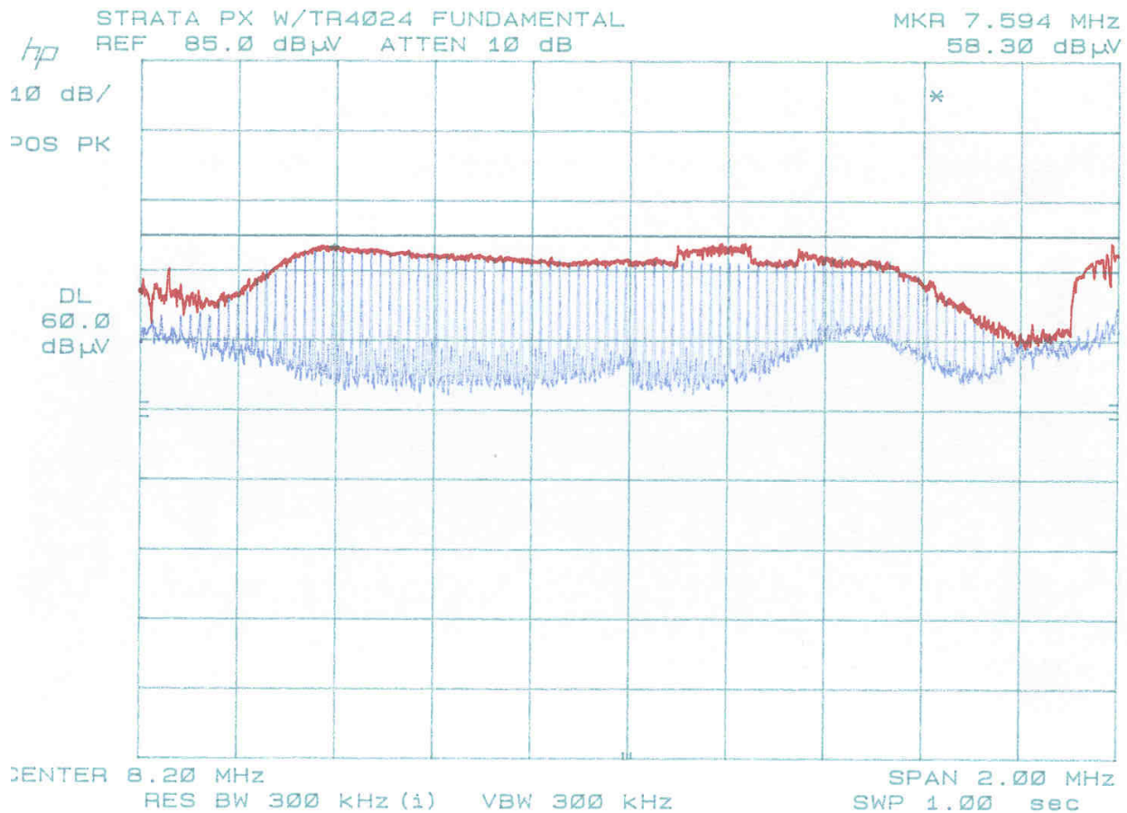
Photo 6 – Bandwidth Plot
