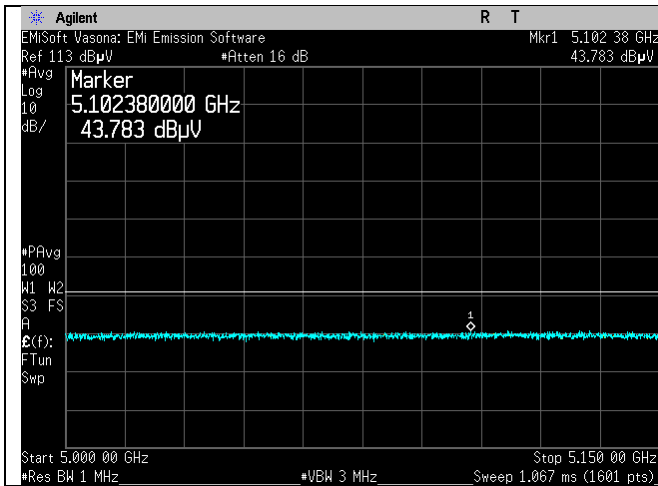
5180_amode_avg
